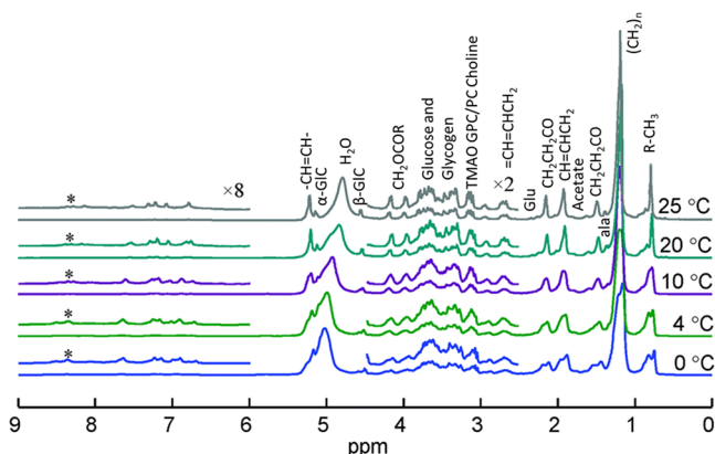
Figure 6. Stacked plot of the variable-temperature ^1\text{H} MAS NMR spectrum of 280 mg of mouse liver from 0 to 25 ^\circ\text{C} . Adapted with permission from ref 16. Copyright 2015 Royal Society of Chemistry.
