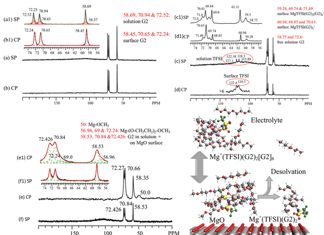
Figure 7. (a) ^{13}\text{C} SP/MAS (a) and CP/MAS (b) spectra obtained on \text{MgO}_{550} (clean surface) + 0.1 M \text{Mg}(\text{TFSI})_2 in G2 after in situ heat treatment at 180 ^\circ\text{C} for 1 h. Traces a1 and b1 are horizontally expanded regions (55 to 75 ppm) of traces a and b, highlighting \text{MgO} surface-adsorbed G2 with peaks located at approximately 58.4, 70.65, and 72.23 ppm. No electrolyte decomposition is observed for this sample. (c) ^{13}\text{C} SP/MAS (c) and CP/MAS (d) spectra obtained on \text{MgO} and 1.0 M \text{Mg}(\text{TFSI})_2 in G2 after in situ heat treatment at 180 ^\circ\text{C} for 1 h. Traces c1 and d1 are horizontally expanded regions of traces c and d, highlighting \text{MgO} surface-mediated adsorption products with peaks at approximately 60.94, 68.85, and 70.63 ppm, surface adsorbed G2 with peaks located at approximately 59.28, 69.74, and 71.49 ppm, and surface adsorbed \text{TFSI}^- at 118.3 and 122.4 ppm. No electrolyte decomposition is observed for this sample. (e) ^{13}\text{C} CP/MAS and SP/MAS (f) spectra obtained on \text{MgO}_{550} + G2 after reacting at 180 ^\circ\text{C} for 1 h. Traces e1 and f1 are horizontally expanded regions of traces e and f. The bottom right schematic depicts the desolvation process. Reprinted with permission from ref 45. Copyright 2019 American Chemical Society.
