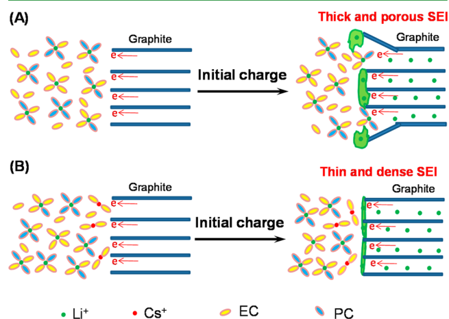
Figure 5. Schematic mechanism of SEI film formation promoted by \text{Cs}^+ . (A) In a conventional electrolyte, \text{Li}^+ favors PC to form solvates. (B) In a \text{Cs}^+ -containing electrolyte, due to the preferential formation of \text{Li}^+(\text{PC})_n solvates, \text{Cs}^+ coordinates with EC molecules, and its solvates have priority to be electrochemically reduced.
