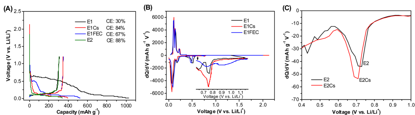
Figure 1. Electrochemical behavior of various \text{LiPF}_6\text{-CsPF}_6 electrolytes on graphite surfaces. (A) Lithiation/delithiation profiles of Lilgraphite half cells using electrolytes of E1, E1Cs, E1FEC, and conventional E2. (B and C) Comparison of differential capacity ( dQ/dV ) plots of Lilgraphite cells using electrolytes of E1, E1Cs, and E1FEC (B), and E2 and E2Cs for the 0.75 V peak (C).
