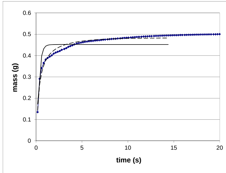
Figure 2. Mass uptake data (♦) for a capillary rise experiment with ethylene glycol in a 3-layer wick made of 4A17-050F Delker expanded metal screens. Least squares curve fit (—) of the data to the single-mode capillary rise equation and to the dual-mode capillary rise equation (- -).
