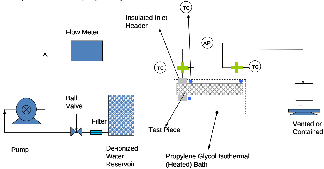
Figure 3. Schematic of phase change heat transfer experimental set-up.
