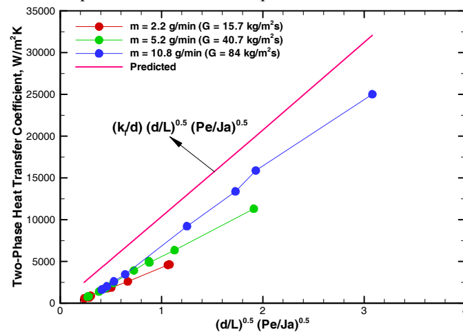
Figure 5. Two-phase heat transfer coefficient as a function of modified Peclet number.
