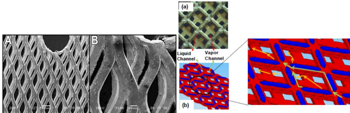
Figure 1. Examples of dual-mode wicks, including a 2-layer Dexmet expanded metal foil wick (A and B) and a second constructed of photo chemically machined (PCM) layers (a) with a schematic showing flow paths (b).
