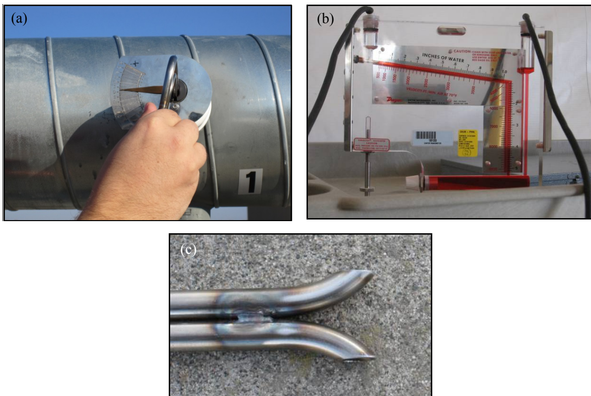
Figure 3.3. Equipment Used for the Flow Angle Test: (a) S-type Pitot Tube Inserted in a Test Port with the Angle-Indicating Device, (b) Slant-Tube Manometer, and (c) Openings at Tip of S-Type Pitot Tube
