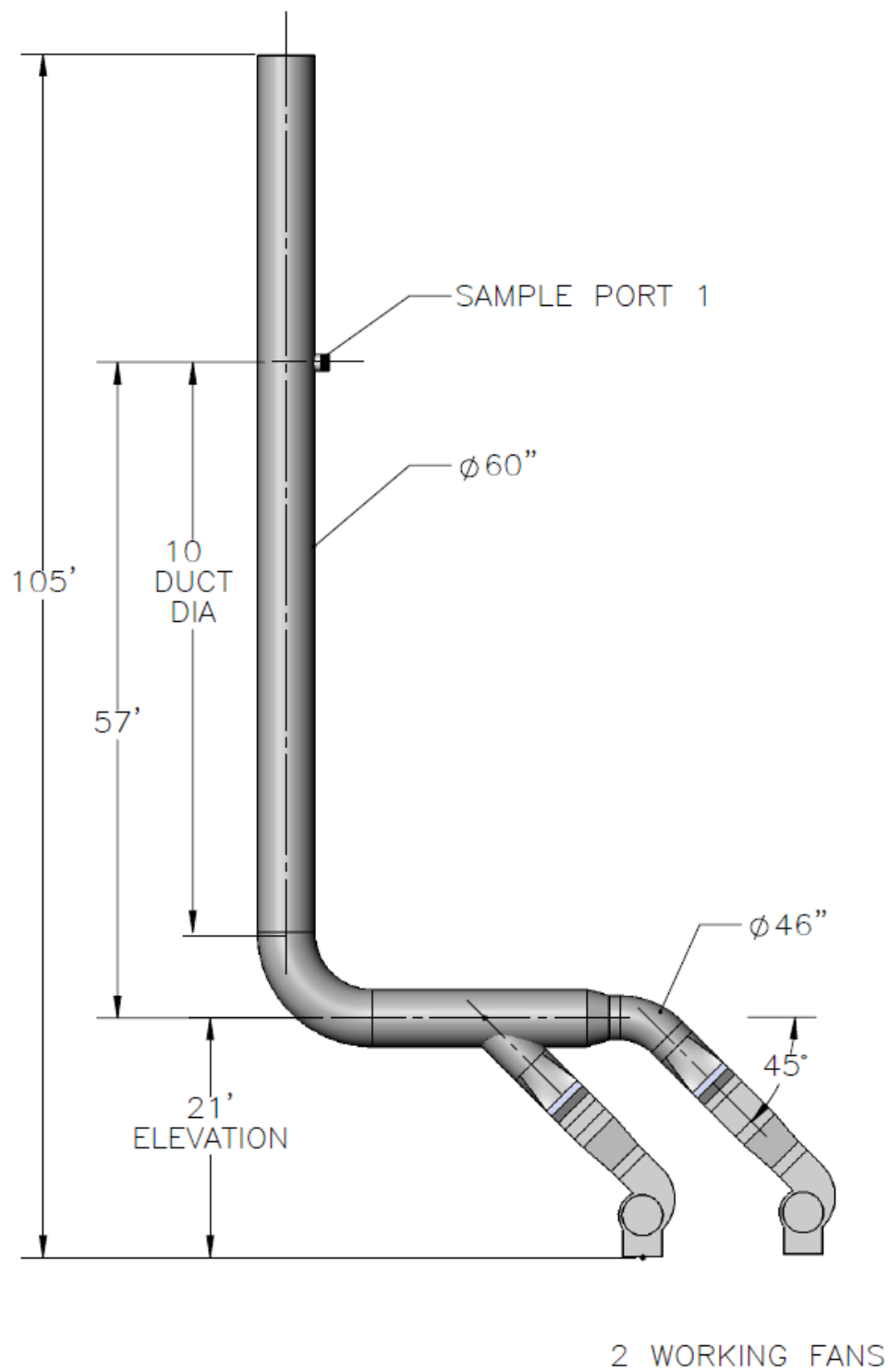
Figure 2.1. LAW C2V (LV-C2) System Per Design
