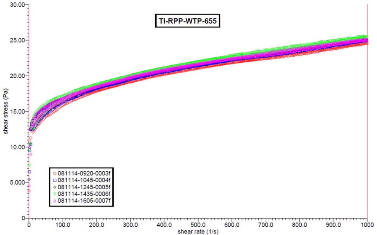
Figure D.6. Rheograms for All Samples Taken During TI-RPP-WTP-655
