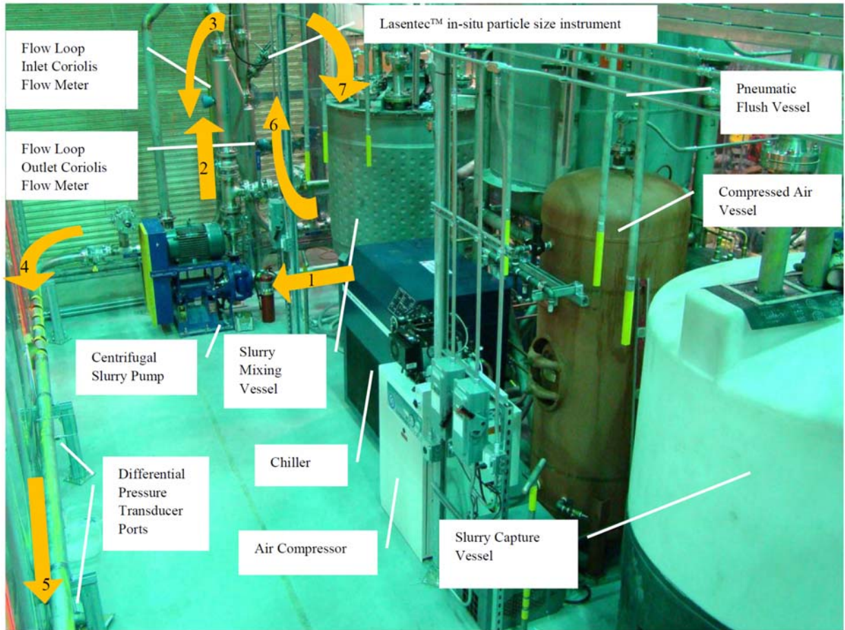
Figure 4.1. Photograph of Flow Loop System with Major Equipment Identified; Arrows and Numbers Indicate Flow Direction in Normal Operation
