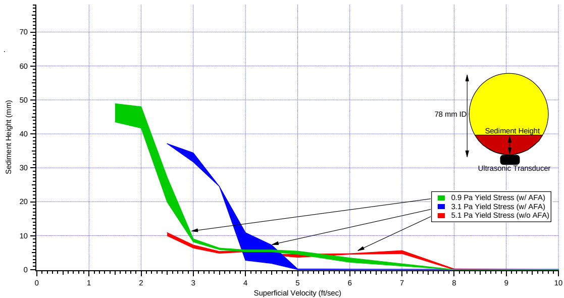
Figure 7.3. Thickness of Stationary Bed of Particles in Pipeline With Simulant of AZ-101 HLW Pretreated Sludge at Different Yield Stresses As Measured by Ultrasonic Pulse-Echo Technique; These data are considered “For Information Only.”
