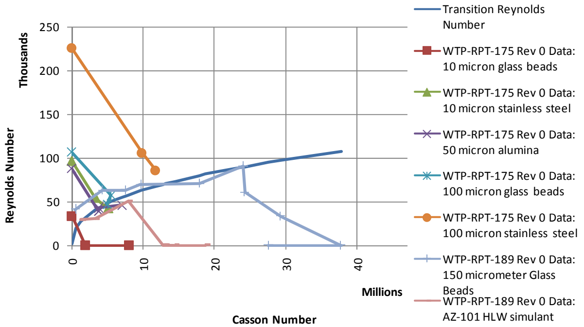
Figure 7.4. Plot of Reynolds Number at Deposition for all Experimental Data from the M-1 Project; Reynolds Number at the Laminar to Turbulent Transition is also Plotted.
