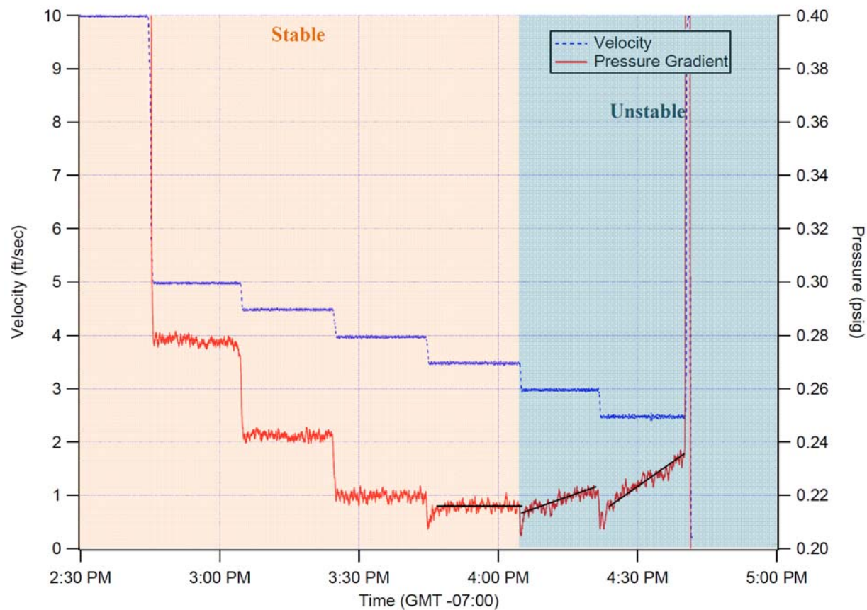
Figure A.8. Pressure-Gradient Data for Casson-Fluid Yield Stress of Approximately 2.6 Pa and Infinite-Shear Viscosity of 1.6 cP. This test was conducted on 11/21/08. The pressure signal is stable until 3.0 ft/sec where an increase in pressure with time is observed. This slurry is considered to be unstable in a 3" pipe below 3.5 ft/sec.
