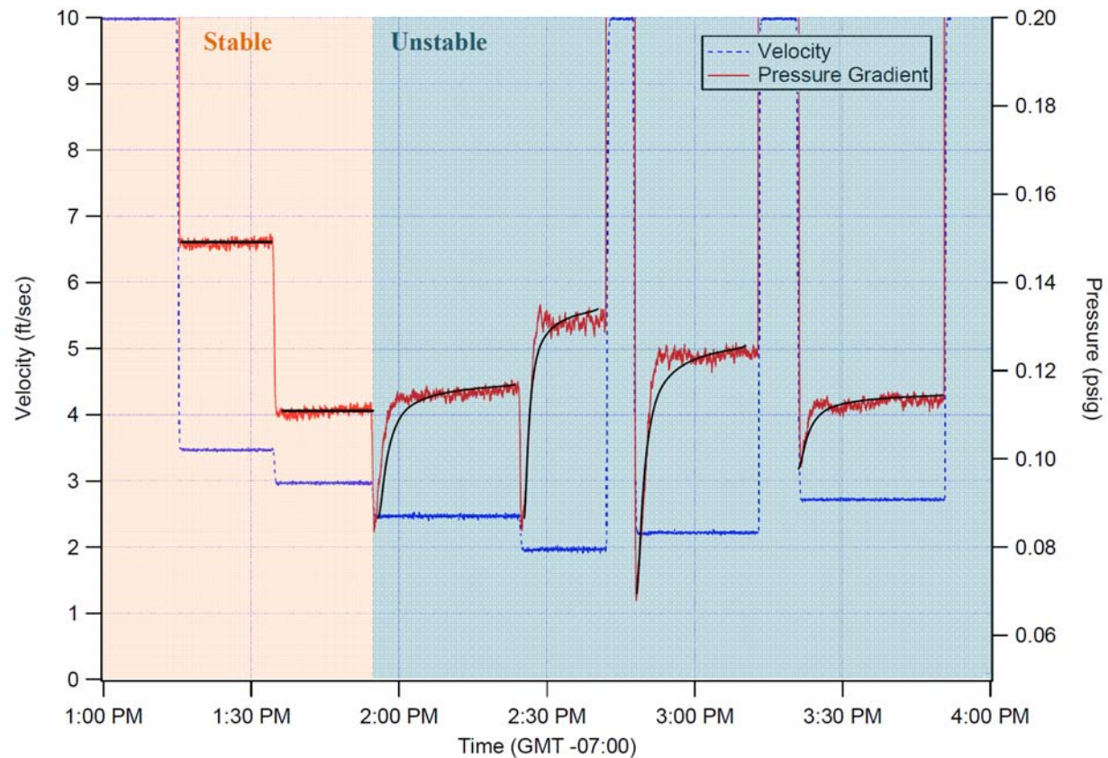
Figure A.10. Pressure-Gradient Data for Casson-Fluid Yield Stress of Approximately 0.3 Pa and Infinite-Shear Viscosity of 2.1 cP. This test was conducted on 11/24/08. The pressure signal is stable until 2.5 ft/sec where an increase in pressure with time is observed. This slurry is considered to be unstable in a 3" pipe below 3.0 ft/sec.
