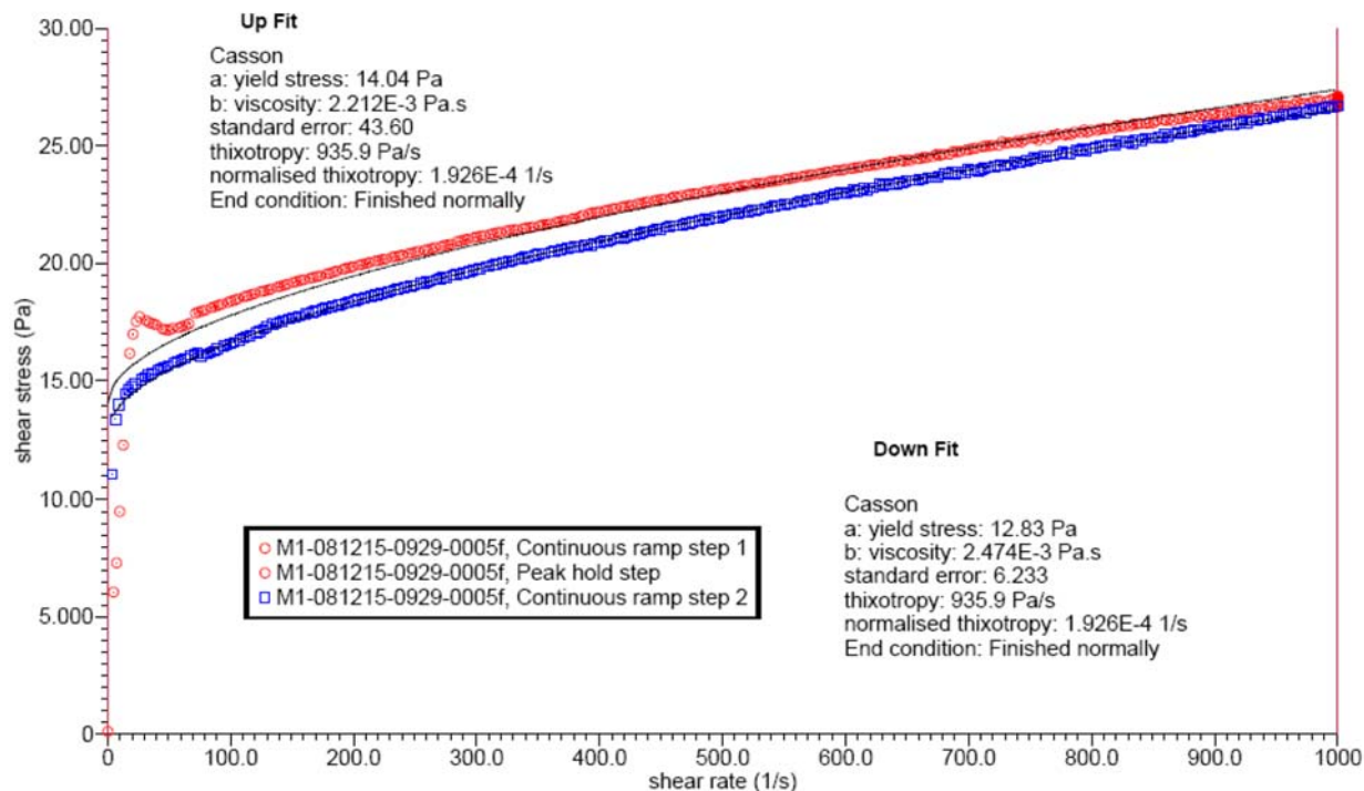
Figure D.25. Rheogram of Physical and Rheological Complex-Simulant Sample for TI-RPP-WTP-664
