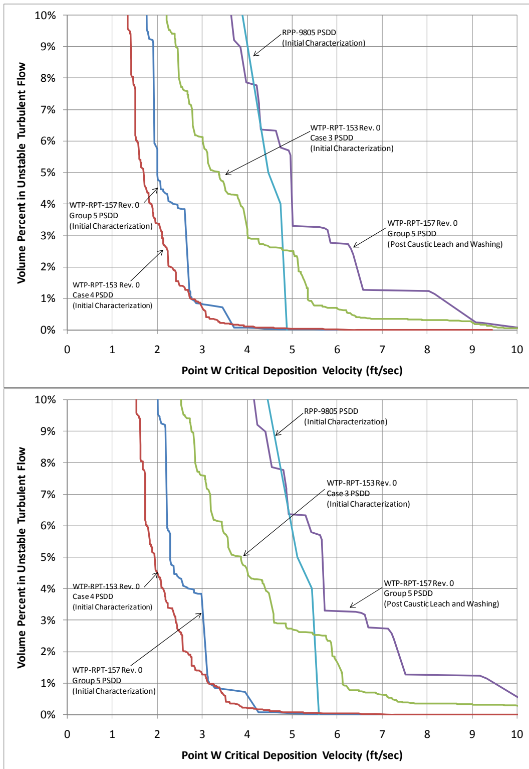
Figure 8.5. Fraction of Slurry Particles in Unstable Turbulent Flow in 3" Pipe (Top) and 4" Pipe (Bottom) at Various Velocities and PSDDs
