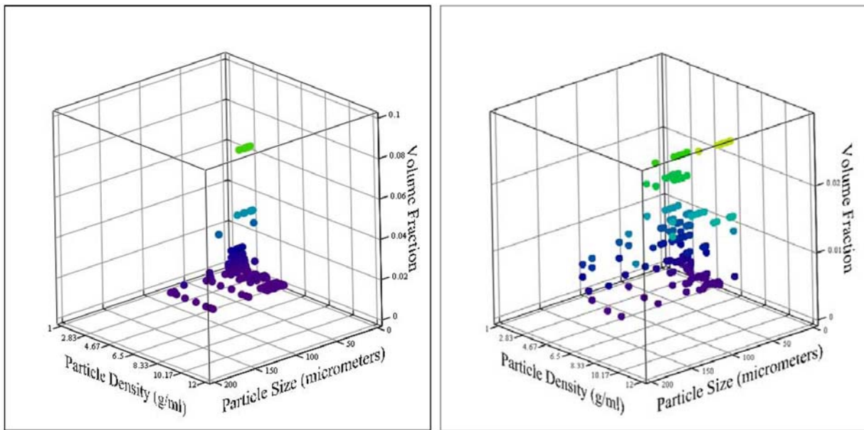
Figure 8.3. M-12 PSDD From Unleached (Left) and Leached (Right) Group 5 Composite With Data From Fiskum et al. (2008; WTP-RPT-157 Rev. 0 )
