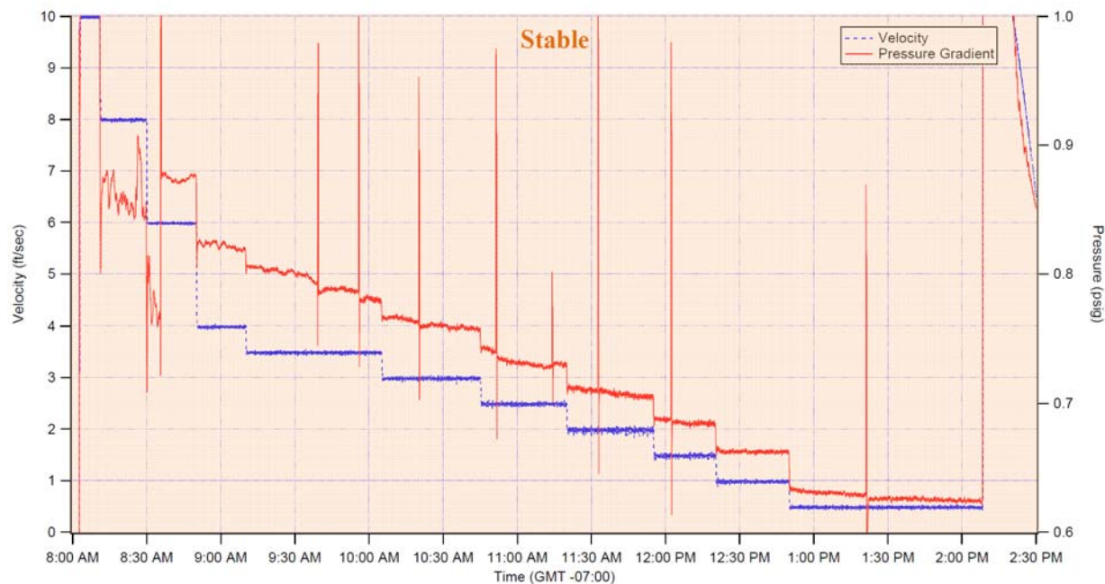
Figure B.3. Pressure-Gradient Data for Casson-Fluid Yield Stress of Approximately 12.8 Pa and Infinite-Shear Viscosity of 2.5 cP. This test was conducted on 12/15/08. Since no dramatic increase in pressure is observed at low velocities this slurry is considered to be stable in a 3" pipe.
