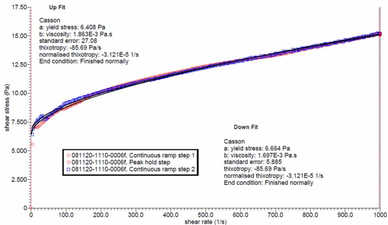
Figure D.11. Rheogram of Physical and Rheological Sample for TI-RPP-WTP-658
