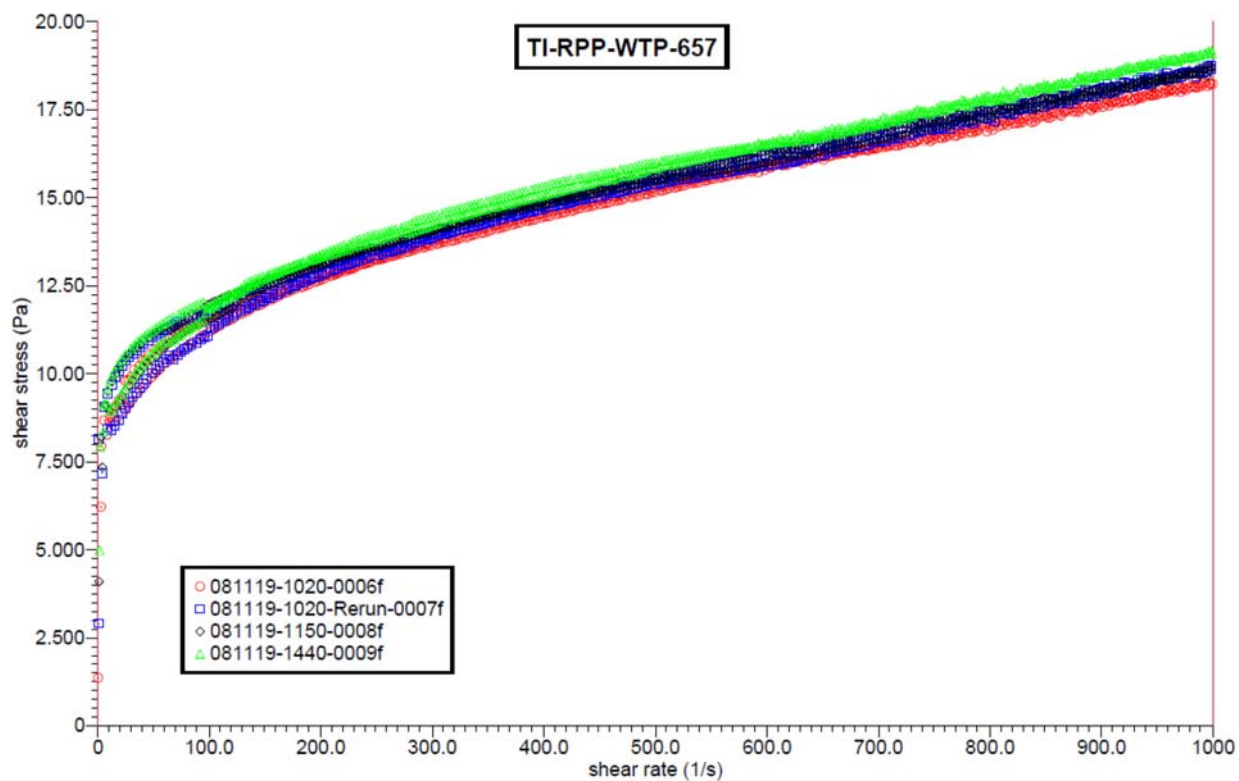
Figure D.10. Rheograms for All Samples Taken During TI-RPP-WTP-657
