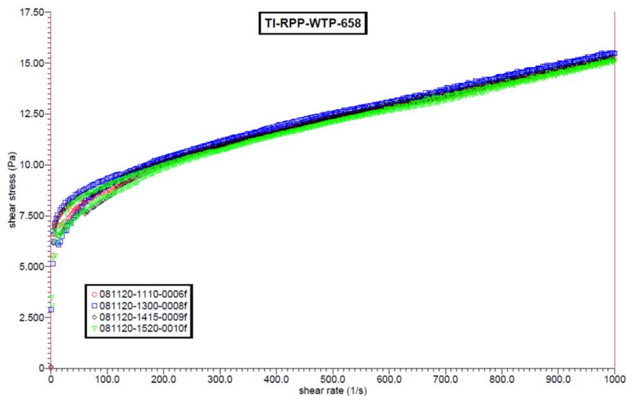
Figure D.12. Rheograms for All Samples Taken During TI-RPP-WTP-658
