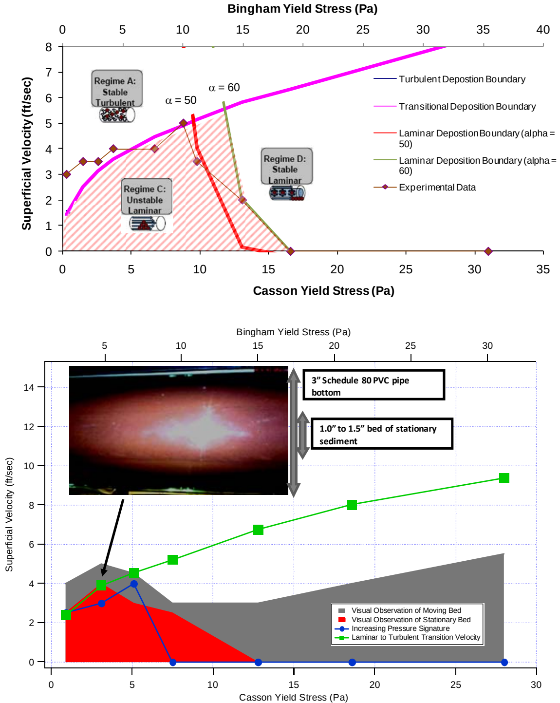
Figure S.1. Deposition Velocity Test Results for 150 \mu m Glass Beads & Kaolin Slurry (Top) and AZ-101 HLW Pretreated Simulant (Bottom)
