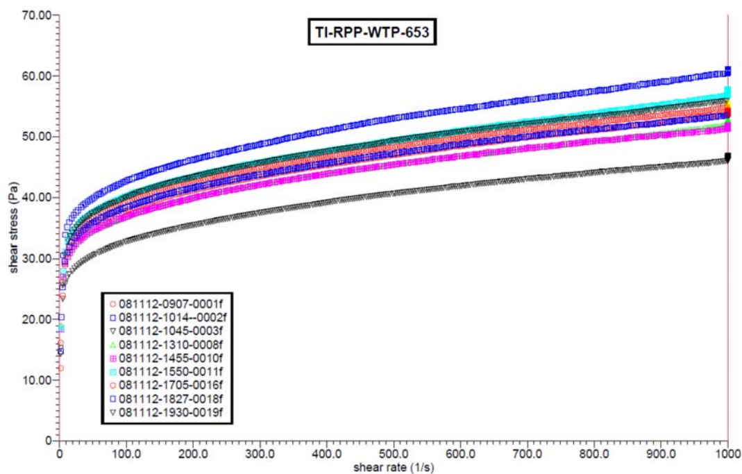
Figure D.2. Rheograms for All Samples Taken During TI-RPP-WTP-653 (Down Curves Only)
