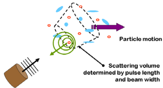
Figure C.4. Concept of Ultrasonic Measurement of Particle Motion
