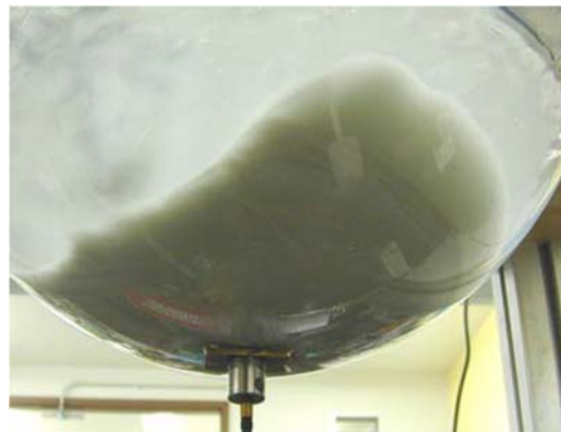
Figure C.2. PulseEcho Ultrasonic Transducer Monitoring the Thickness of an Uneven Sediment Bed
