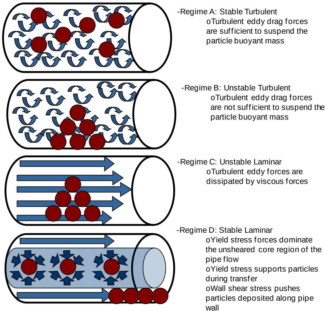
Figure 3.1. Graphical Interpretation of Four Major Slurry-Transport Flow Regimes
