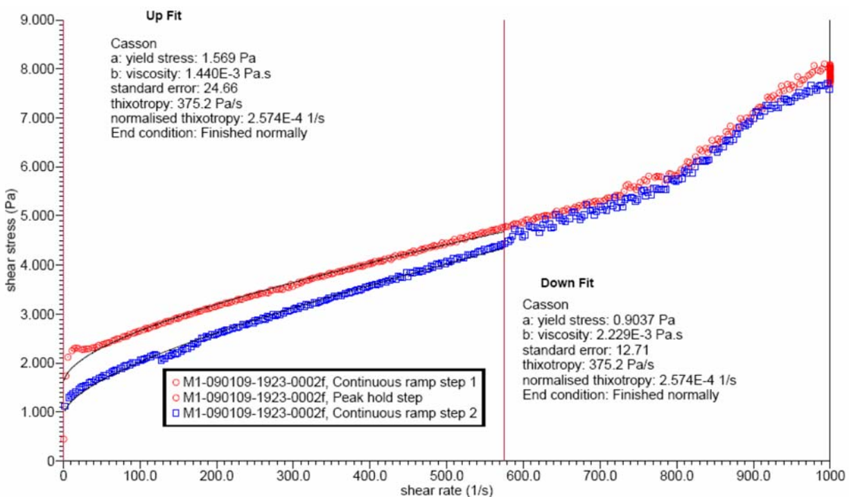
Figure D.34. Rheogram of the Only Physical and Rheological Complex-Simulant Sample Taken for TI-RPP-WTP-668
