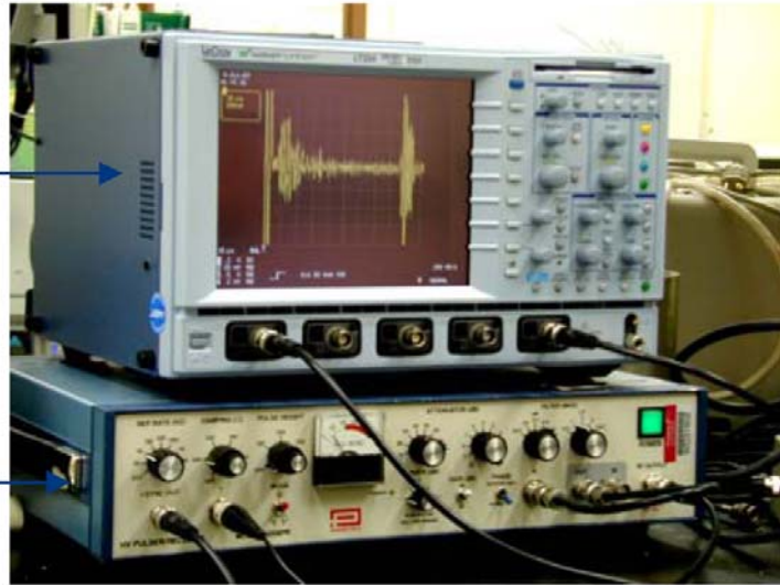
Figure C.7. Components of the PulseEcho Monitoring System
