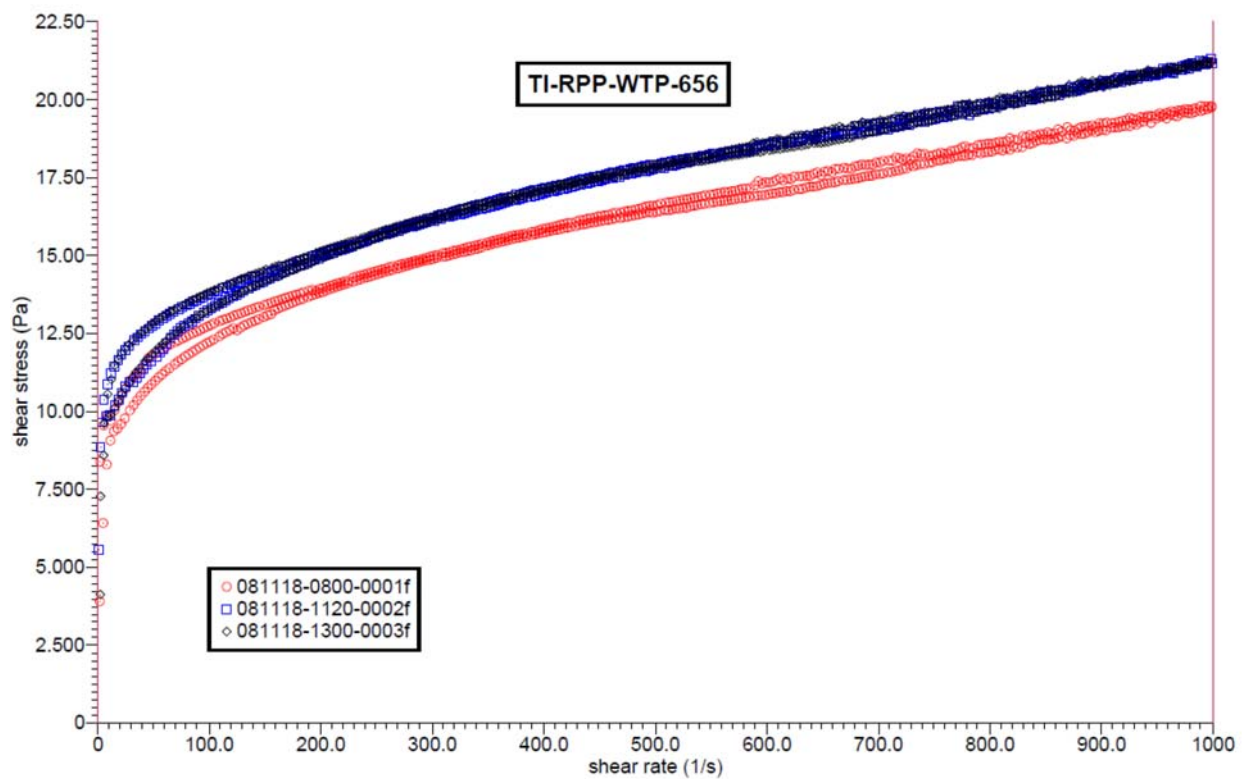
Figure D.8. Rheograms for All Samples Taken During TI-RPP-WTP-656
