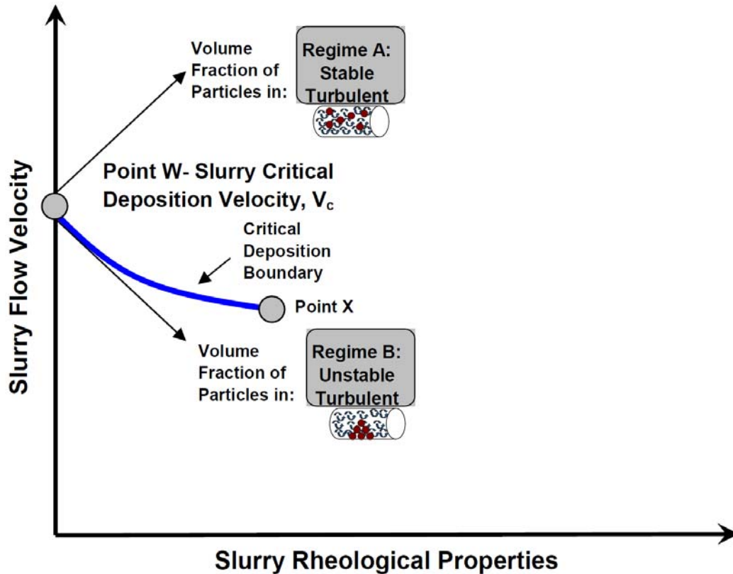
Figure 8.4. Schematic Showing a Design Approach for Newtonian Slurries of Setting a Maximum Velocity at which Turbulent Deposition Can Occur and Determining the Volume Fraction of Slurry Particles in Unstable Turbulent Flow
