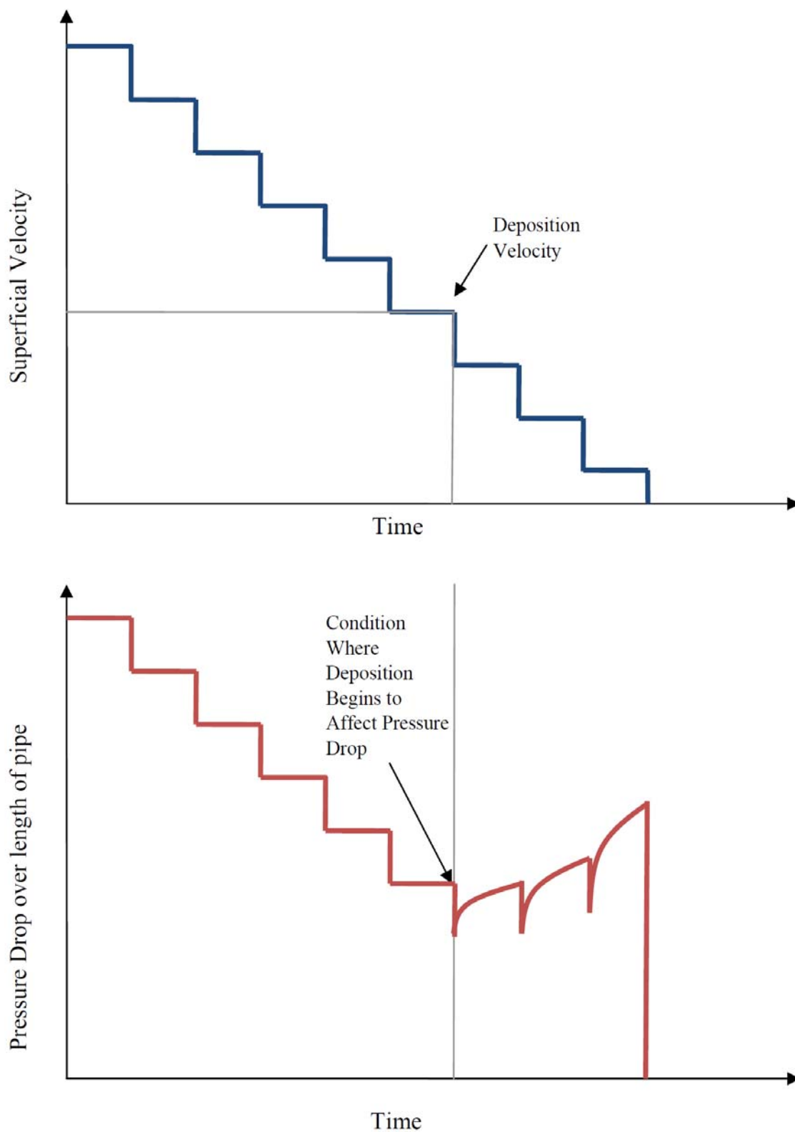
Figure 6.1. Example Data Showing Pressure Drop as a Function of Pipeline Superficial Velocity
