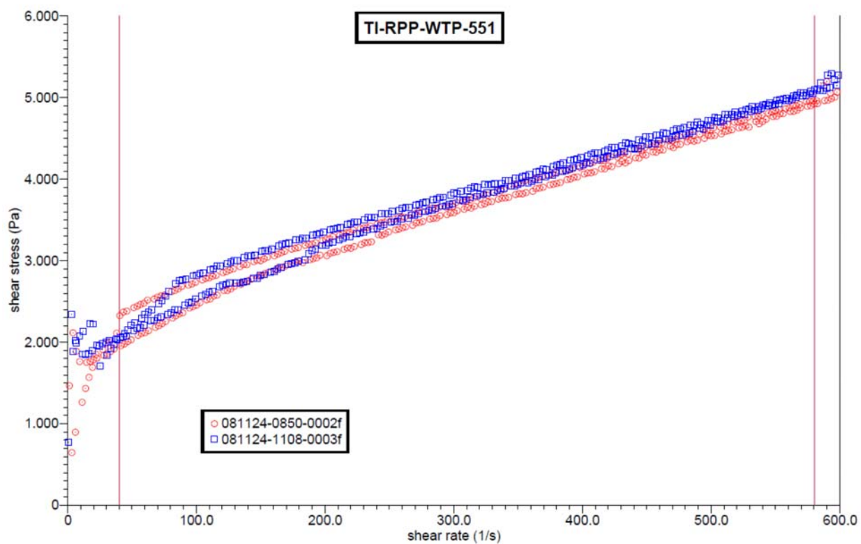
Figure D.18. Rheograms for All Samples Taken During TI-RPP-WTP-551
