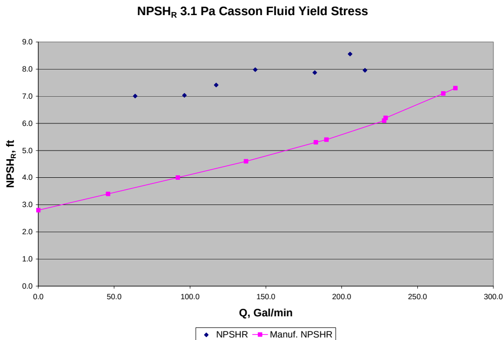
Figure 9.3. NPSH R Data for Casson-Fluid Yield Stress of Approximately 3.1 Pa; T Approximately 25°C. This test was conducted on 1/9/09. Head is calculated on a head-of-slurry basis.
