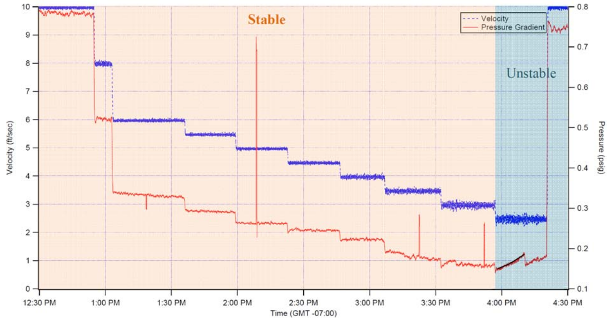
Figure B.7. Pressure-Gradient Data for Casson-Fluid Yield Stress of Approximately 3.1 Pa and Infinite-Shear Viscosity of 2.3 cP. This test was conducted on 1/9/09 after AFA addition. The pressure signal is stable until 2.5 ft/sec where an increase in pressure with time is observed. This slurry is considered to be unstable in a 3" pipe below 3.0 ft/sec.
