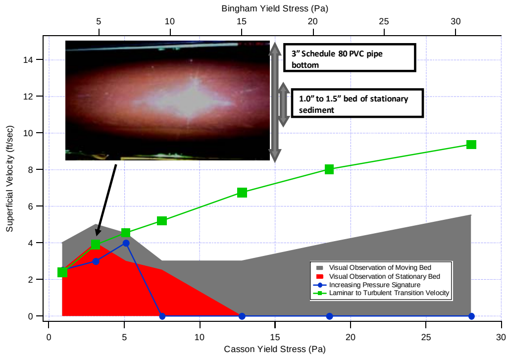
Figure 7.2. Stability Map for Simulant of AZ-101 HLW Pretreated Sludge With Deposition Velocities Determined by Pressure Signatures and Visual Observation in Transparent Pipe Section
