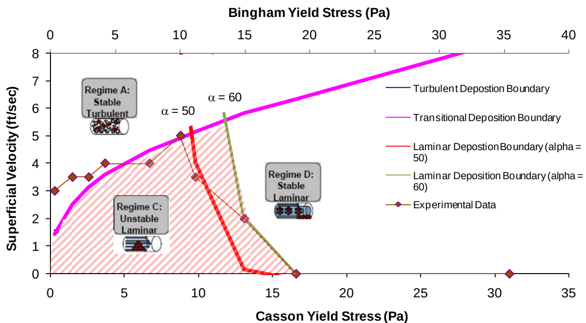
Figure 7.1. Stability Map for 150 μm Glass Beads and Corresponding Measured Deposition Velocity
