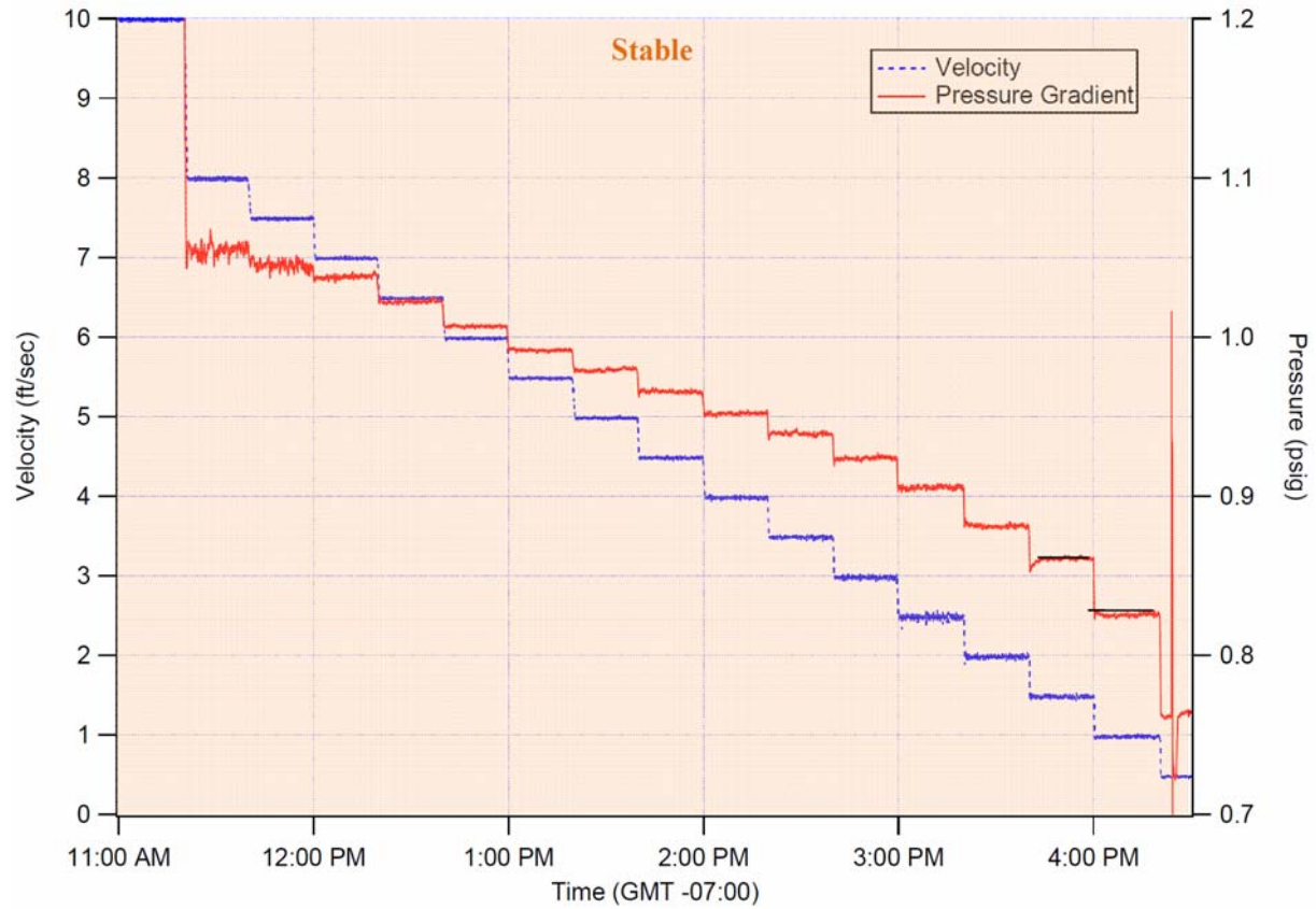
Figure A.2. Pressure-Gradient Data for Casson-Fluid Yield Stress of Approximately 16.6 Pa and Infinite-Shear Viscosity of 1.9 cP. This test was conducted on 11/13/08. The absence of the rheopexy observed in the 11/12/08 tests is due to the lower concentration of kaolin clay used in this test. Since no dramatic increase in pressure is observed at low velocities this slurry is considered to be stable in a 3" pipe.
