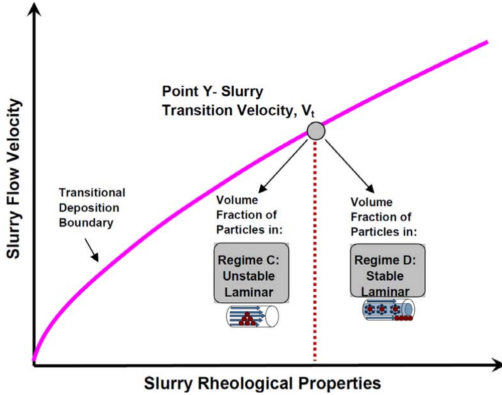
Figure 8.6. Schematic Showing a Design Approach for Non-Newtonian Slurries of Setting a Maximum Velocity at which Turbulent Flow Can Occur and Determining the Volume Fraction of Slurry Particles in Unstable Laminar Flow
