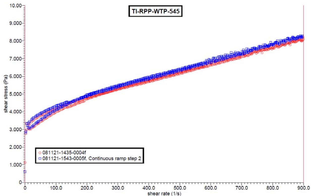
Figure D.16. Rheograms for All Samples Taken During TI-RPP-WTP-545
