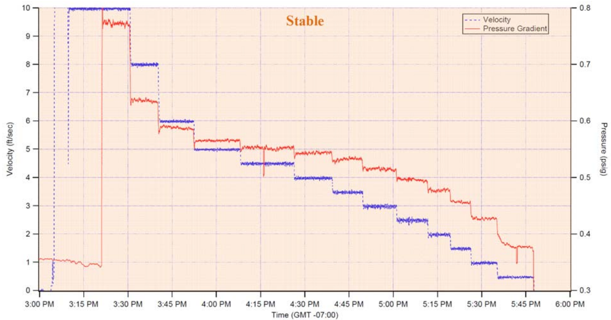
Figure B.4. Pressure-Gradient Data for Casson-Fluid Yield Stress of Approximately 7.5 Pa and Infinite-Shear Viscosity of 2.0 cP. This test was conducted on 1/5/09. Since no dramatic increase in pressure is observed at low velocities this slurry is considered to be stable in a 3" pipe.
