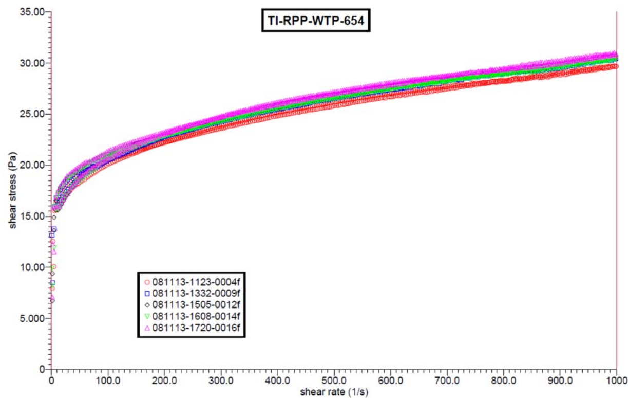
Figure D.4. Rheograms for All Samples Taken During TI-RPP-WTP-654
