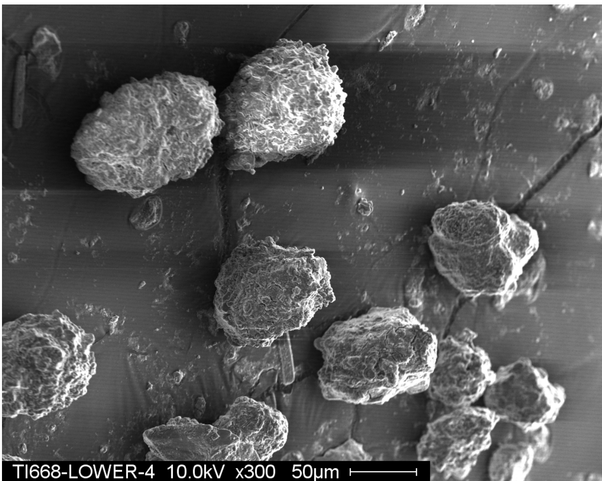
Figure 5.1. Micrograph of Fastest-Settling Particles in the Complex Simulant
