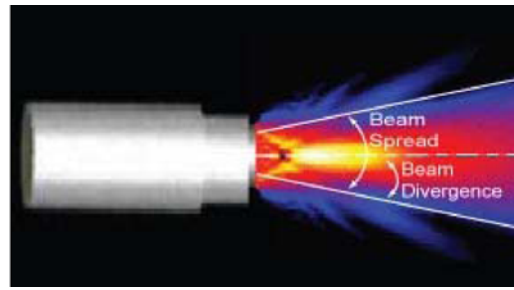
Figure C.1. Ultrasonic Transducer Emitting a Conical Sound Field. (Courtesy of the Center for Nondestructive Evaluation at Iowa State University)
