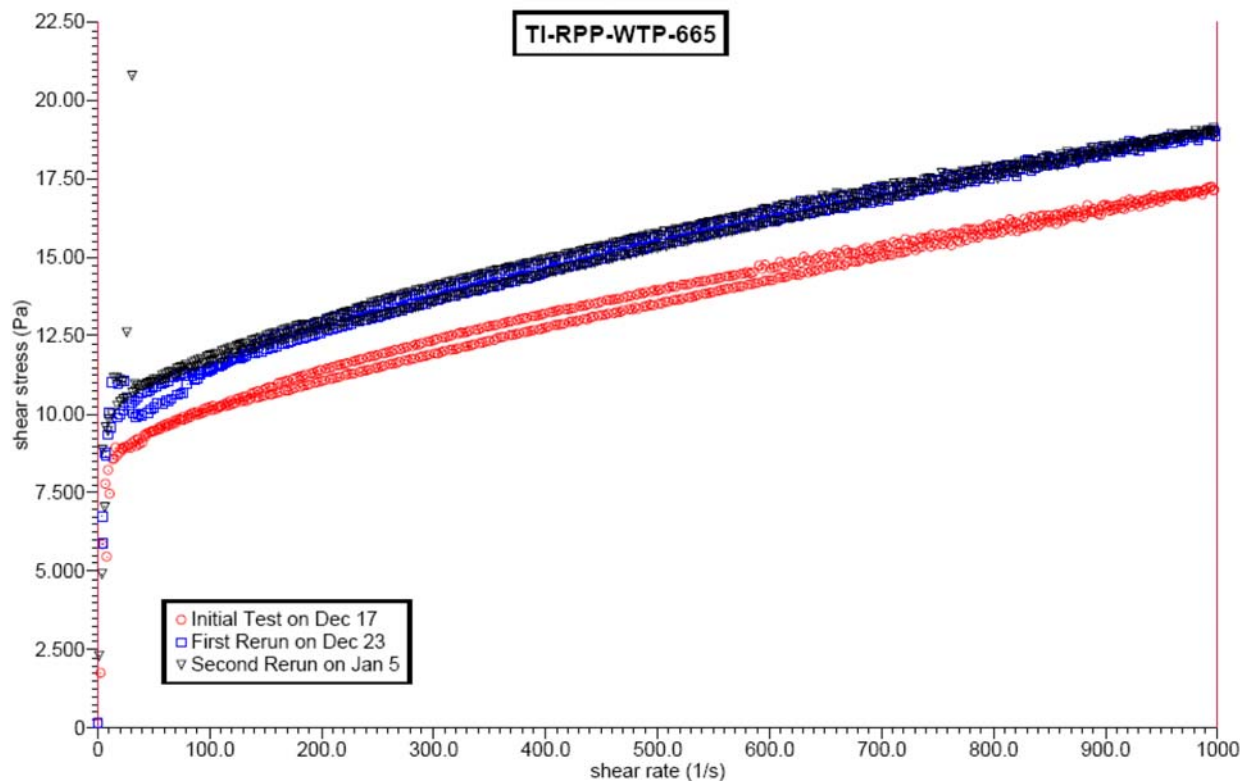
Figure D.28. Rheograms for All Samples Taken During TI-RPP-WTP-665
