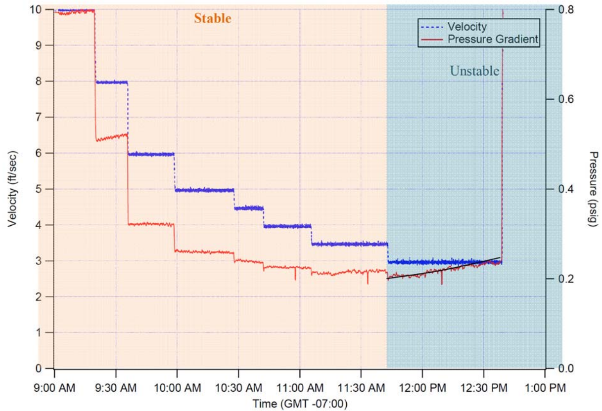
Figure B.6. Pressure-Gradient Data for Casson-Fluid Yield Stress of Approximately 2.6 Pa and Infinite-Shear Viscosity of 2.5 cP. This test was conducted on 1/8/09 prior to AFA addition. The pressure signal is stable until 3.0 ft/sec where an increase in pressure with time is observed. This slurry is considered to be unstable in a 3" pipe below 3.5 ft/sec.
