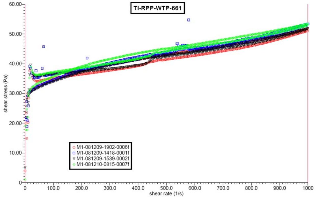
Figure D.22. Rheograms for All Samples Taken During TI-RPP-WTP-661
