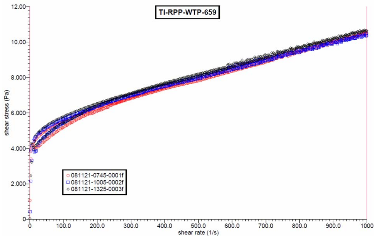
Figure D.14. Rheograms for All Samples Taken During TI-RPP-WTP-659
