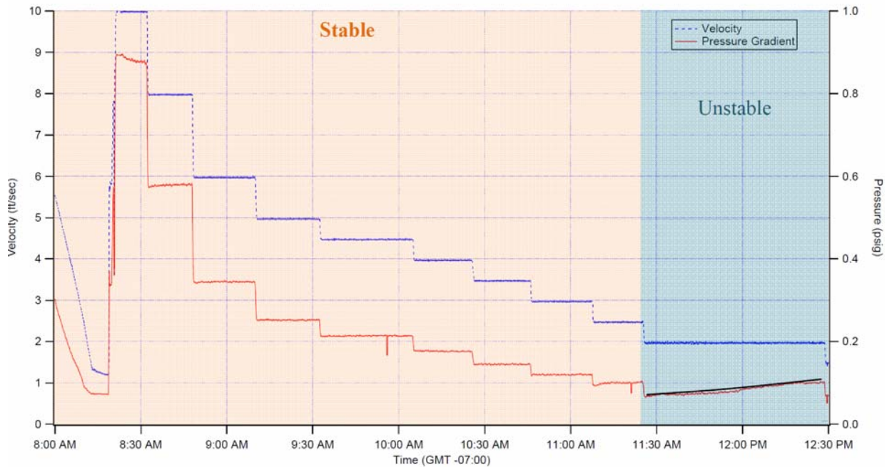
Figure B.8. Pressure-Gradient Data for Casson-Fluid Yield Stress of Approximately 0.9 Pa and Infinite-Shear Viscosity of 2.2 cP. This test was conducted on 1/10/09. The pressure signal is stable until 2.0 ft/sec where an increase in pressure with time is observed. This slurry is considered to be unstable in a 3" pipe below 2.5 ft/sec.
