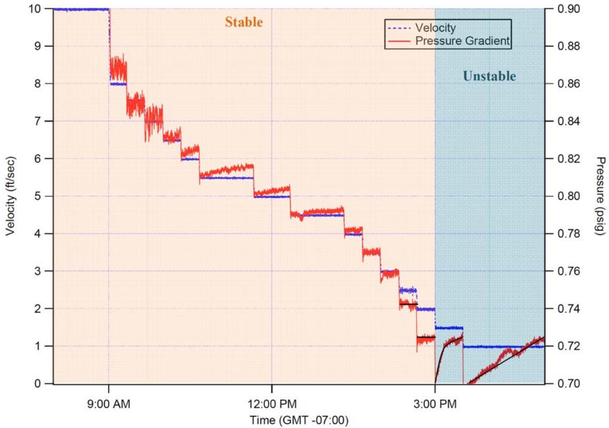
Figure A.3. Pressure-Gradient Data for Casson-Fluid Yield Stress of Approximately 13.1 Pa and Infinite-Shear Viscosity of 1.9 cP. This test was conducted on 11/14/08. Note the increase in pressure with time while running at 6 to 5 ft/sec. This is likely due to slurry entering the differential-pressure ports and creating a plug. The drop in pressure at a velocity of 4.5 ft/sec is from the pressure-port lines being purged with rinse water. The pressure signal is then stable until 1.5 ft/sec where an increase in pressure with time is observed. This slurry is considered to be unstable in a 3" pipe below 2 ft/sec.
