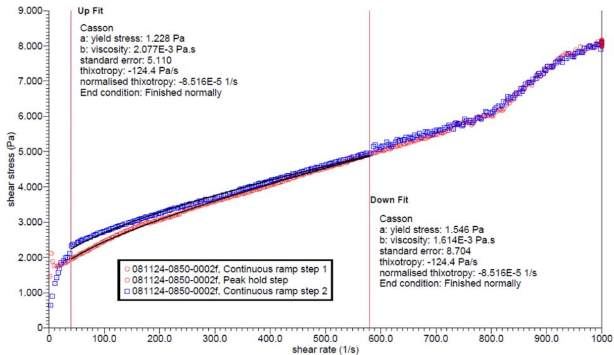
Figure D.17. Rheogram of Physical and Rheological Sample for TI-RPP-WTP-551
