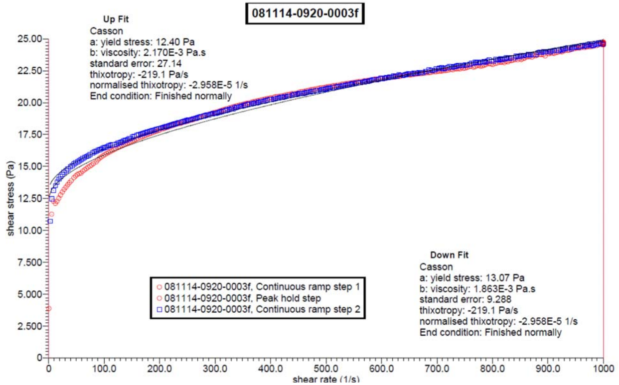
Figure D.5. Rheogram of Physical and Rheological Sample for TI-RPP-WTP-655
