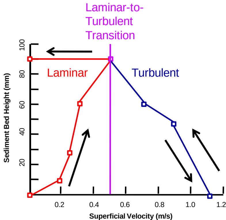
Figure 3.5. Sand-Clay Slurry Deposition Data in a Rectangular Pipeline; Arrows show the testing progression starting and ending with a superficial velocity of zero; Source: Song and Chiew (1997)
