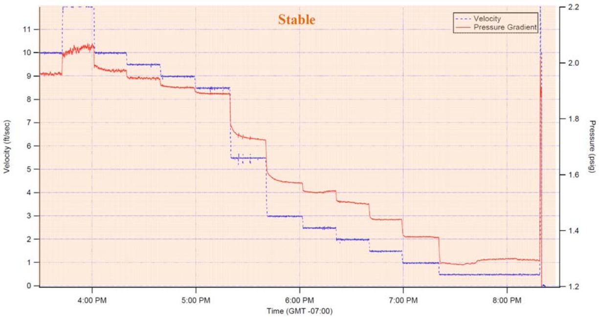
Figure B.1. Pressure-Gradient Data for Casson-Fluid Yield Stress of Approximately 28.0 Pa and Infinite-Shear Viscosity of 3.3 cP. This test was conducted on 12/9/08. Since no dramatic increase in pressure is observed at low velocities this slurry is considered to be stable in a 3" pipe.
