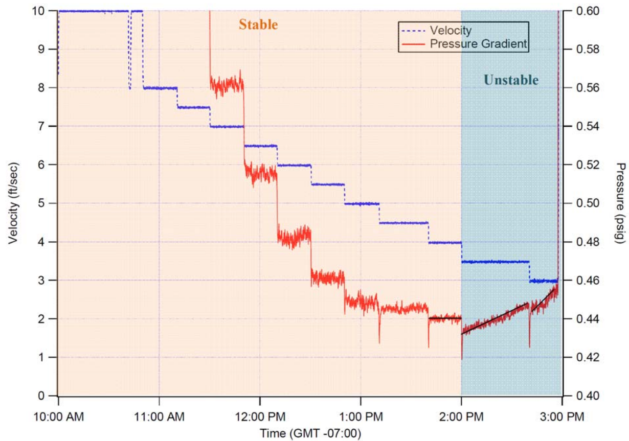
Figure A.6. Pressure-Gradient Data for Casson-Fluid Yield Stress of Approximately 6.7 Pa and Infinite-Shear Viscosity of 1.7 cP. This test was conducted on 11/20/08. The pressure signal is stable until 3.5 ft/sec where an increase in pressure with time is observed. This slurry is considered to be unstable in a 3" pipe below 4.0 ft/sec.
