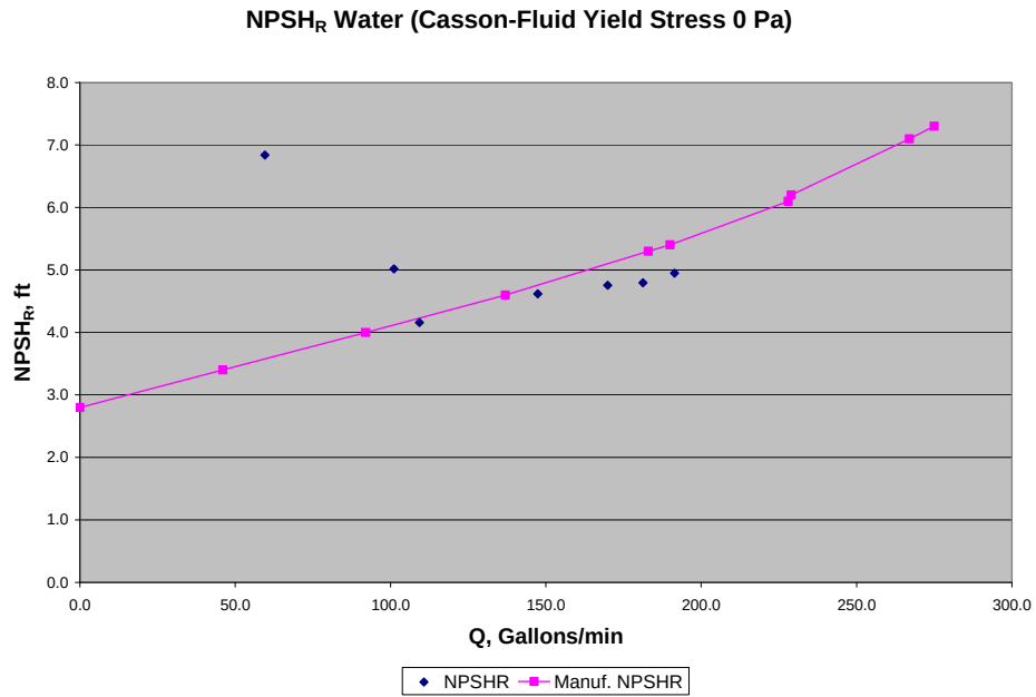
Figure 9.5. NPSH R Data for Process Water (Casson-Fluid Yield Stress 0 Pa); T Approximately 19°-23°C. This test was conducted on 1/19/09. Head is calculated on a head-of-water basis.
