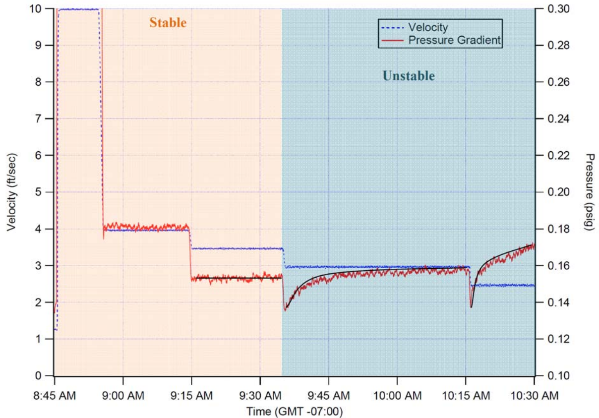
Figure A.9. Pressure-Gradient Data for Casson-Fluid Yield Stress of Approximately 1.5 Pa and Infinite-Shear Viscosity of 1.6 cP. This test was conducted on 11/24/08. The pressure signal is stable until 3.0 ft/sec where an increase in pressure with time is observed. This slurry is considered to be unstable in a 3" pipe below 3.5 ft/sec.
