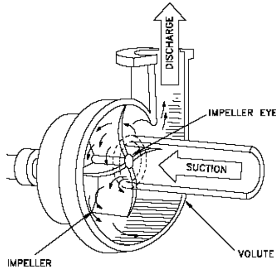
Figure 9.1. Principal Components of a Centrifugal Pump
