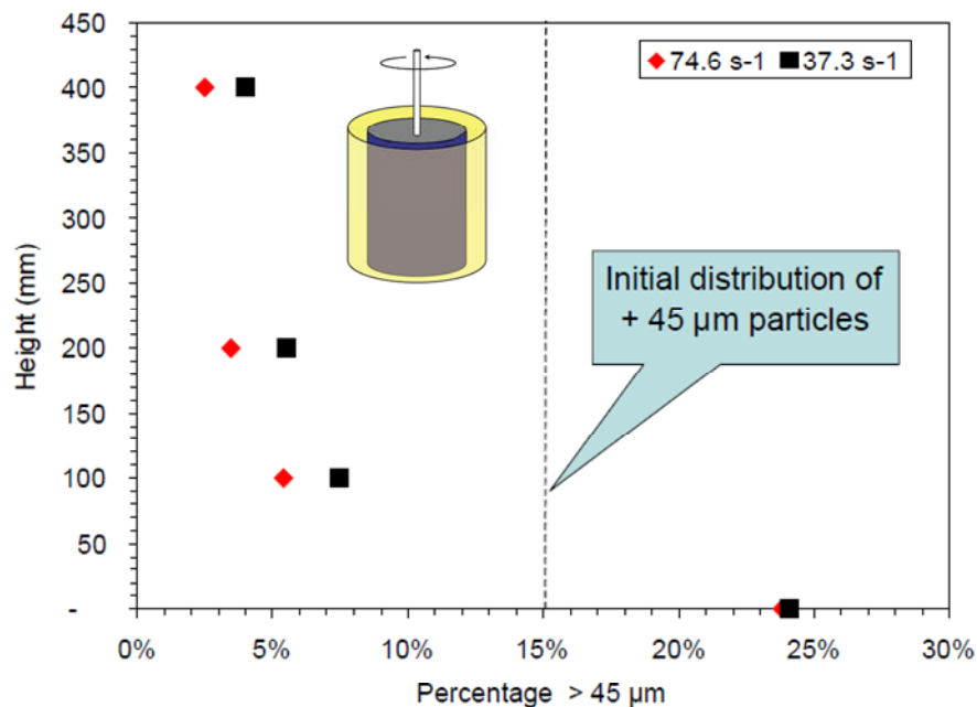
Figure 3.3. Laminar-Settling Test Data in Couette Flow; Source: Cook (2002)
