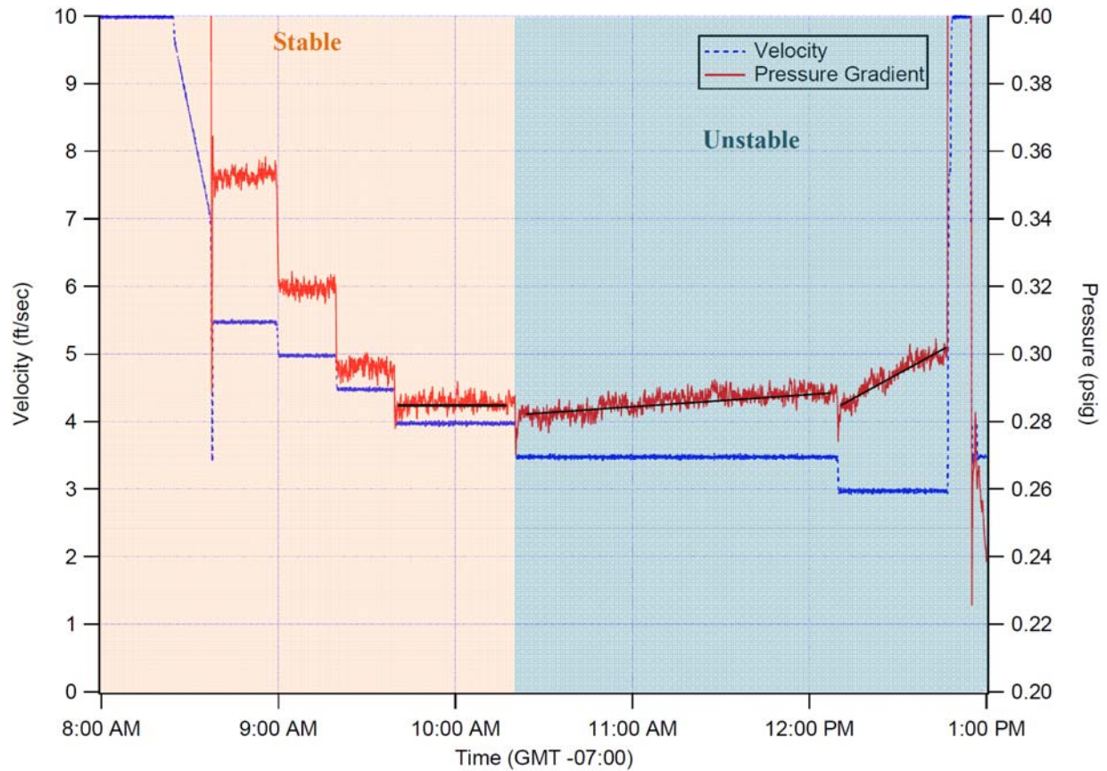
Figure A.7. Pressure-Gradient Data for Casson-Fluid Yield Stress of Approximately 3.7 Pa and Infinite-Shear Viscosity of 1.7 cP. This test was conducted on 11/21/08. The pressure signal is stable until 3.5 ft/sec where an increase in pressure with time is observed. This slurry is considered to be unstable in a 3" pipe below 4.0 ft/sec.
