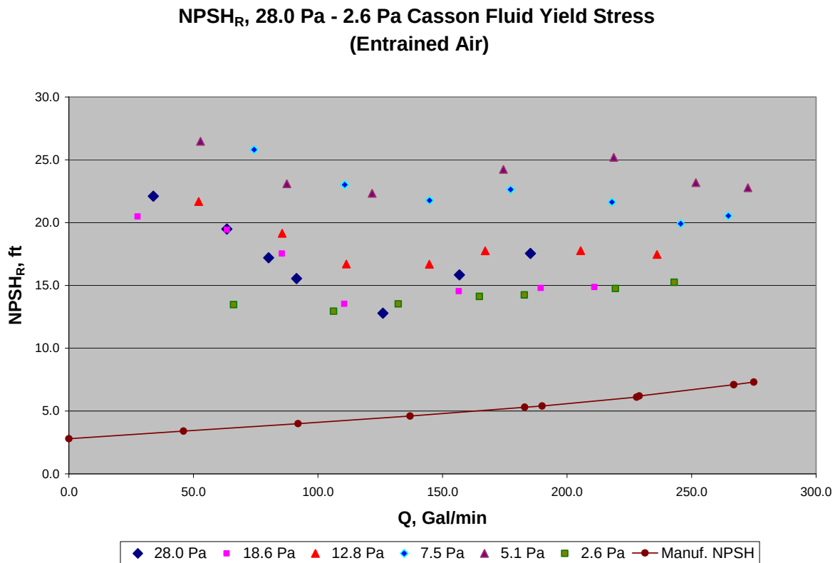
Figure 9.6. Apparent NPSH R Data for HLW Simulant (With Entrained Air) at Casson-Fluid Yield-Stress Range of 28.0 Pa to 2.6 Pa; All tests conducted at a 60 Hz VFD Setting. These tests were conducted from 12/10/08 to 1/6/09. Head is calculated on a head-of-slurry basis.
