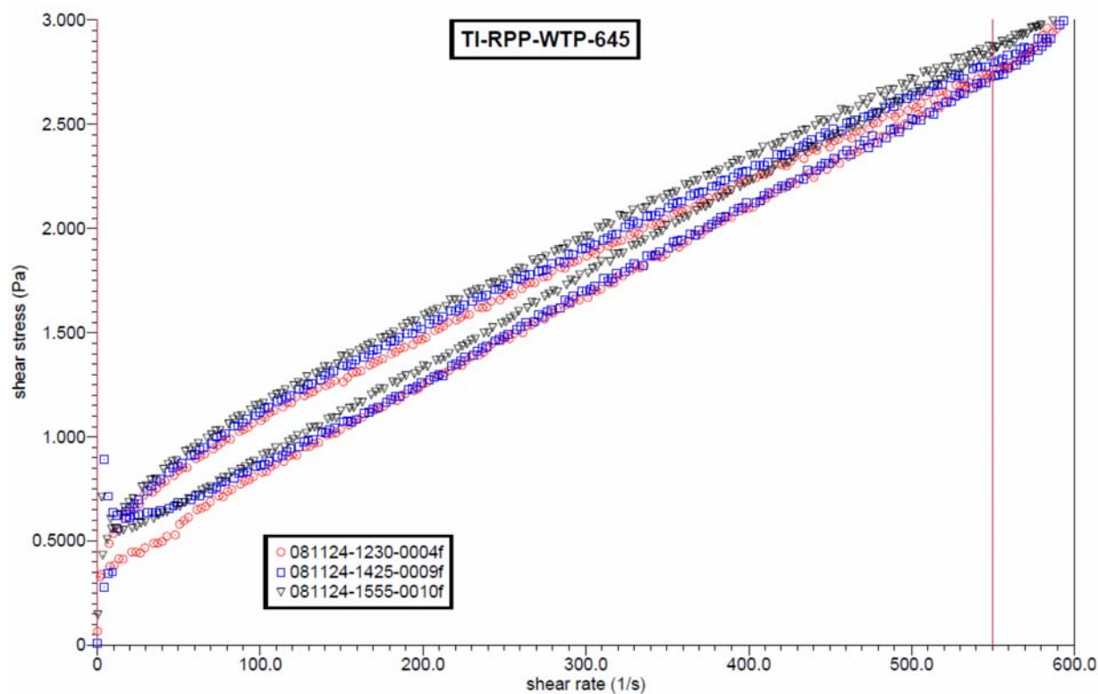
Figure D.20. Rheograms for All Samples Taken During TI-RPP-WTP-645
