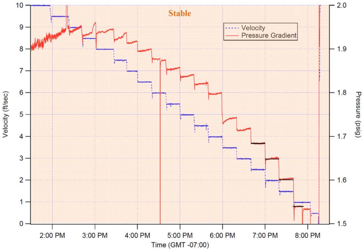
Figure A.1. Pressure-Gradient Data for Casson-Fluid Yield Stress of Approximately 31.0 Pa and Infinite-Shear Viscosity of 3.2 cP. This test was conducted on 11/12/08. Note the increasing pressure as a function of time at high velocities were due to the rheopexy (thickens as shearing continues) of kaolin clay slurries at higher concentrations. Since no dramatic increase in pressure is observed at low velocities this slurry is considered to be stable in a 3" pipe.
