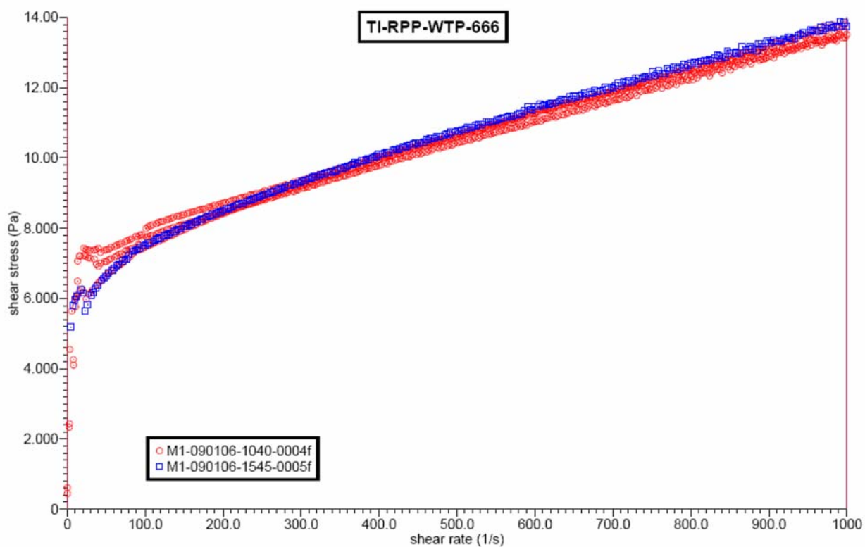
Figure D.30. Rheograms for All Samples Taken During TI-RPP-WTP-666
