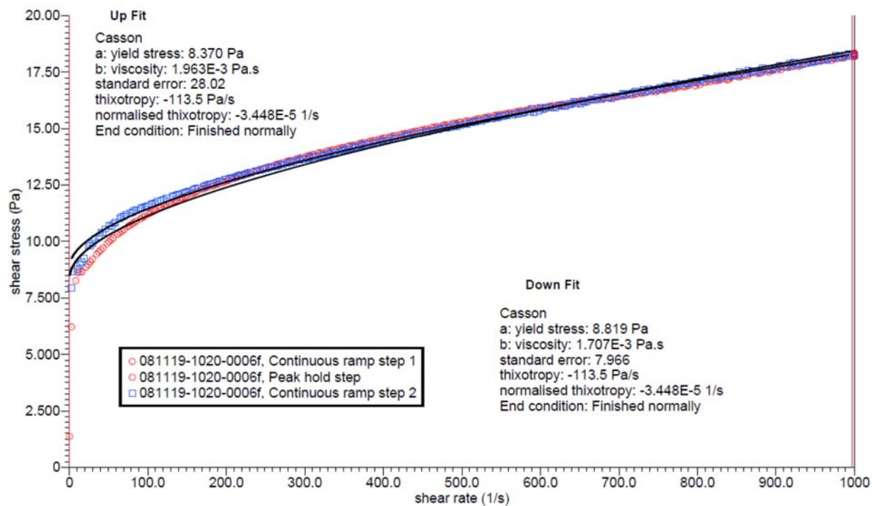
Figure D.9. Rheogram of Physical and Rheological Sample for TI-RPP-WTP-657
