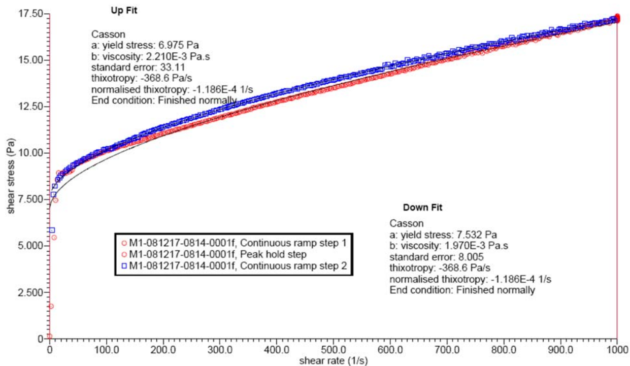
Figure D.27. Rheogram of Physical and Rheological Complex-Simulant Sample for TI-RPP-WTP-665
