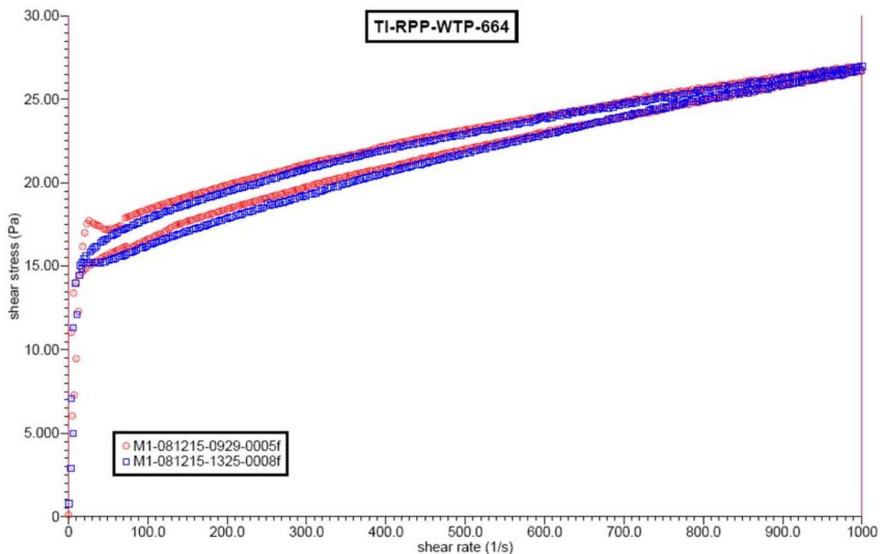
Figure D.26. Rheograms for All Samples Taken During TI-RPP-WTP-664
