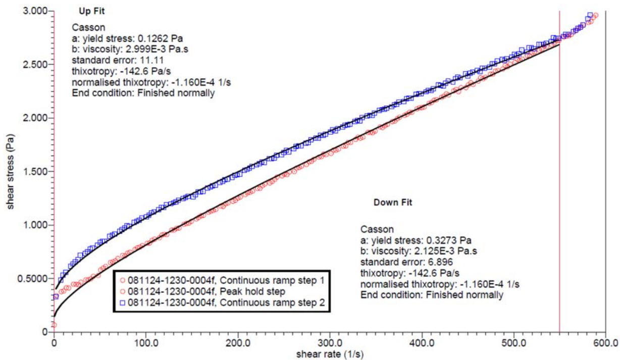
Figure D.19. Rheogram of Physical and Rheological Sample for TI-RPP-WTP-645
