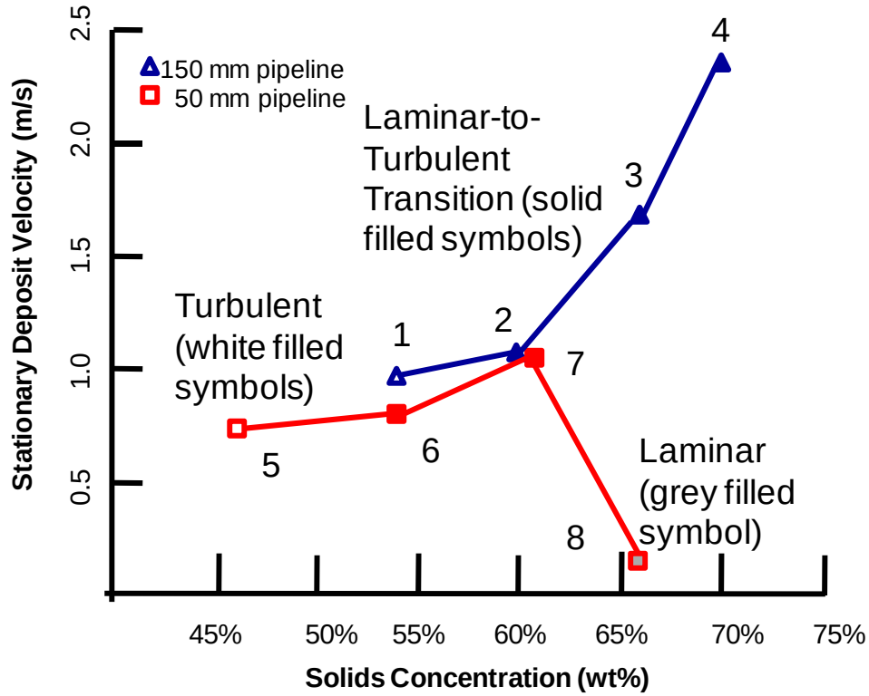
Figure 3.6. Copper-Tailings Deposition-Velocity Data; Source: Cooke (2002)
