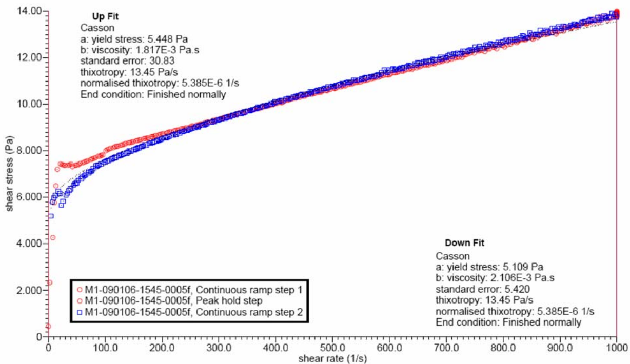
Figure D.29. Rheogram of Physical and Rheological Complex-Simulant Sample for TI-RPP-WTP-666
