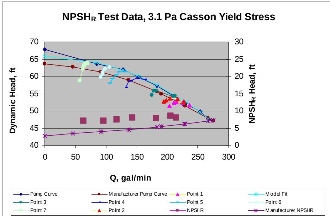
Figure 9.2. NPSH R Testing Data for Casson-Fluid Yield Stress of Approximately 3.1 Pa. the Manufacturer's Pump-Performance Curve and NPSH R Curves Are Shown, as well as NPSH R Data Points Collected. Head is Calculated on a Head-of-Slurry Basis
