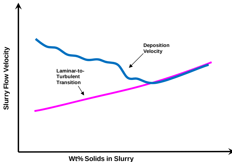
Figure 3.4. Relationship Between Deposition Velocity and Transition Velocity for an Example Slurry; Source: Ricks (2002)
