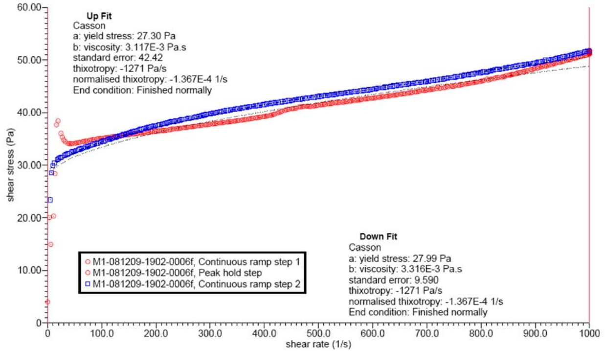
Figure D.21. Rheogram of Physical and Rheological Complex-Simulant Sample for TI-RPP-WTP-661
