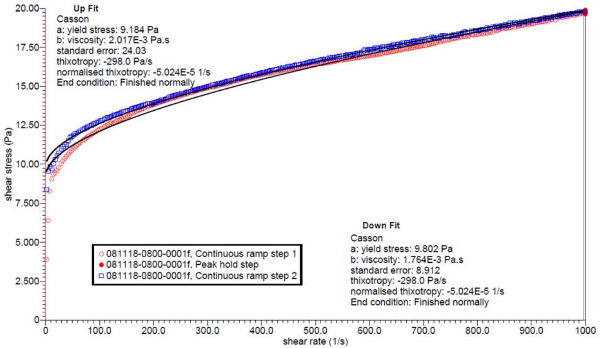
Figure D.7. Rheogram of Physical and Rheological Sample for TI-RPP-WTP-656
