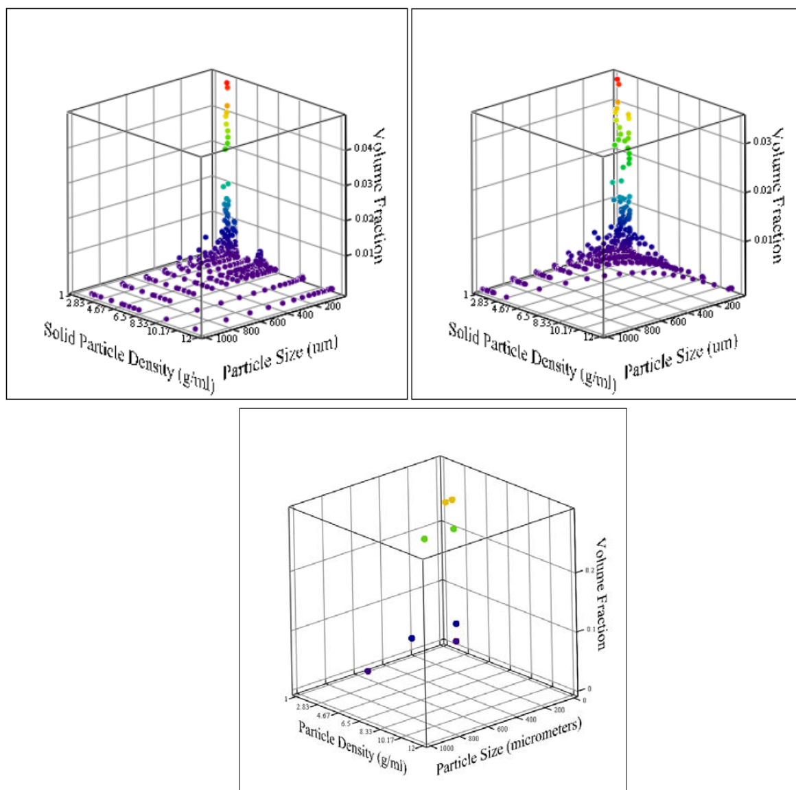
Figure 8.2. Wells et al. (2007; WTP-RPT-153 Rev. 0) Case 3 (Top-Left), Case 4 (Top-Right) and Jewett et al. (2002; RPP-9805; Bottom) Particle Size and Density Distributions
