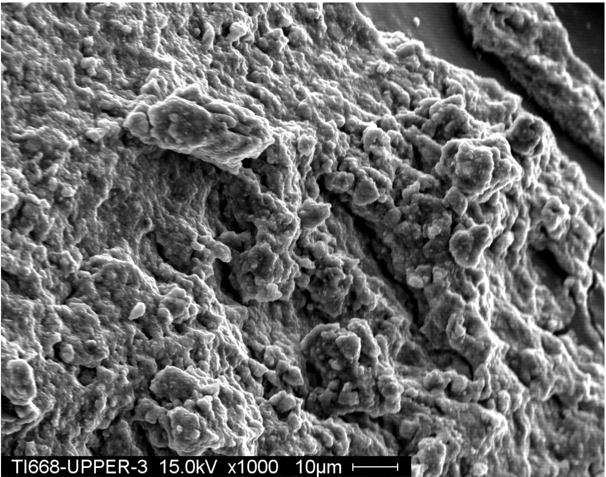
Figure 5.2. Micrograph of Slower-Settling Particles in the Complex Simulant
