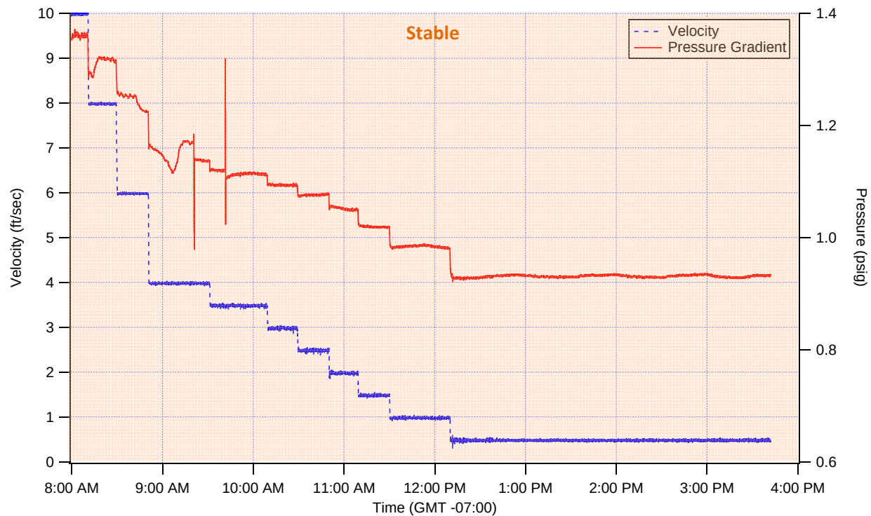
Figure B.2. Pressure-Gradient Data for Casson-Fluid Yield Stress of Approximately 18.6 Pa and Infinite-Shear Viscosity of 3.2 cP. This test was conducted on 12/11/08. Since no dramatic increase in pressure is observed at low velocities this slurry is considered to be stable in a 3" pipe.
