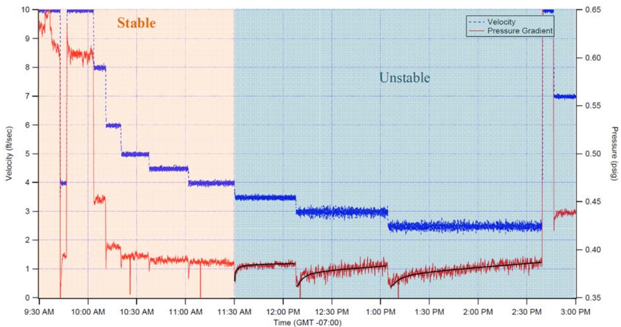
Figure B.5. Pressure-Gradient Data for Casson-Fluid Yield Stress of Approximately 5.1 Pa and Infinite-Shear Viscosity of 2.1 cP. This test was conducted on 1/6/09. The pressure signal is stable until 3.5 ft/sec where an increase in pressure with time is observed. This slurry is considered to be unstable in a 3" pipe below 4.0 ft/sec.
