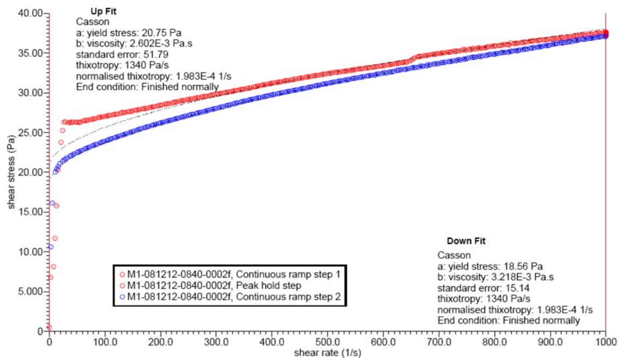
Figure D.23. Rheogram of Physical and Rheological Complex-Simulant Sample for TI-RPP-WTP-662
