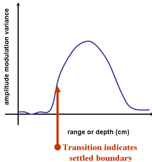
Figure C.5. Illustration of Pulse Echo Variance Algorithm
