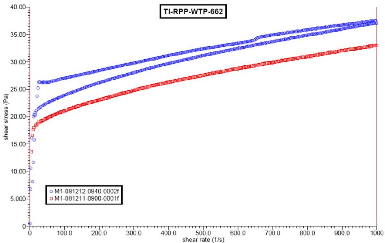
Figure D.24. Rheograms for All Samples Taken During TI-RPP-WTP-662
