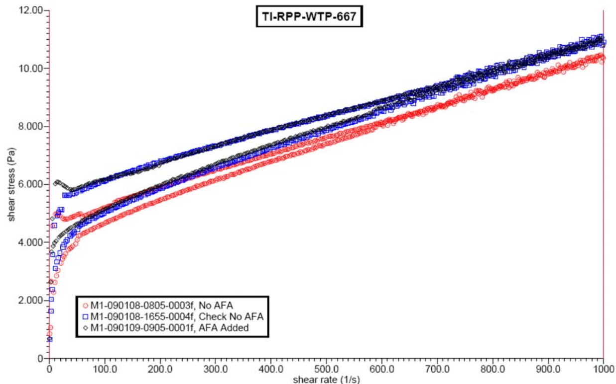
Figure D.33. Rheograms for All Samples Taken During TI-RPP-WTP-667
