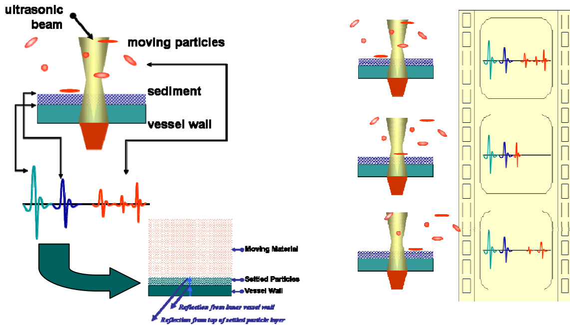
Figure C.6. Illustration of Pulse Echo Measurement and Signal-Processing Concepts
