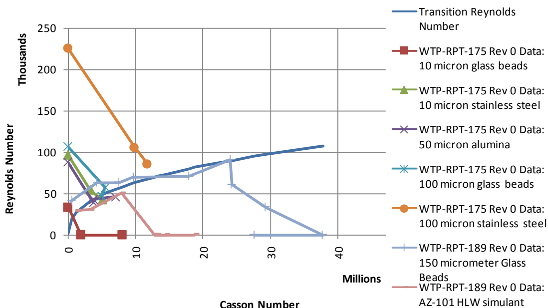
Figure S.2. Plot of Reynolds Number at Deposition for all Experimental Data from the M-1 Project; Reynolds Number at the Laminar to Turbulent Transition is also Plotted.
