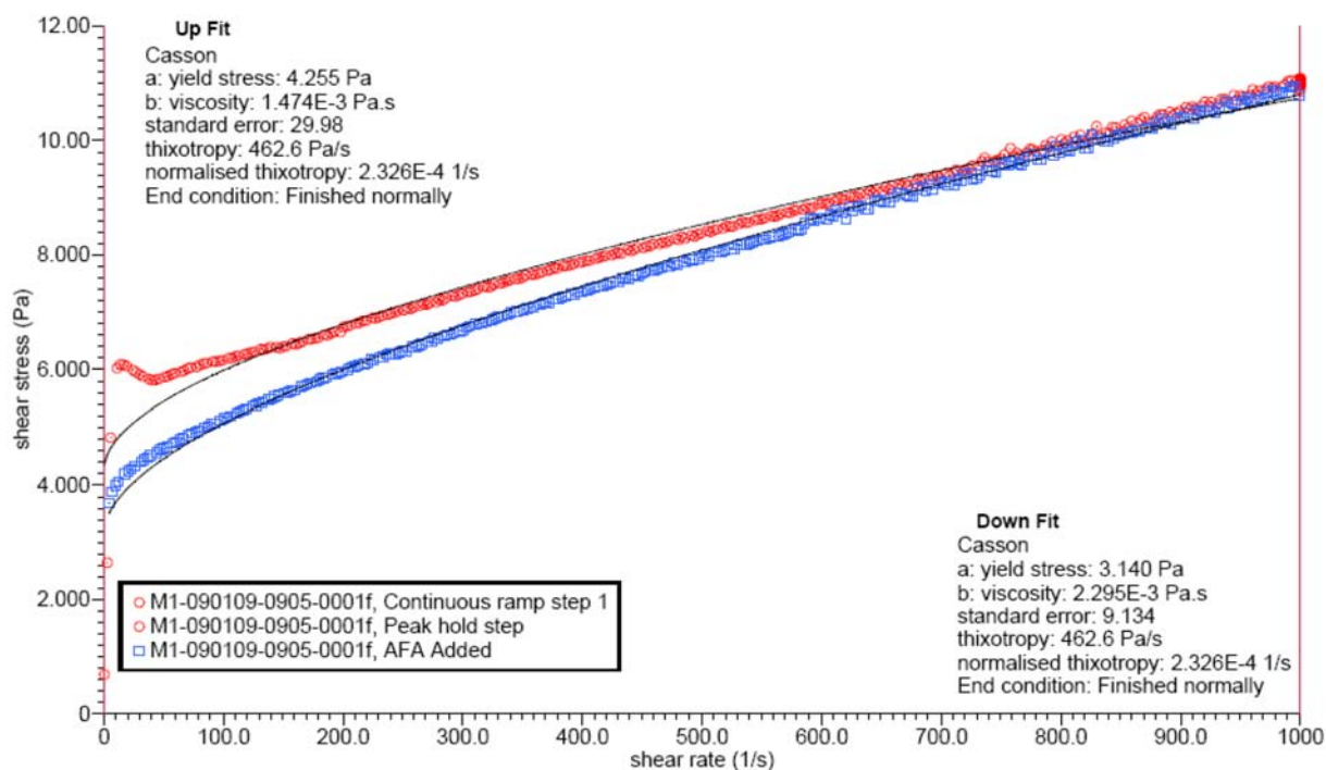
Figure D.32. Rheogram of Physical and Rheological Complex Simulant Sample for TI-RPP-WTP-667 After the Addition of AFA
