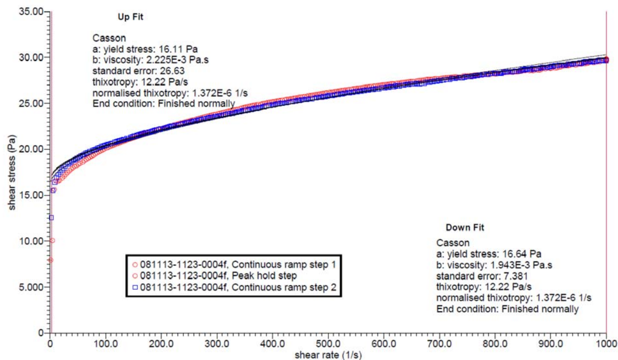
Figure D.3. Rheogram of Physical and Rheological Sample for TI-RPP-WTP-654
