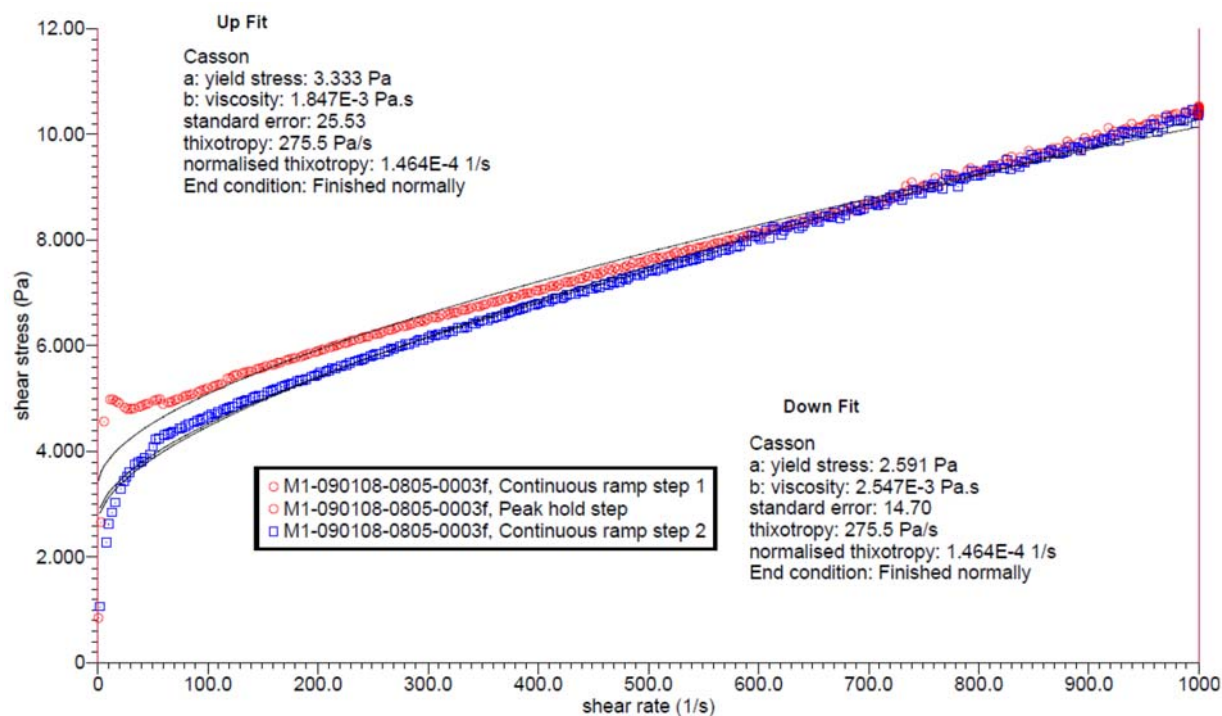
Figure D.31. Rheogram of Physical and Rheological Complex-Simulant Sample for TI-RPP-WTP-667 Prior to the Addition of AFA
