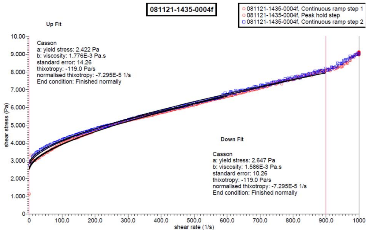
Figure D.15. Rheogram of Physical and Rheological Sample for TI-RPP-WTP-545
