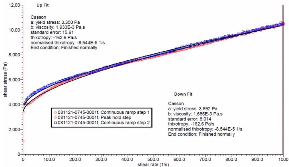
Figure D.13. Rheogram of Physical and Rheological Sample for TI-RPP-WTP-659
