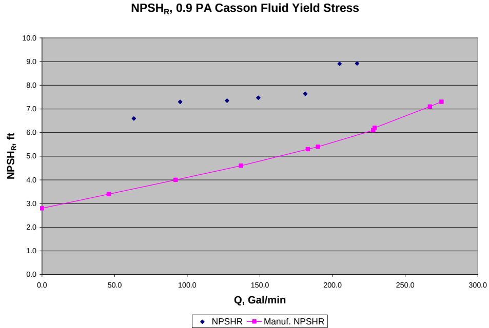
Figure 9.4. NPSH R Data for Casson-Fluid Yield Stress of Approximately 0.9 Pa; T Approximately 24°C. This test was conducted on 1/10/09. Head is calculated on a head-of-slurry basis.
