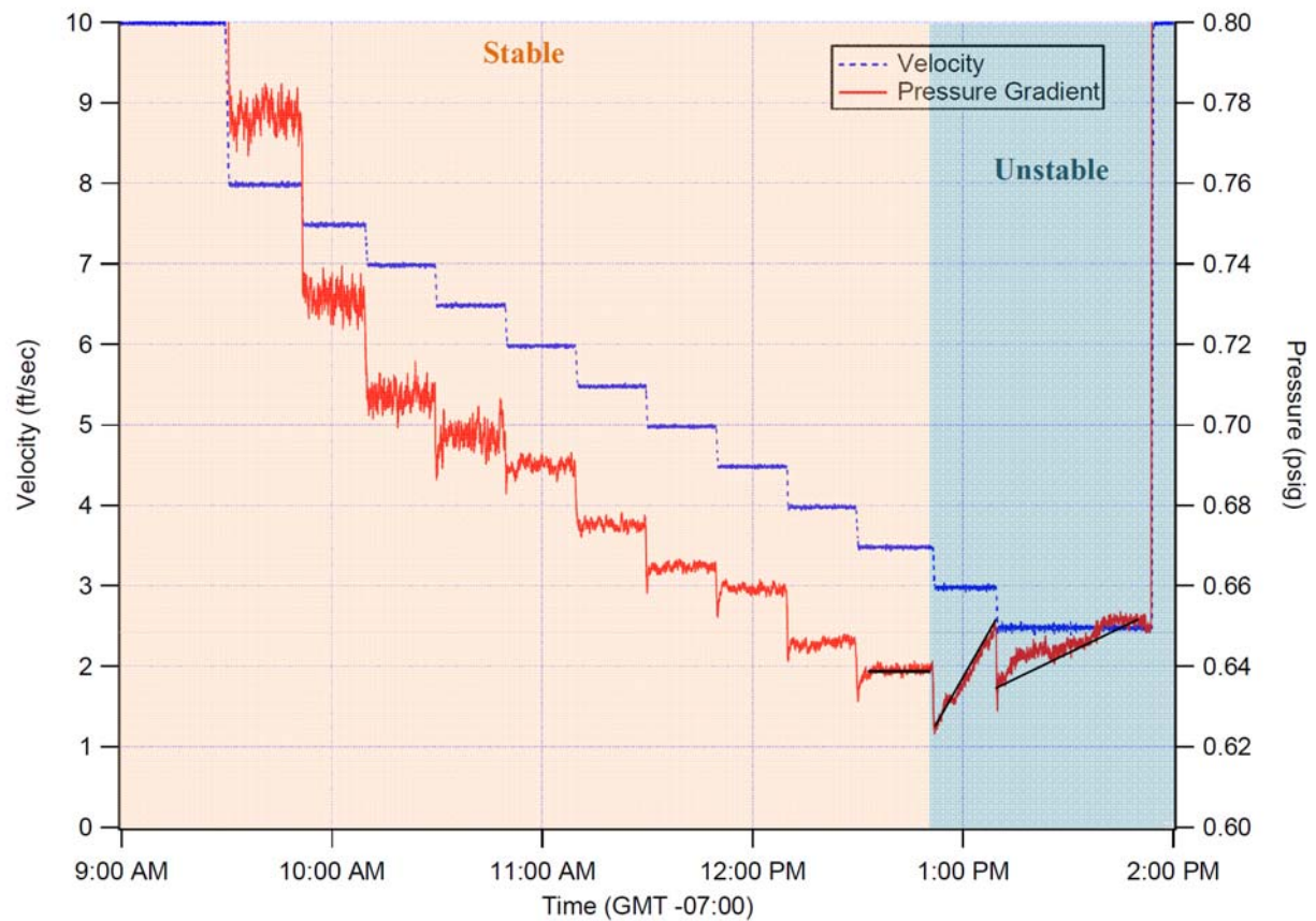
Figure A.4. Pressure-Gradient Data for Casson-Fluid Yield Stress of Approximately 9.8 Pa and Infinite-Shear Viscosity of 1.8 cP. This test was conducted on 11/18/08. The pressure signal is stable until 3.0 ft/sec where an increase in pressure with time is observed. This slurry is considered to be unstable in a 3" pipe below 3.5 ft/sec.
