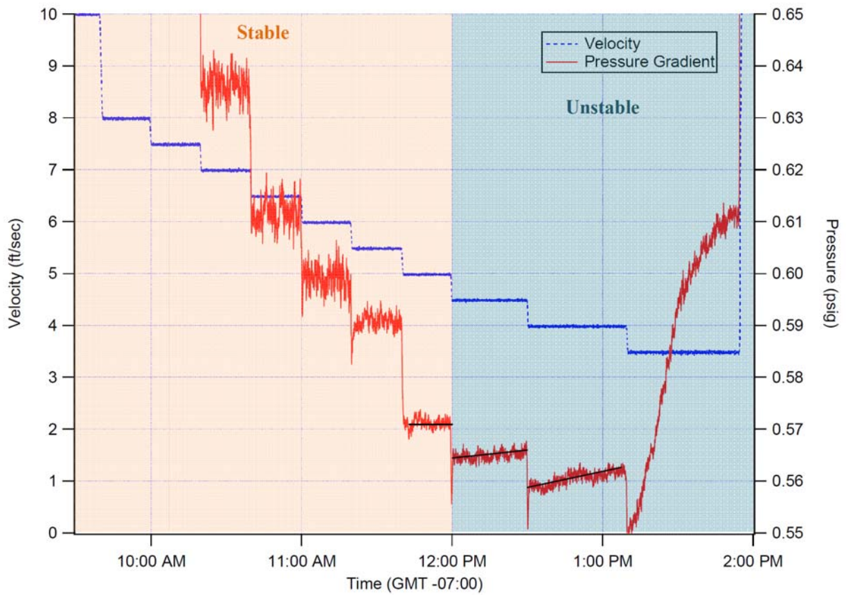
Figure A.5. Pressure-Gradient Data for Casson-Fluid Yield Stress of Approximately 8.8 Pa and Infinite-Shear Viscosity of 1.7 cP. This test was conducted on 11/19/08. The pressure signal is stable until 4.5 to 4.0 ft/sec where an increase in pressure with time is observed. Due to the slow increase in pressure observed at 4.5 ft/sec, this slurry is considered to be unstable in a 3" pipe below 5.0 ft/sec.
