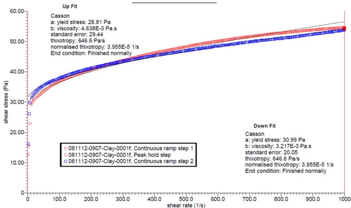
Figure D.1. Rheogram of Physical and Rheological Sample for TI-RPP-WTP-653
