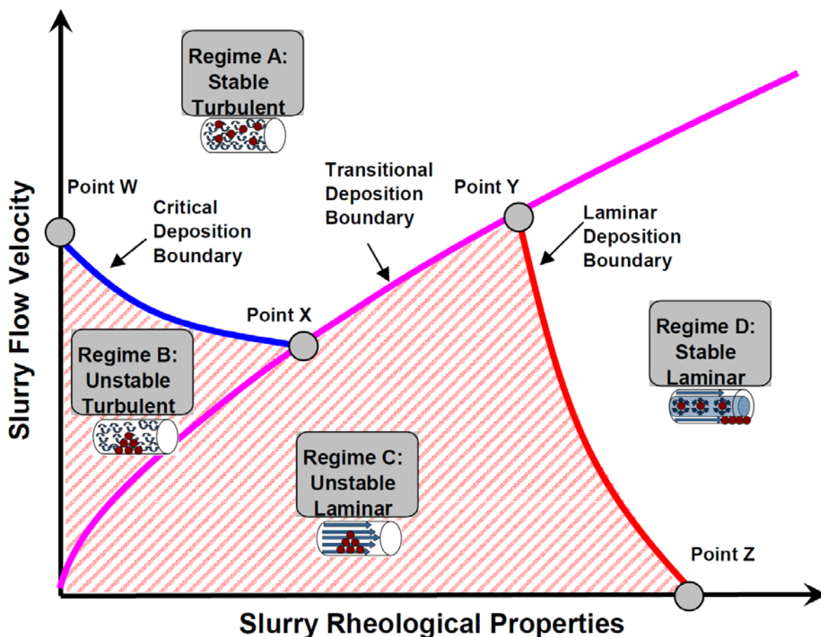
Figure 3.2. Graphical Illustration of a “Stability Map”
