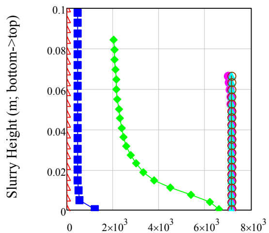
Shear Strength(Pa)
