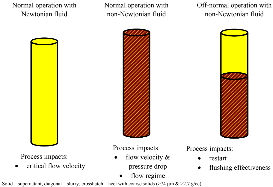
Figure S.2. Example Operational Scenarios for Vertical Process Piping
