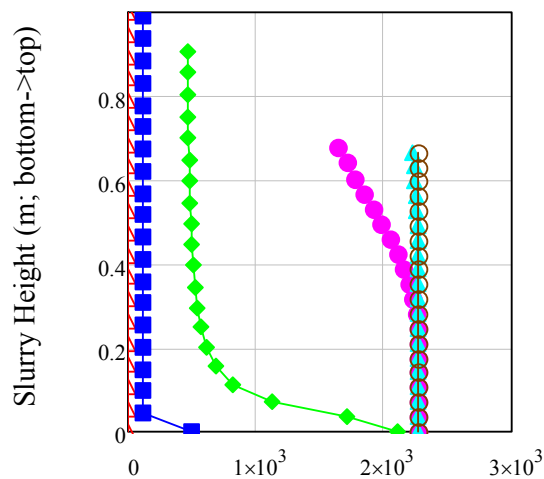
Shear Strength(Pa)
