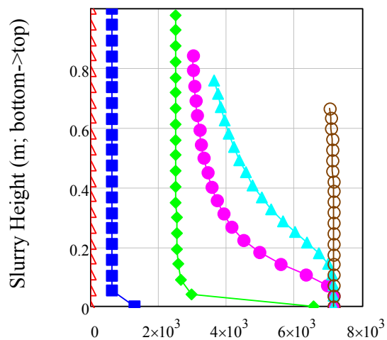
Shear Strength(Pa)
