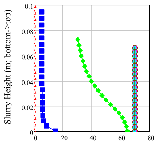
Shear Strength(Pa)
