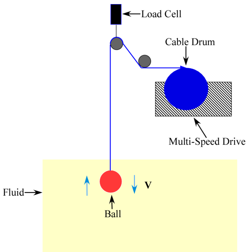
Figure 5.1. Schematic of the Falling Ball Rheometer
