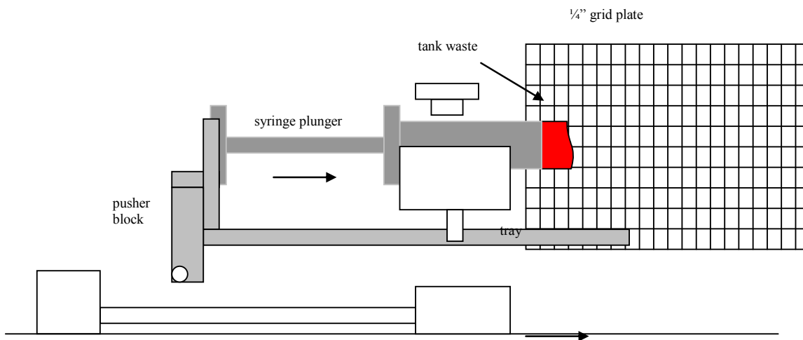
Figure 5.4. Mini-Extrusion Design
