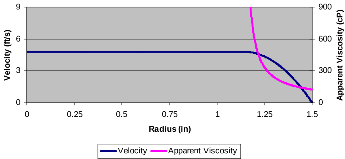
Figure 4.3. Example Flow Profiles for a Bingham Plastic Fluid (30 cP consistency, 30 Pa yield stress) in a 3-inch-ID Smooth Pipe at 90 gpm
