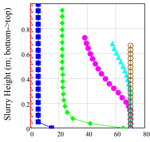
Shear Strength(Pa)
