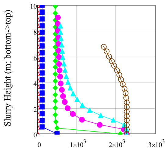
Shear Strength(Pa)
