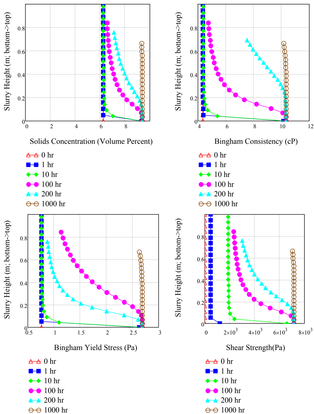
Figure 13.3. Predicted Sludge Properties from Hanford Tank C-104 with Water Dilution at Starting Slurry Height of 1 M with 33% Volume Excess Supernatant from Fully Settled Configuration; Rheological Properties Taken at a Temperature Range of 20°–35°C
