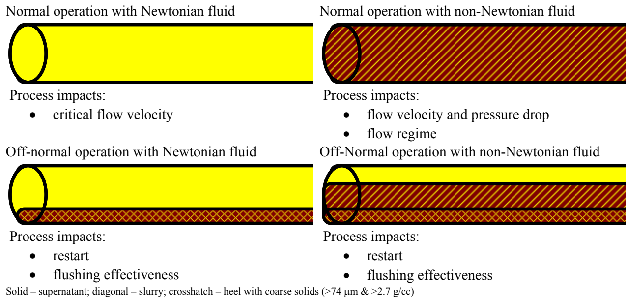
Figure S.3. Example Operational Scenarios for Horizontal Process Piping
