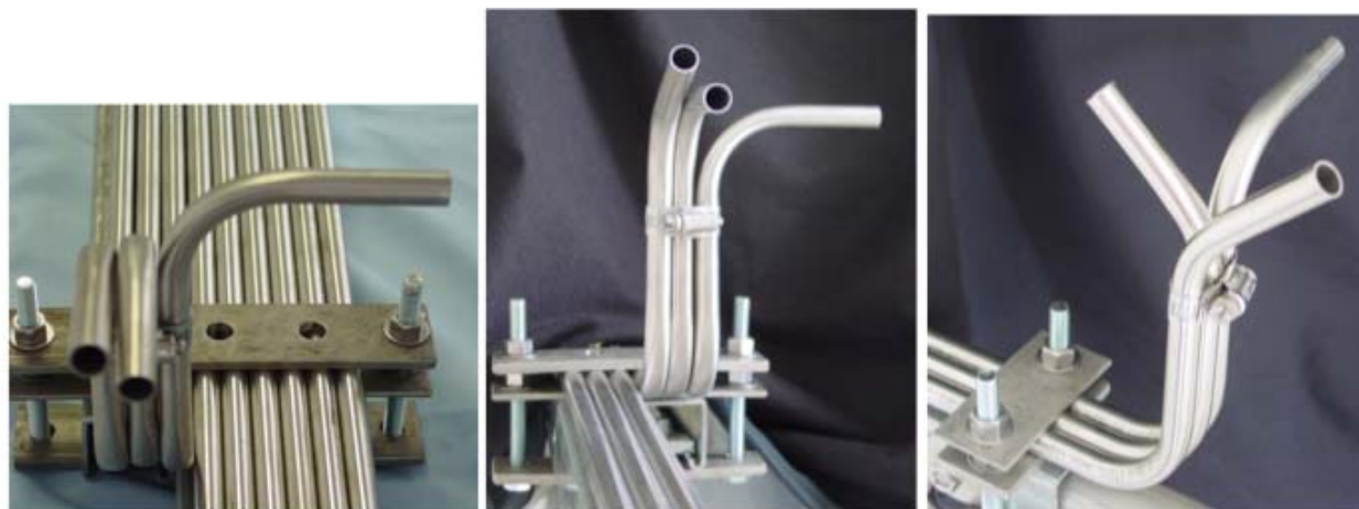
Figure 3.4. In-Tank Pressure Sensor Mounting Tubes at Top (Left), Middle (Center) and Bottom (Right) Elevations
