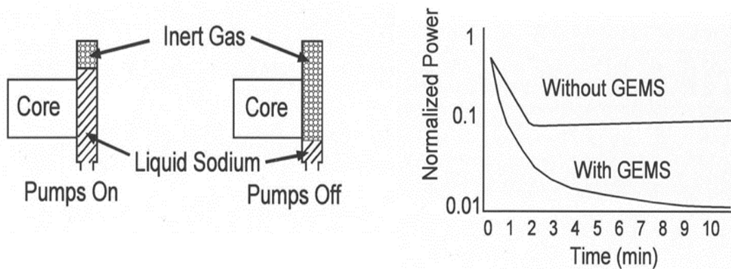
FIG. 2. Gas expansion module (GEM)
