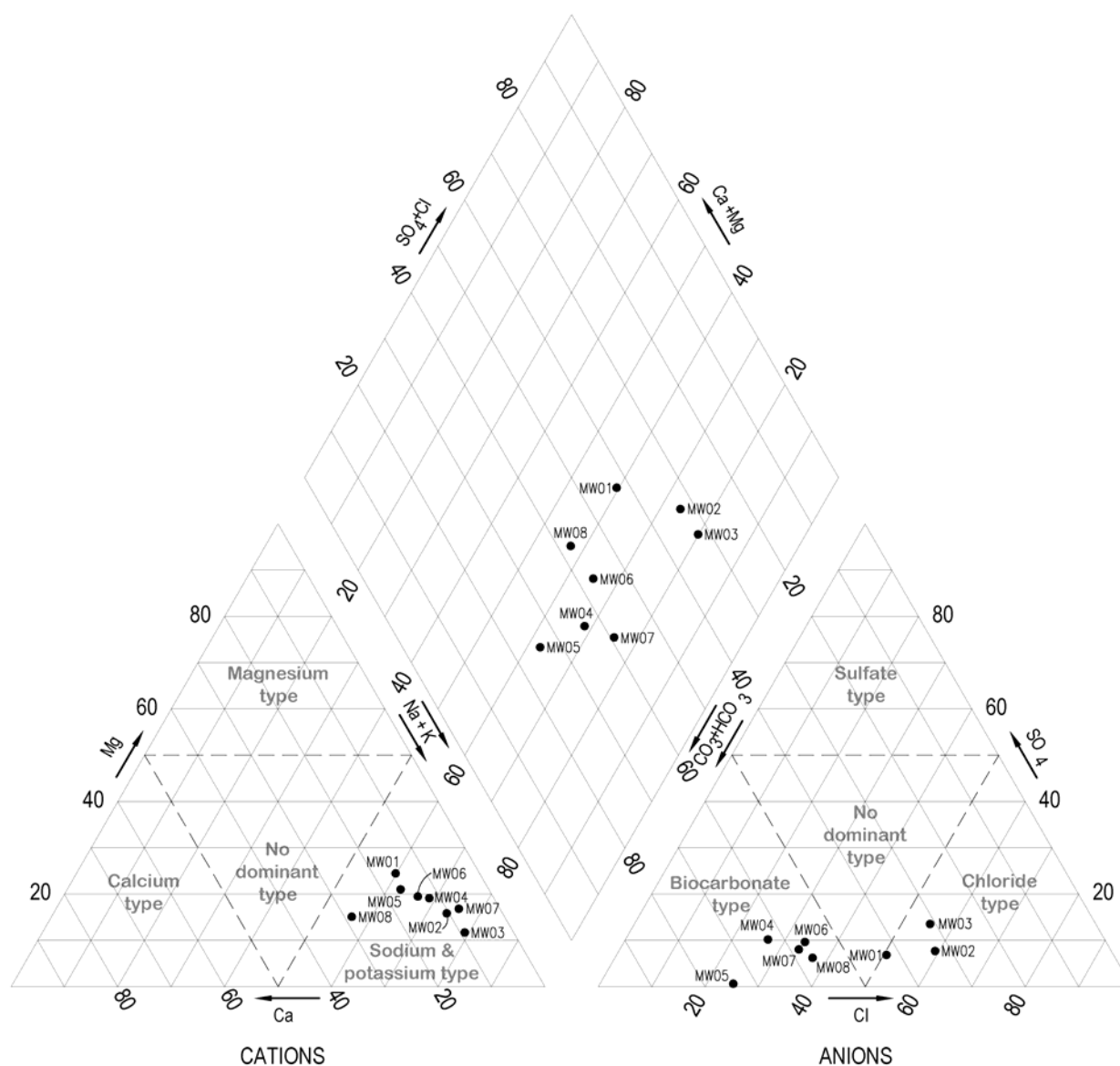
FIGURE 5-5. Piper trilinear diagram Round 1, investigation site
