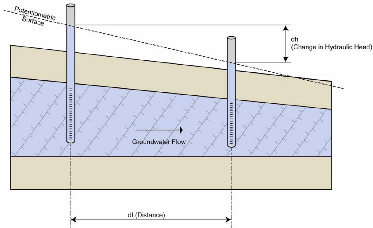
FIGURE 2-4. Hydraulic gradient
