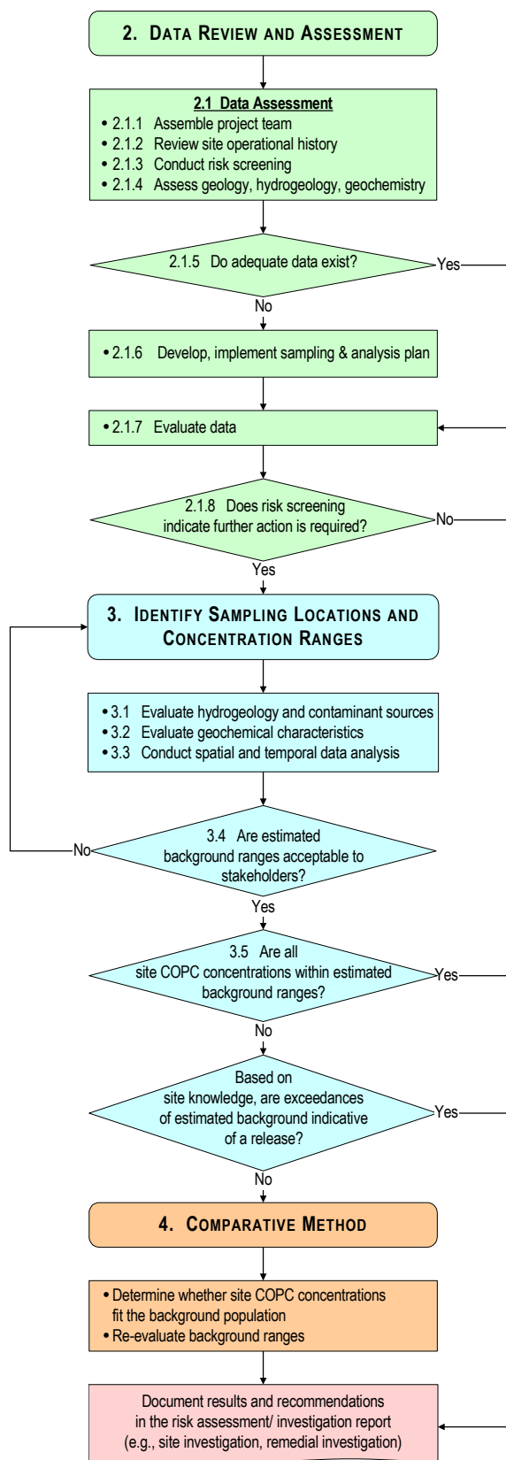
FIGURE 1-4. Typical background data evaluation and comparative statistical testing for groundwater COPCs
