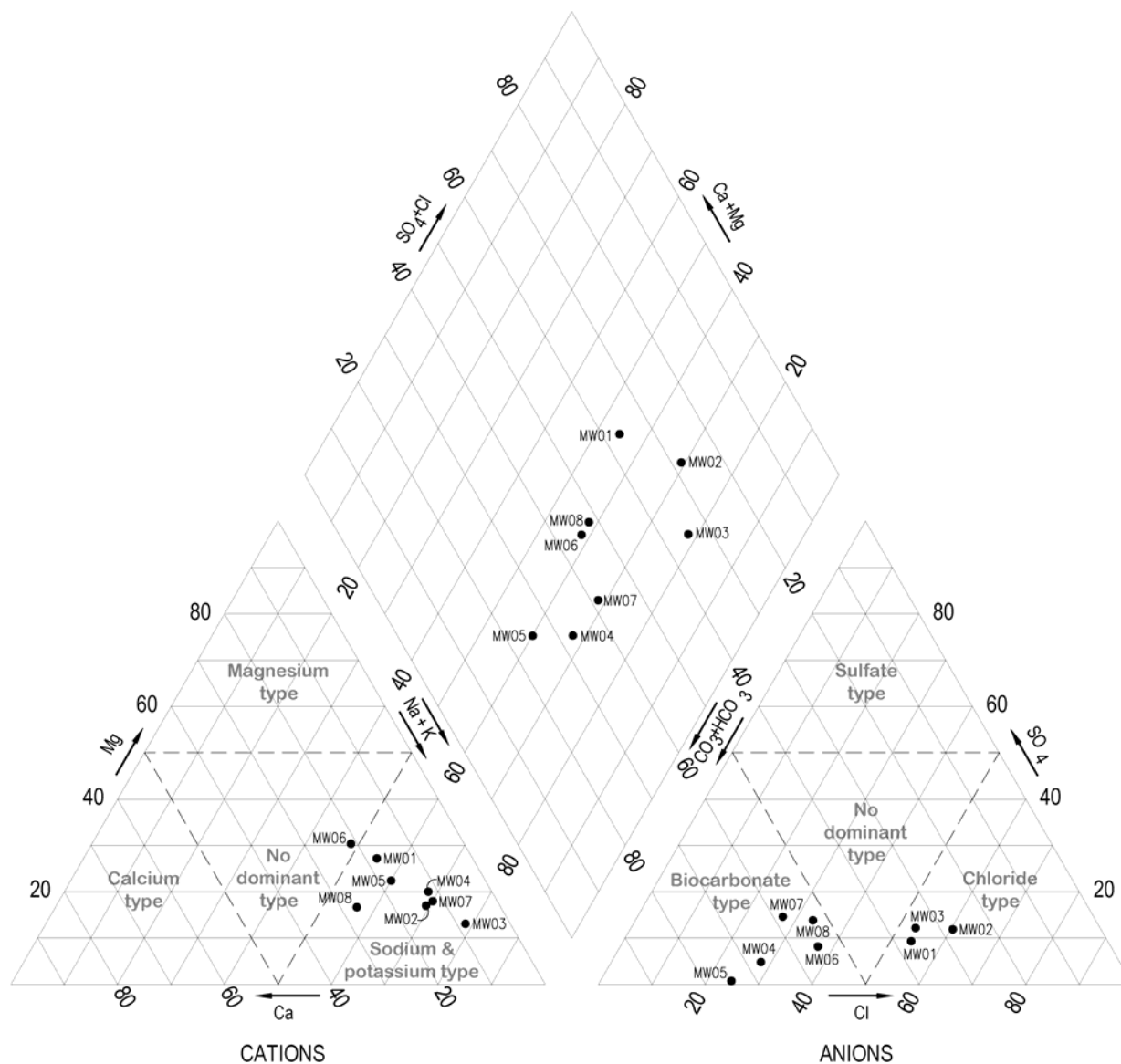
FIGURE 5-6. Piper trilinear diagram Round 2, investigation site
