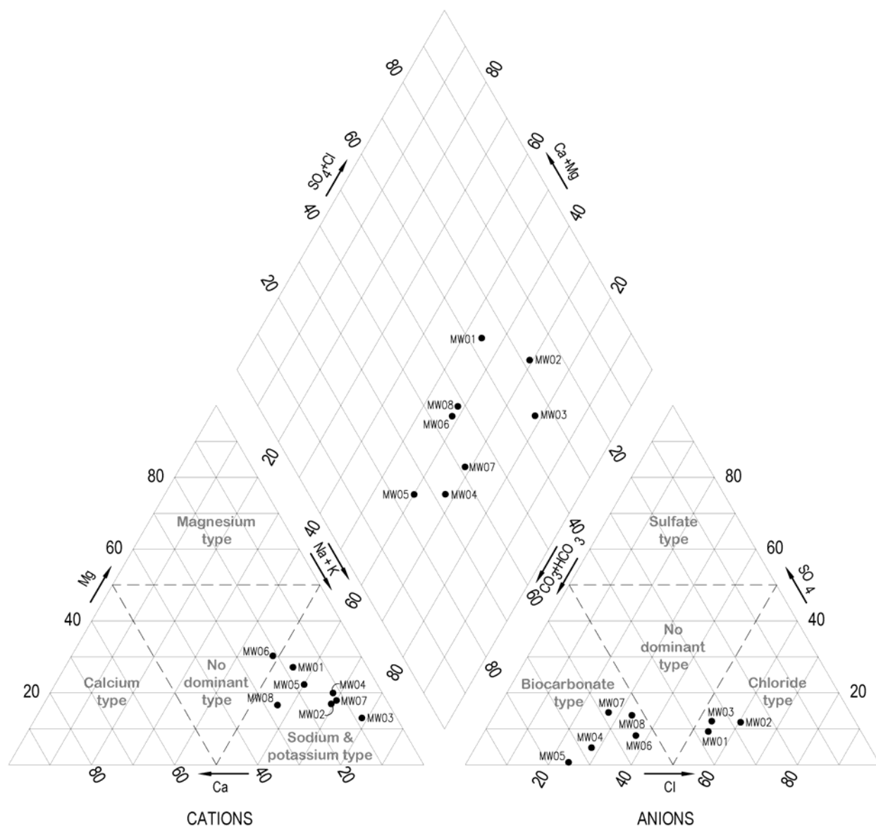
FIGURE 3-2. Example of Piper diagram
