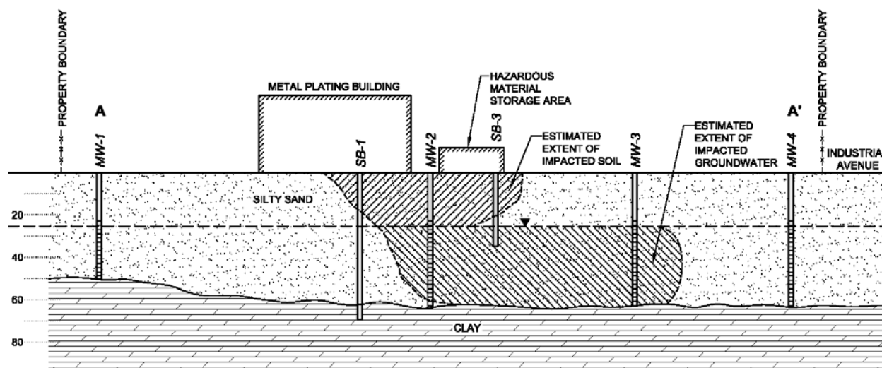
FIGURE 3-1b. Conceptual site model for background analysis, cross sectional view
