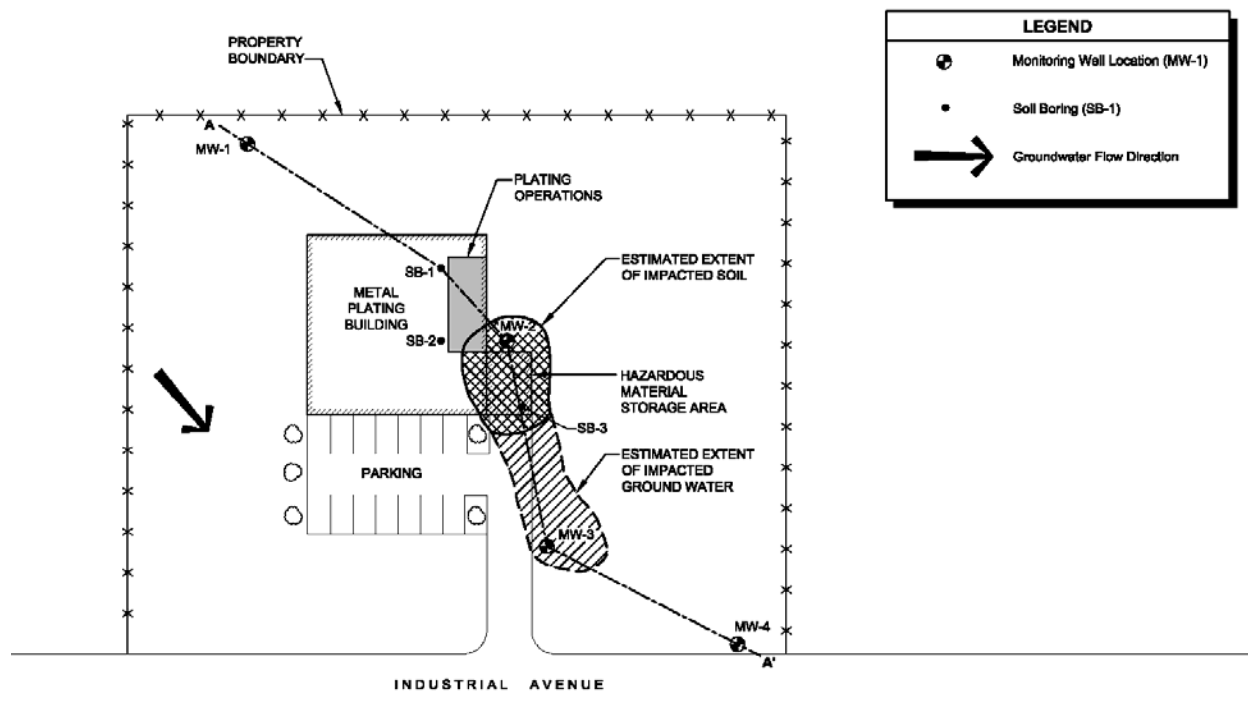
FIGURE 3-1a. Conceptual site model for background analysis, plan view
