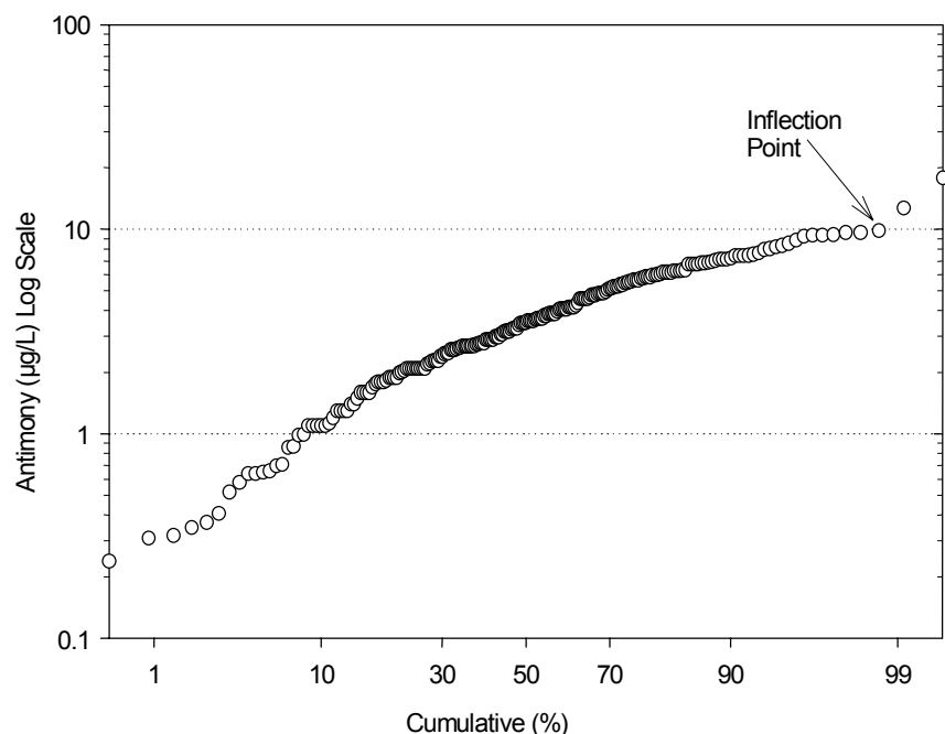
FIGURE 3-5. Example probability plot
