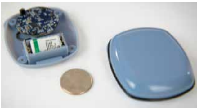
PNNL designed the R&D 100 Award-winning Acoustic Gunshot Detection technology to be easily adapted and affordable. The golf ball-sized sensor contains a Wi-Fi-enabled microcontroller, microphone, and battery.
