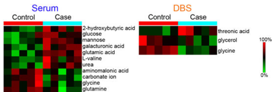
Figure 4. Heatmaps illustrating the polar metabolites found to have statistically significant changes in the patient groups. [Colour figure can be viewed at wileyonlinelibrary.com ]
