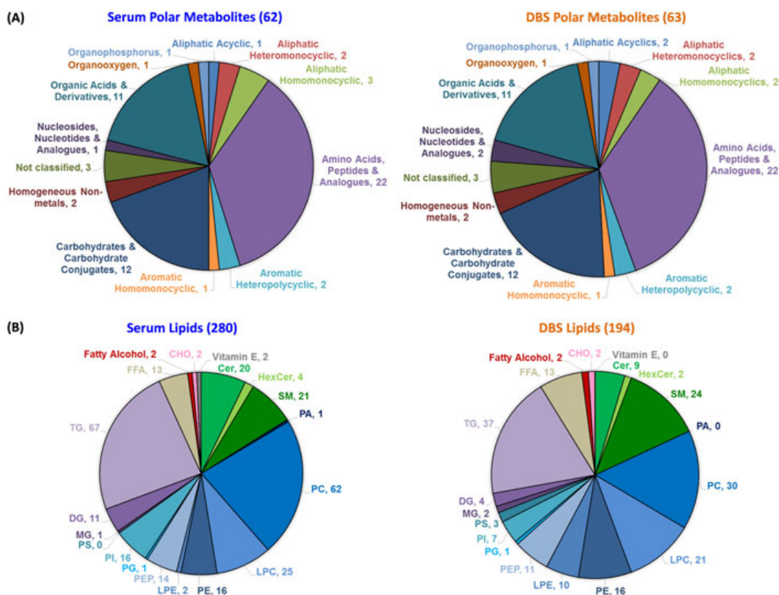
Figure 3. The small molecule distribution of (A) polar metabolites and (B) lipid subclass identifications for the serum and DBS samples. Parentheses show the number of identifications per pie chart. CHO: cholesterol; Cer: ceramide; HexCer: hexosylceramide; SM: sphingomyelin; PA: diacylglycerophosphate; PC: diacylglycerophosphocholine; LPC: monoacylglycerophosphocholine; PE: diacylglycerophosphoethanolamine; LPE: monoacylglycerophosphoethanolamine; PEP: PE plasmalogen; PG: diacylglycerophosphoglycerol; PI: diacylglycerophosphoinositol; PS: diacylglycerophosphoserine; MG: monoacylglycerol; DG: diacylglycerol; TG: triacylglycerol; FFA: free fatty acids. [Colour figure can be viewed at wileyonlinelibrary.com ]
