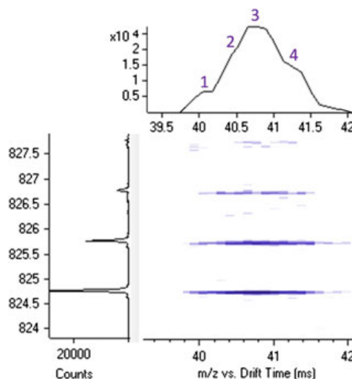
Figure 5. The 1-s nested IMS-MS spectra for (TG(48:0) + NH 4 ) + extracted at LC elution time 71.8 min. Only one LC peak was observed for TG(48:0) but four IMS peaks were present indicating the co-eluting isomers. [Colour figure can be viewed at wileyonlinelibrary.com ]
