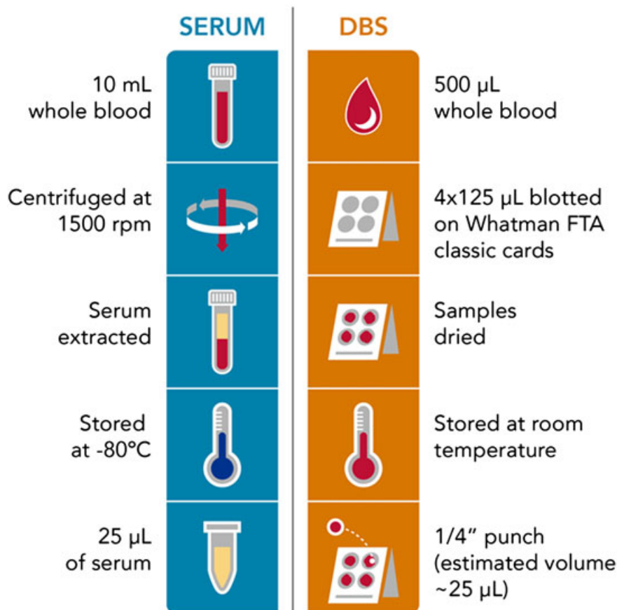
Figure 1. Schematic illustrating the differences in sample collection and preparation for serum and DBS samples. [Colour figure can be viewed at wileyonlinelibrary.com ]
