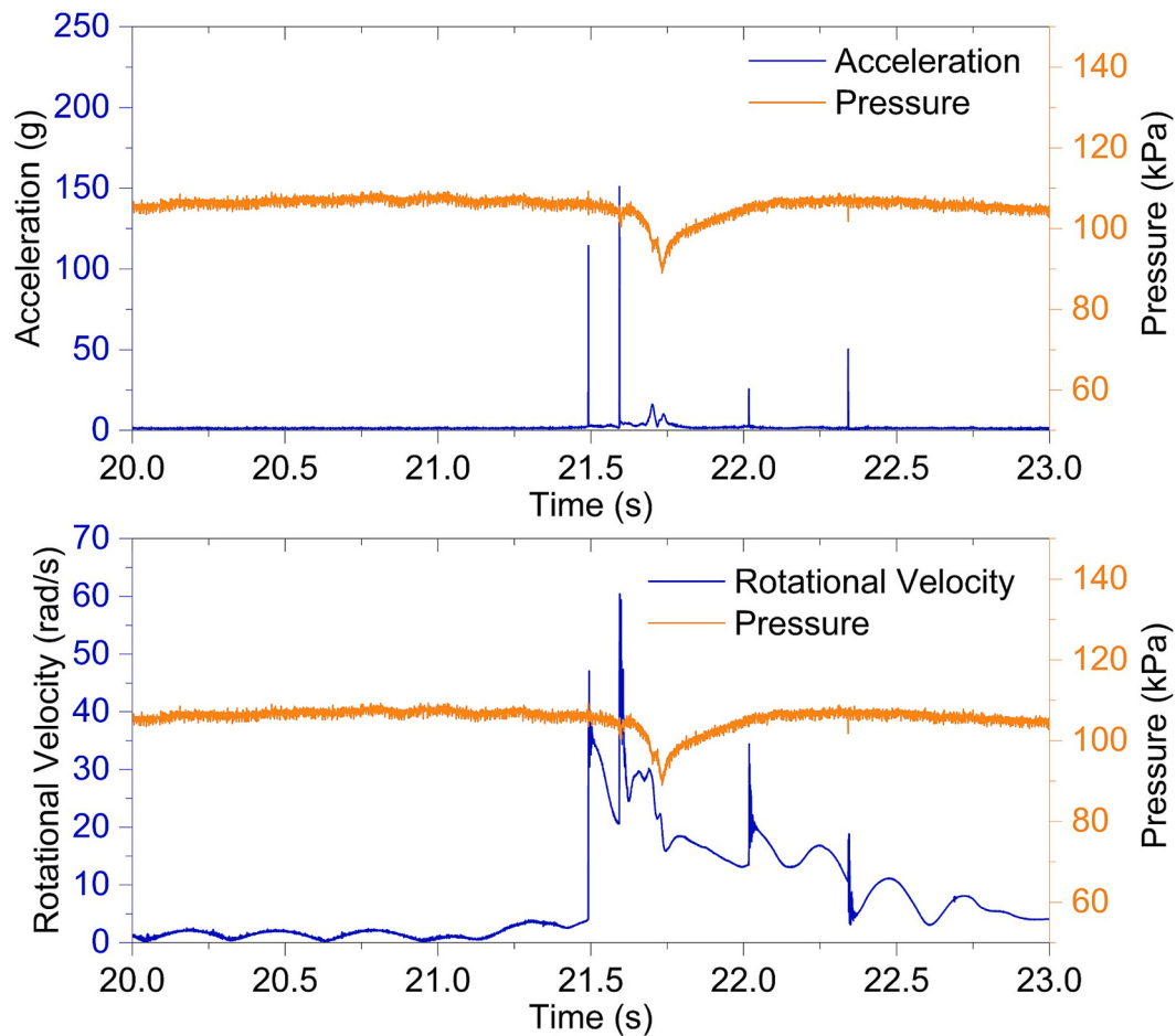
Fig. 8. Example of SF Mini data collected from a scaled model of a Kaplan turbine in a test rig. The data are compared with CFD simulations to validate flow characteristics and assess hydraulic performance.
