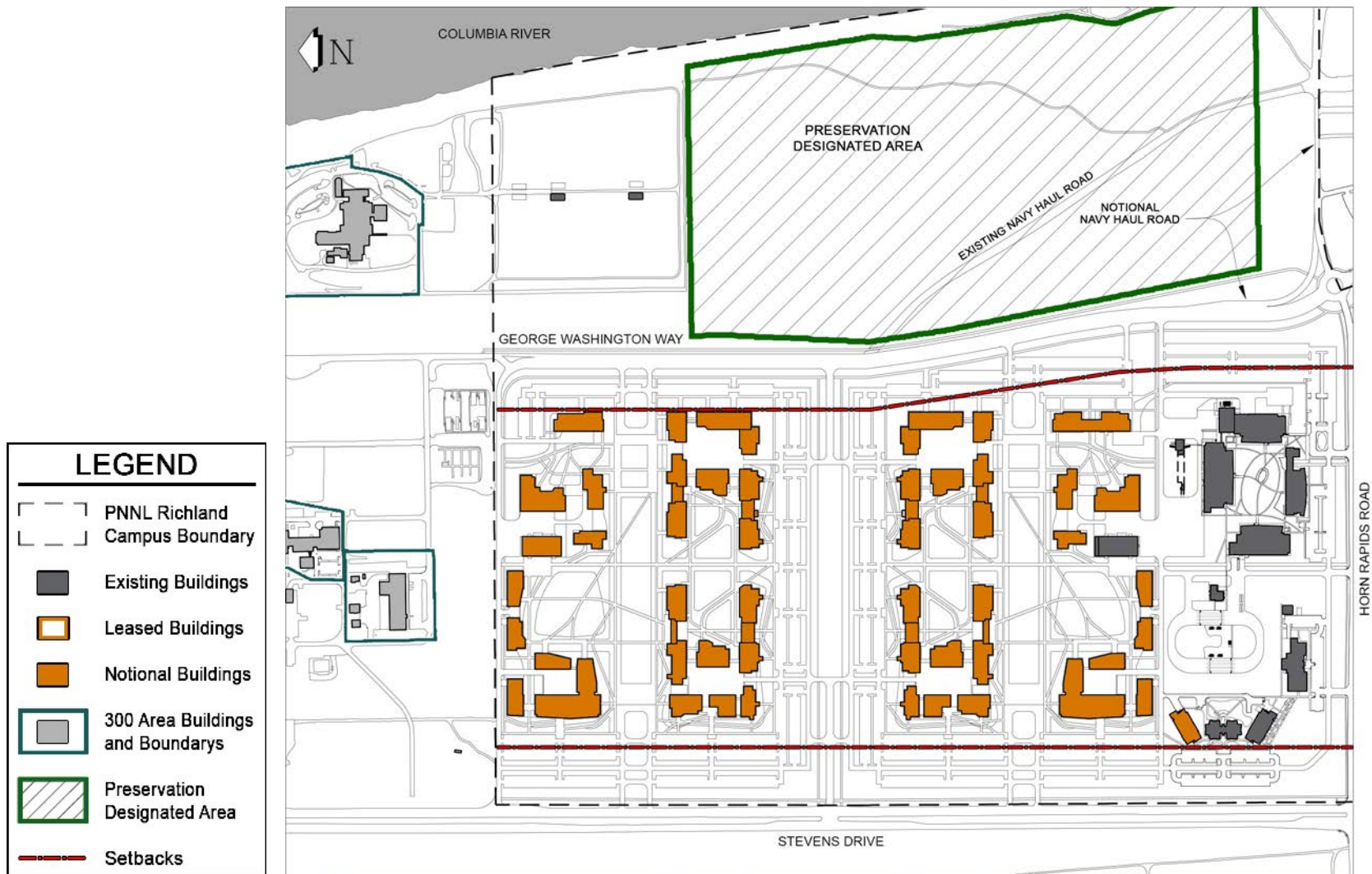
Figure 4.10. Building setbacks
