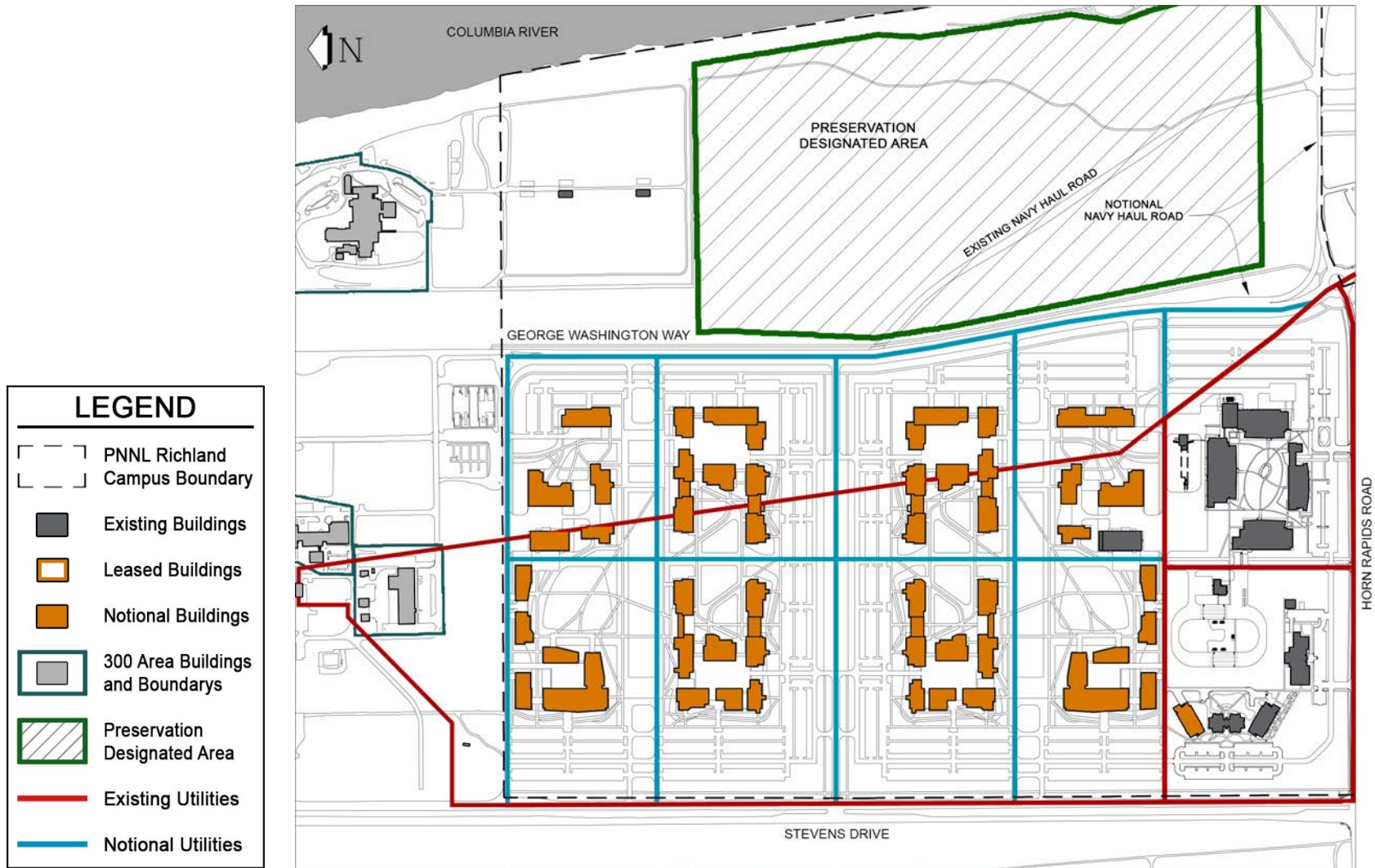
Figure 3.4. Utilities infrastructure and distribution systems corridors
