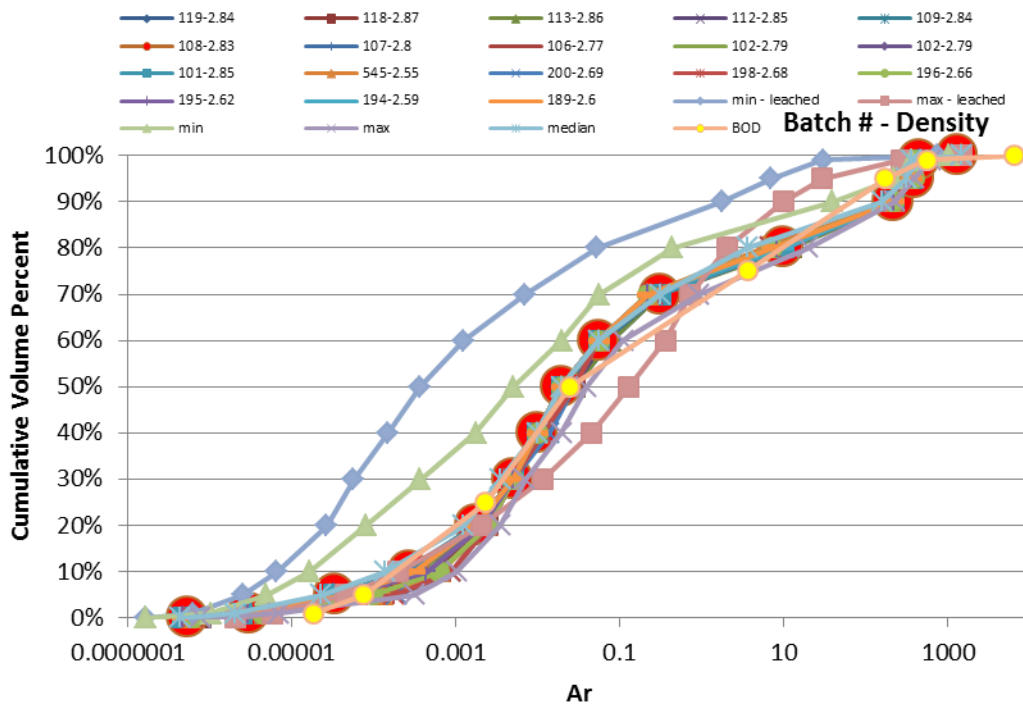
Figure A.17. Selected 80 th to 100 th percentile of the 80 th percentile Ar batch results.
