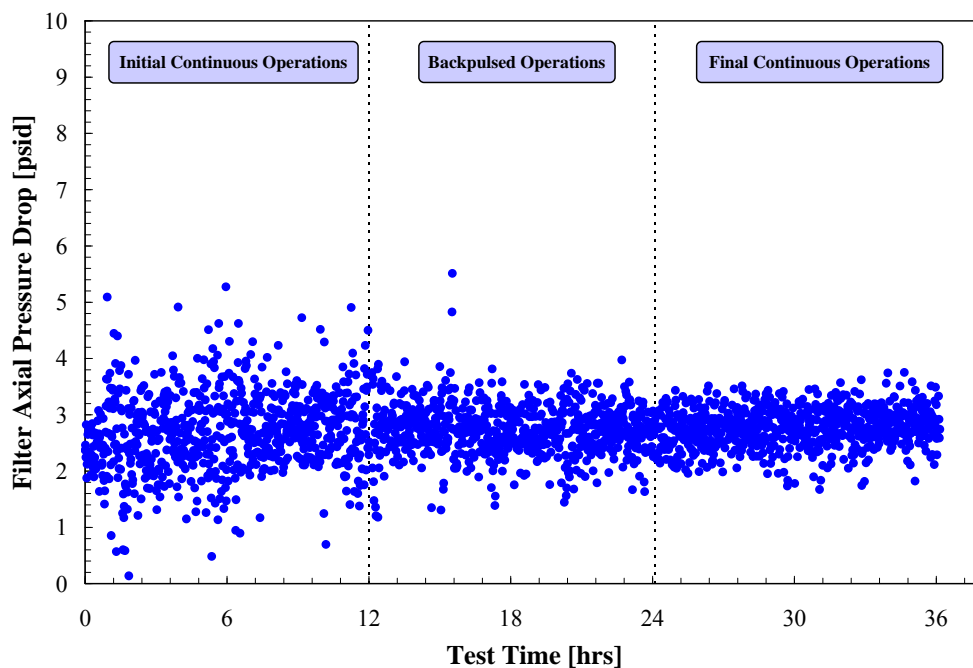
Figure 5.9. CUF Filter APD During Low-Solids Scaling Test #1
