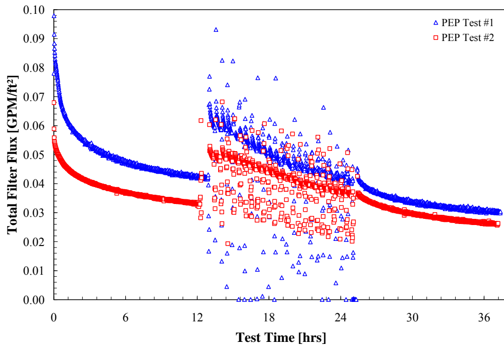
Figure 5.31. Comparison of Total PEP Filter Flux for Low-Solids Scaling Tests #1 and #2. The test time scale for PEP Test #2 has been modified to better align the periods of continuous and backpulsed filtration for CUF and PEP.
