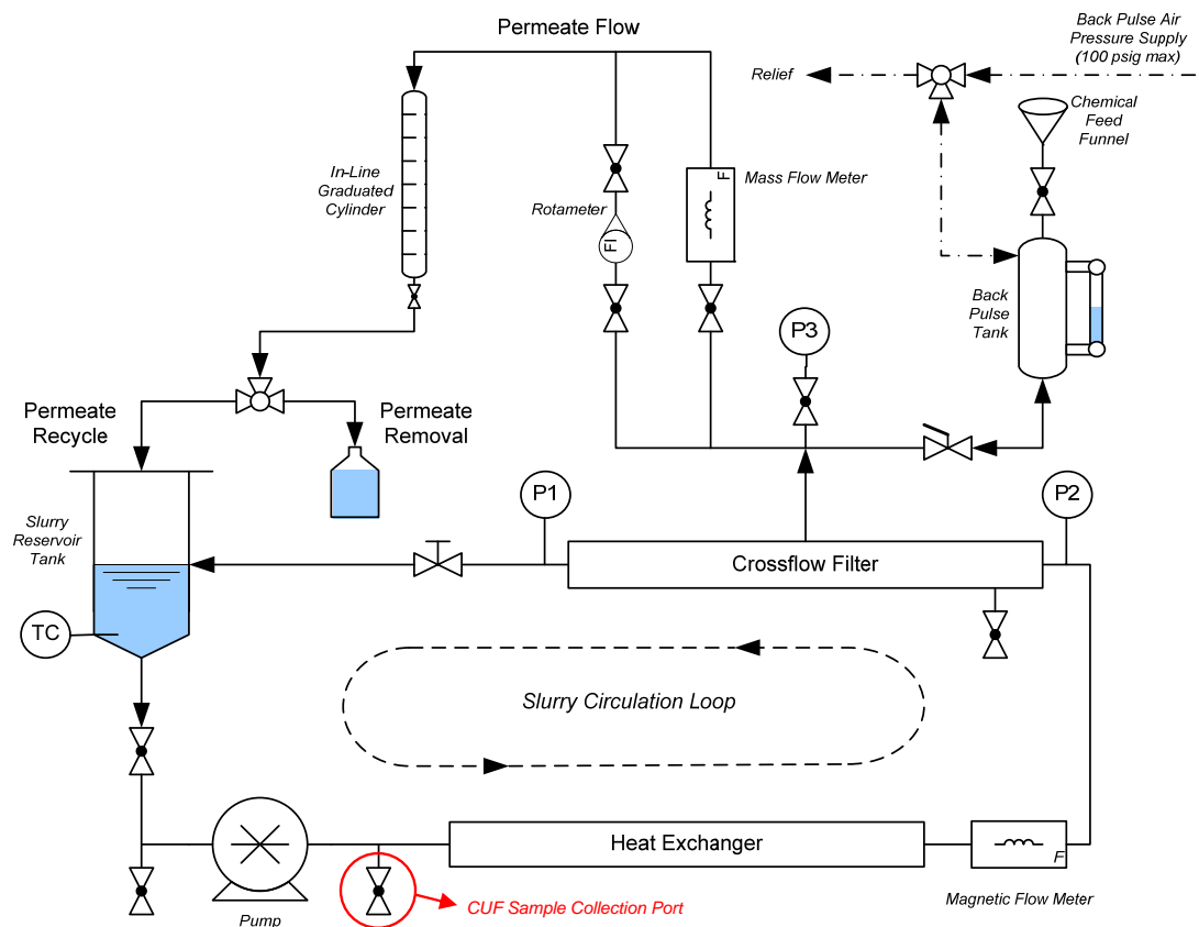
Figure 3.8. CUF Piping Diagram
