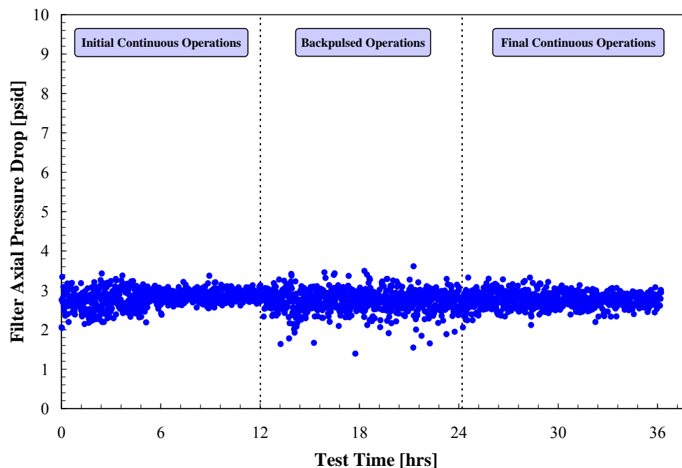
Figure 5.24. CUF Filter APD During Low-Solids Scaling Test #2
