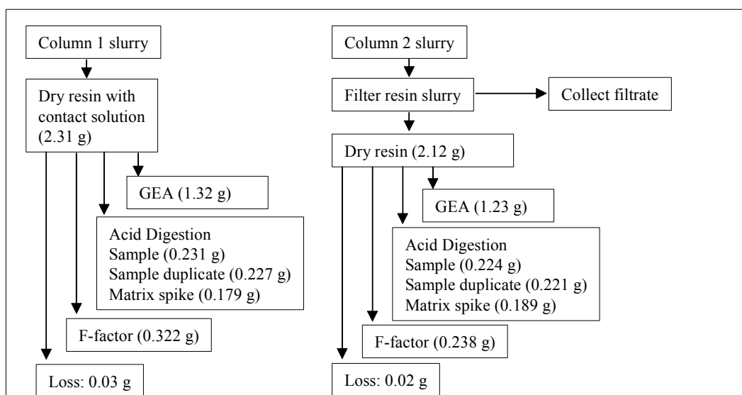
Figure 3.1. Spent-Resin Disposition
