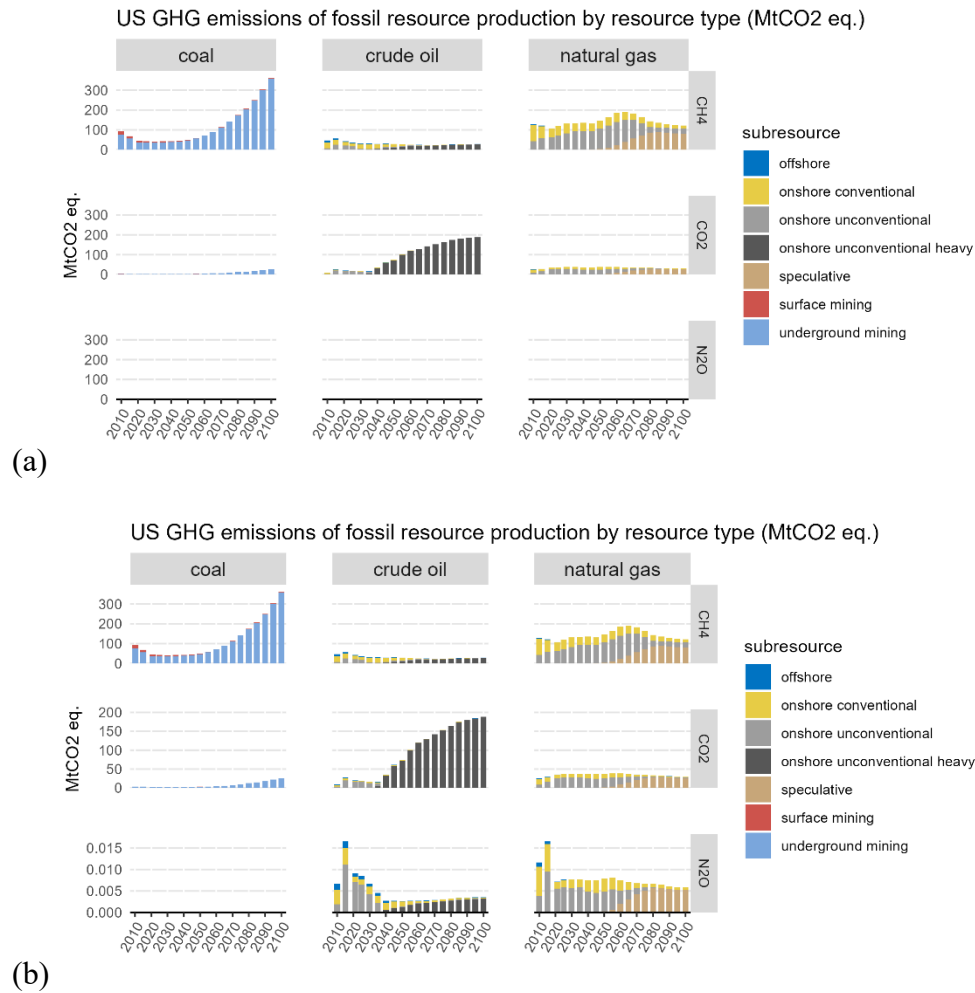
Fig.16 U.S. GHG emissions from fossil resource production by sub-resource in the GCAM-USA-CMP. (a) shows the results in the same y-axis scale; (b) shows different scales of y-axis.
