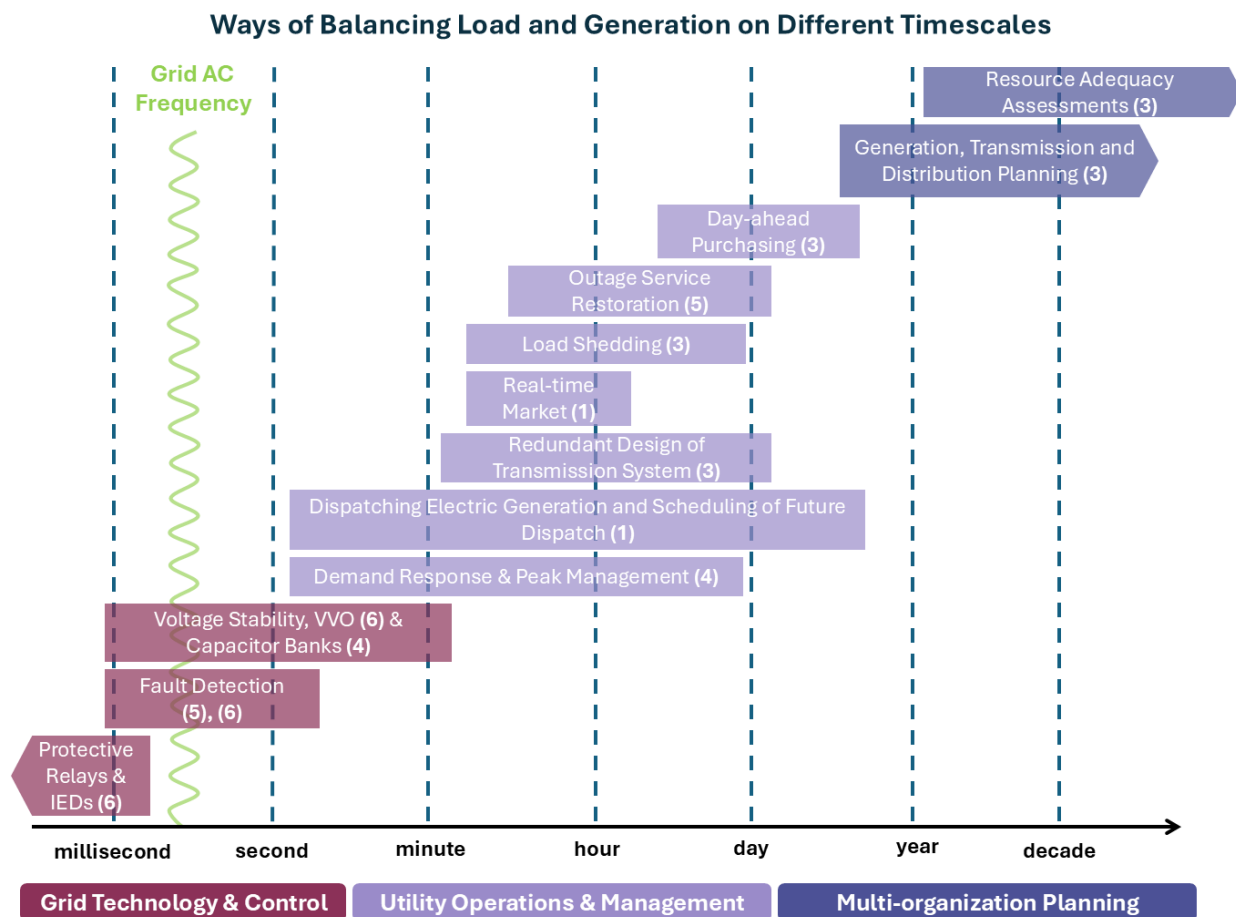
Figure 33: Ways of Balancing Load and Generation on Different Timescales
