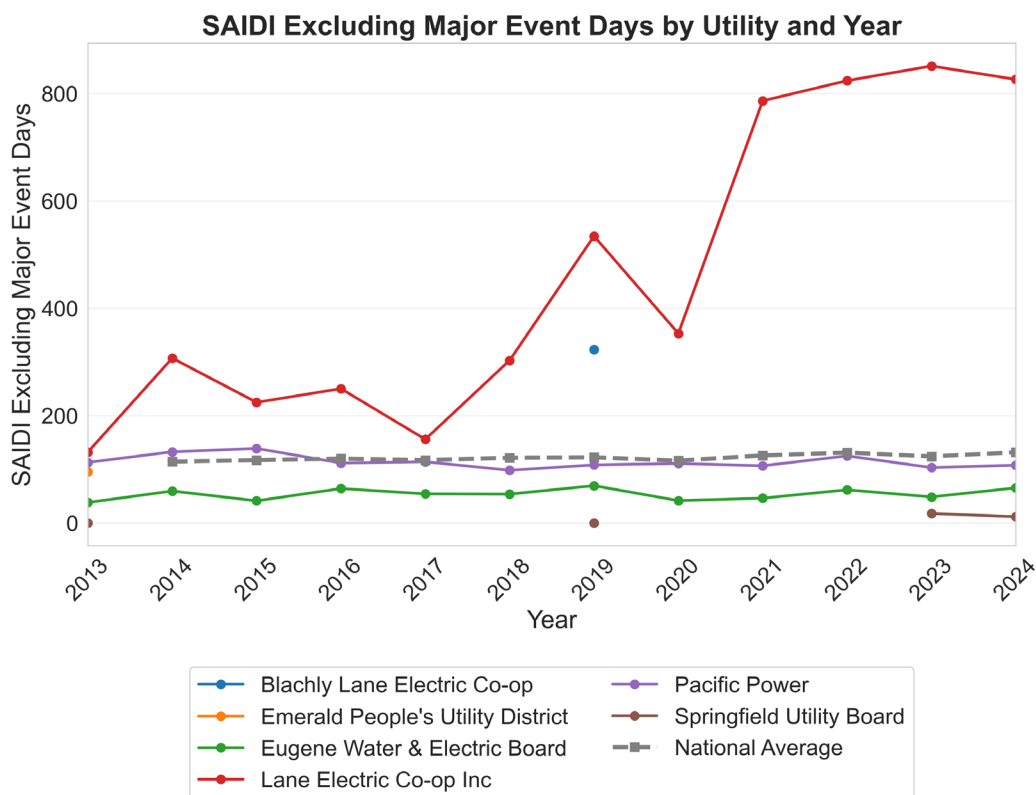
Figure 36: Annual Lane County SAIDI Data Reported to EIA vs National Average
