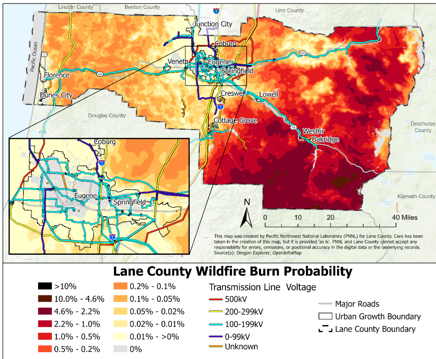
Figure 53: Lane County Wildfire Burn Probability. 1, 2
