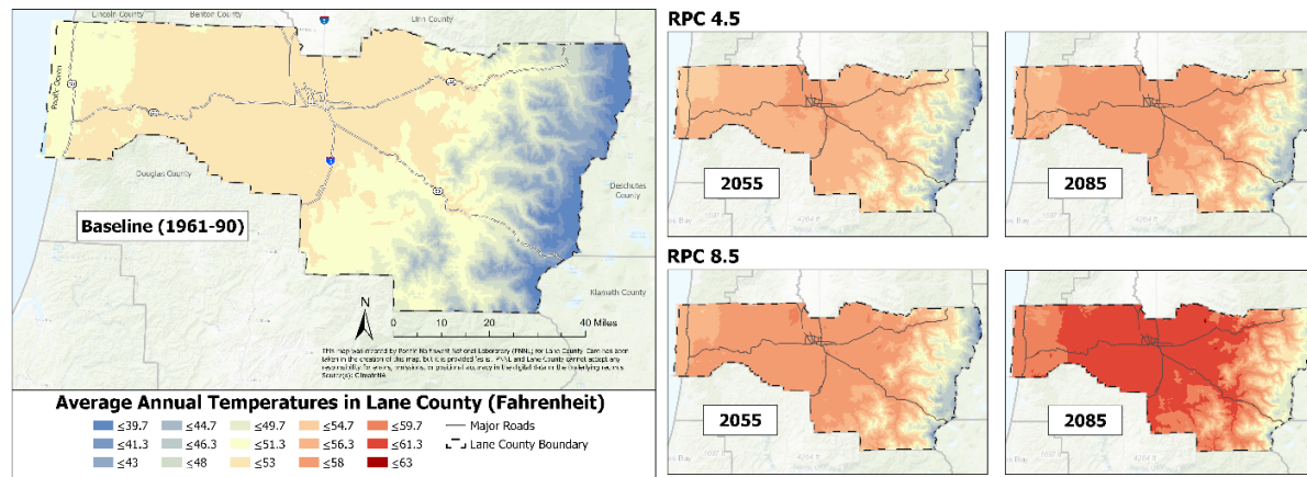
Figure 63: Baseline and Future Projected Mean Annual Temperature Across Lane County Baseline historical timeframe (1961–1990) and two future years (2055 and 2085) each with two different future scenarios: Representative Concentration Pathways (RCP) 4.5, which considers intermediate greenhouse gas reduction success, and RCP 8.5, which represents the business-as-usual projection 2,3
