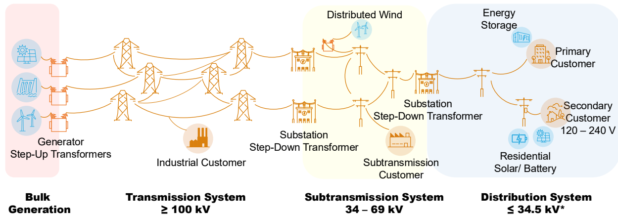
Figure 11: The Electric Grid
