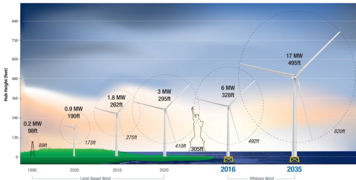
Figure 72: Wind Turbine Capacity, Hub Height, and Rotor Diameter 2
