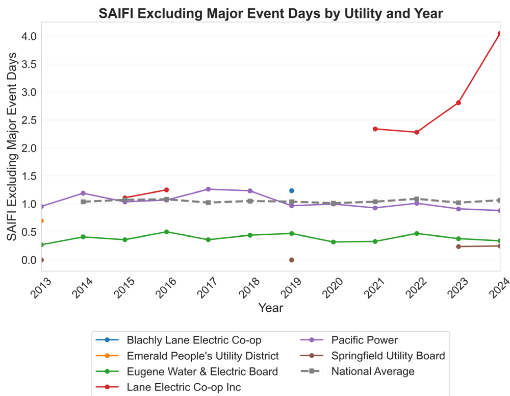
Figure 37: Annual Lane County SAIFI Data Reported to EIA vs National Average
