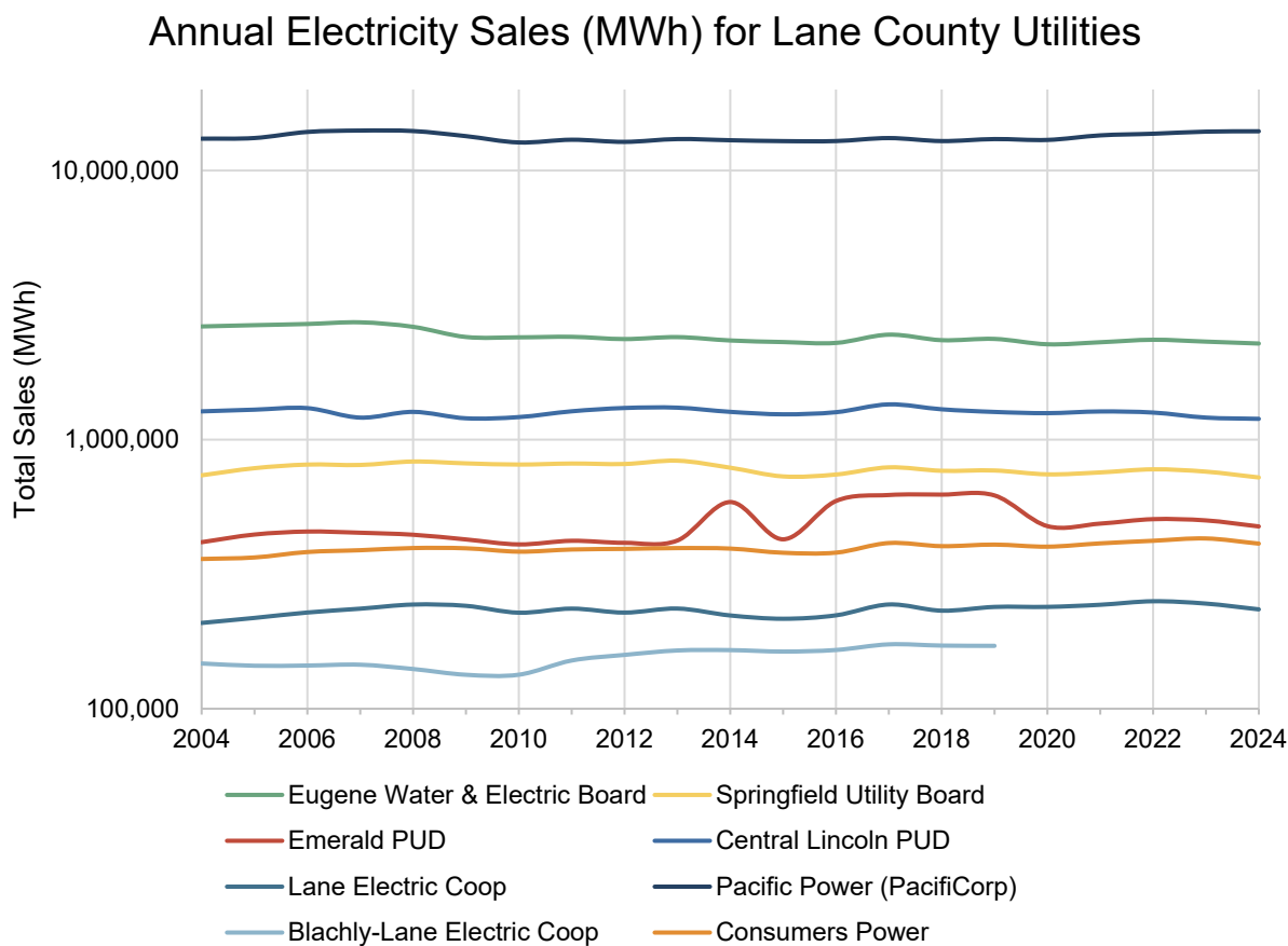
Figure 44: Annual Electricity Sales for Lane County Utilities, 2004–2024 1
