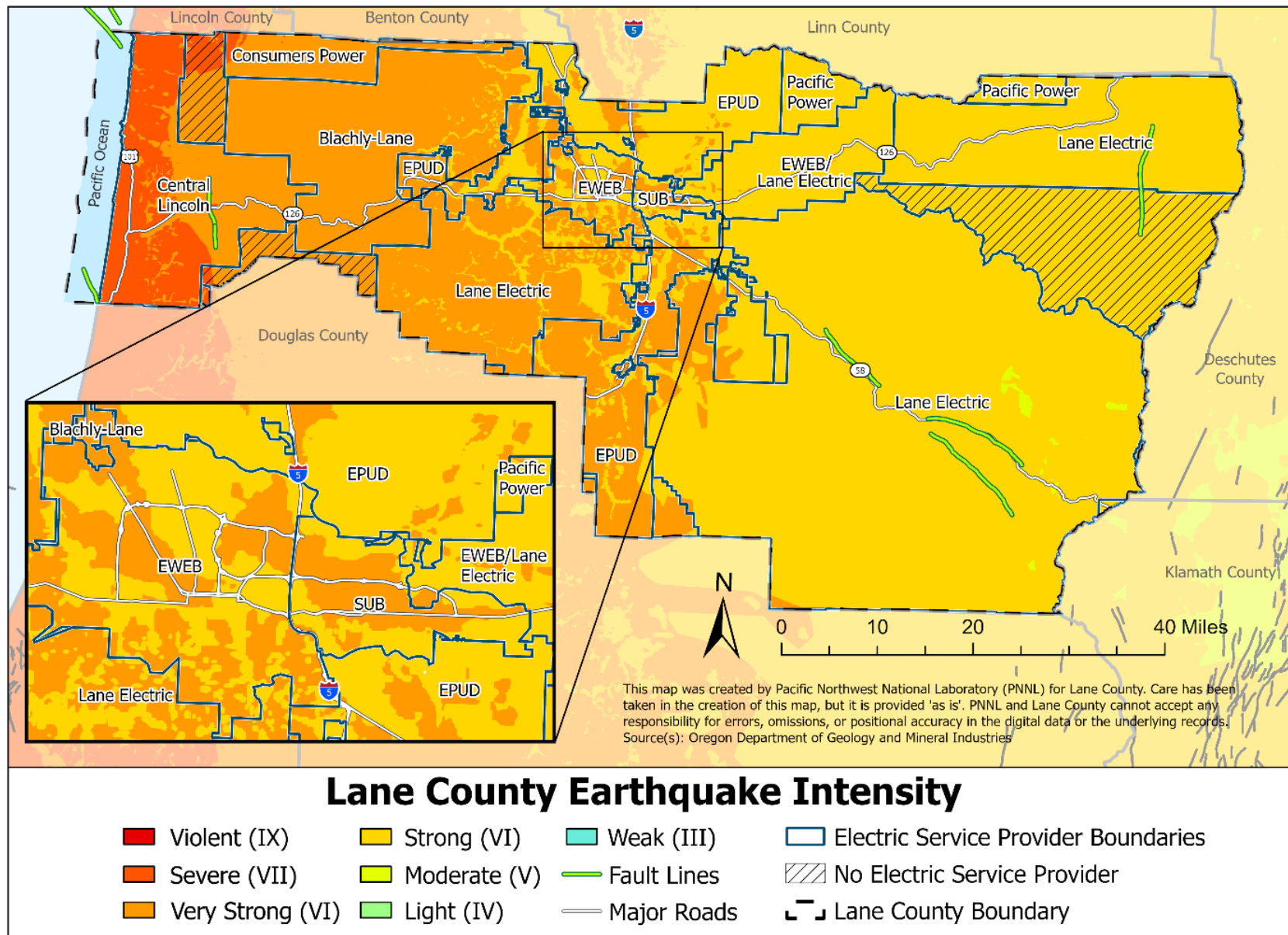
Figure 59: Estimated Severity of Earthquake Amplification (Ground-Shaking) in Lane County 1
