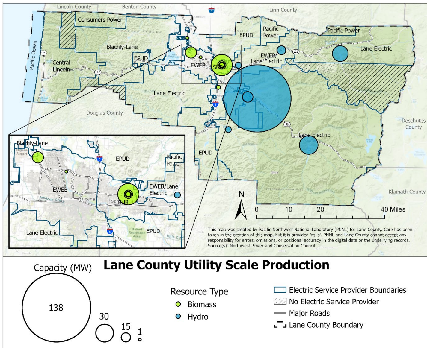
Figure 27: Grid-connected biomass (green) and hydro (blue) power production in Lane County scaled by MW capacity. 1
