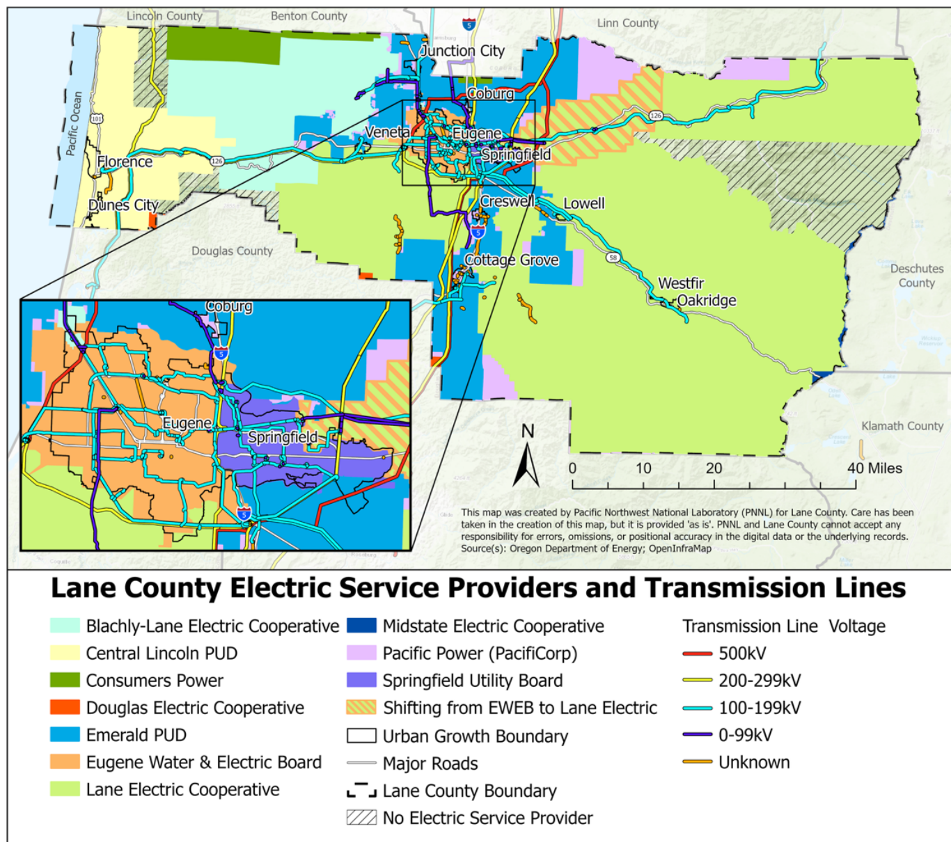
Figure 39: Map of Utility Service Territories and Transmission Infrastructure for Lane County 1,2
