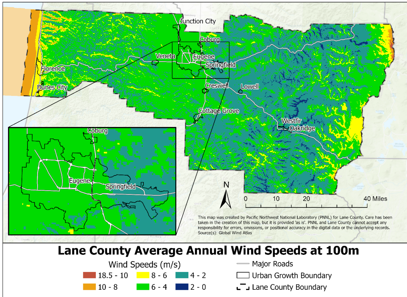
Figure 73: Annual Average Wind Speeds at 100m in Lane County, Oregon 1
