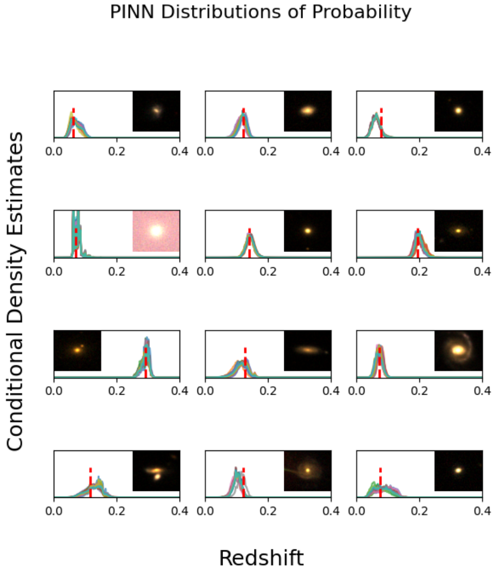
Figure 12: A selection of PINN model output conditional density estimates plot over 20 random rotations and background re-samplings of the shown galaxy. In comparison to the baseline model, our PINN model is less variant, but it is very similar to the augmentation model, which is much cheaper to train.
