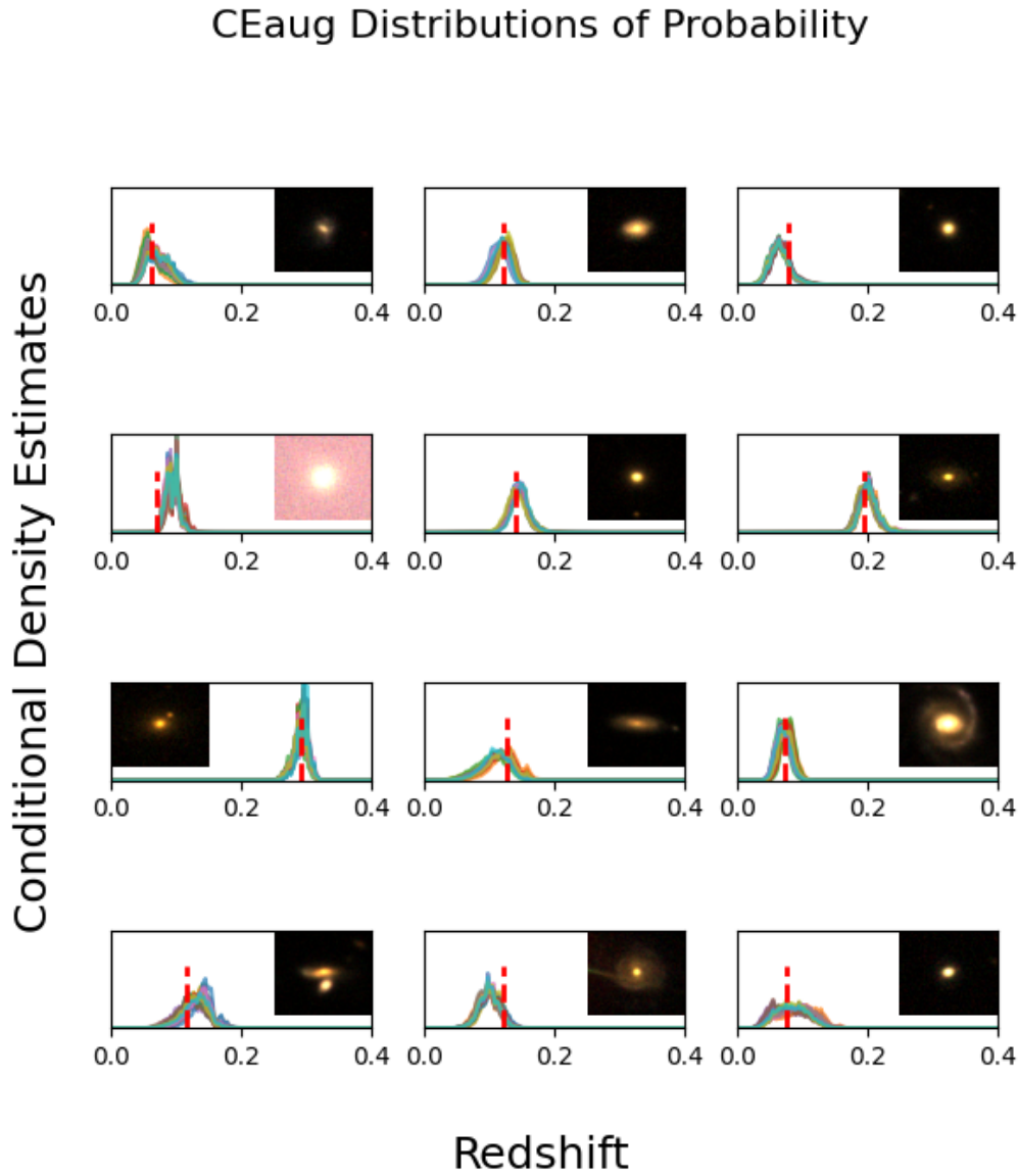
Figure 11: A selection of Baseline w/ Augmentation model output conditional density estimates plot over 20 random rotations and background re-samplings of the shown galaxy. In comparison the baseline model, the distributions are markedly less variant. This is the precise effect our invariance to rotation and background samples seeks to achieve, so it would appear these terms are more-or-less satisfied through augmentation alone.
