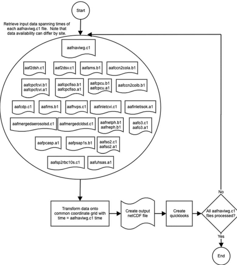
Figure 2. Detailed process flow diagram of AAFMERGED VAP.
