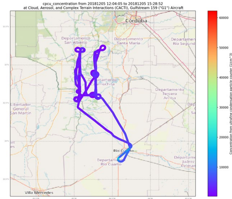
Figure 4. Concentration from ultrafine condensation particle counter from CACTI flight initiated on December 5, 2018 at 15:28:52 GMT.
