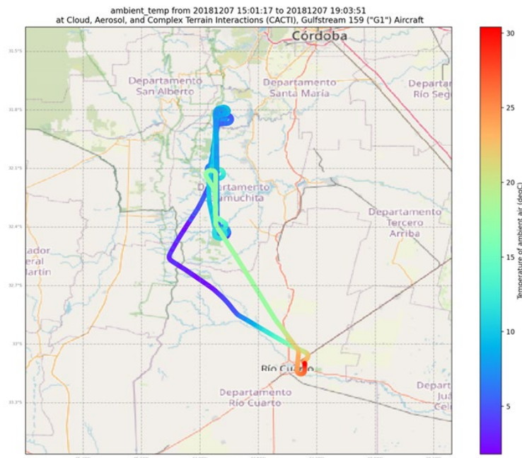
Figure 3. Ambient temperature from CACTI on flight initiated on December 7, 2018 at 15:01:17 GMT.
