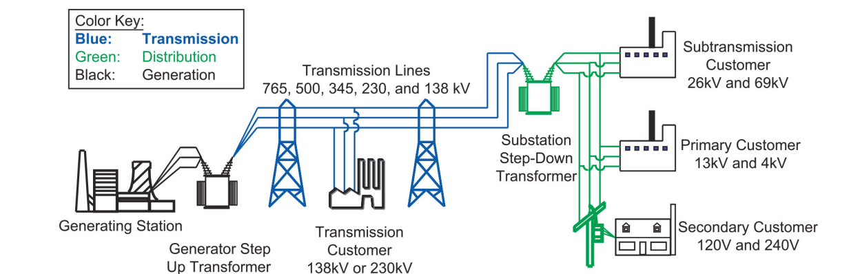
Figure 9. High-voltage electricity transmission corridor that feeds into distribution feeders for delivery to customers. 17
