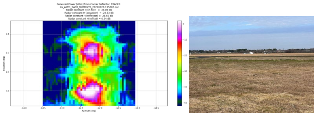
Figure 36. a) The challenges of the SACR corner reflector calibration caused by the “mirror-like” effects from the two runways directly between the SACR and the trihedral. b) A look at the corner reflector from the SACR roof. The two runways produce obvious multipath effects seen in the results.
