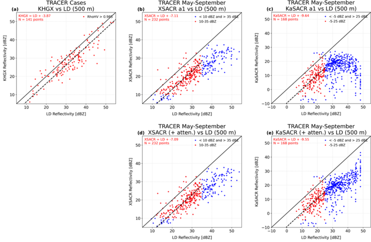
Figure 17. Reflectivity cross-comparisons between the ARM Laser Disdrometer Quantities VAP (LDQUANTS, at x-axis) and radars at y-axis: a) KHGX, b) XSACR, and c) KaSACR, respectively. d-e) Same plots as b and c, but with hydrometeor attenuation corrections.
