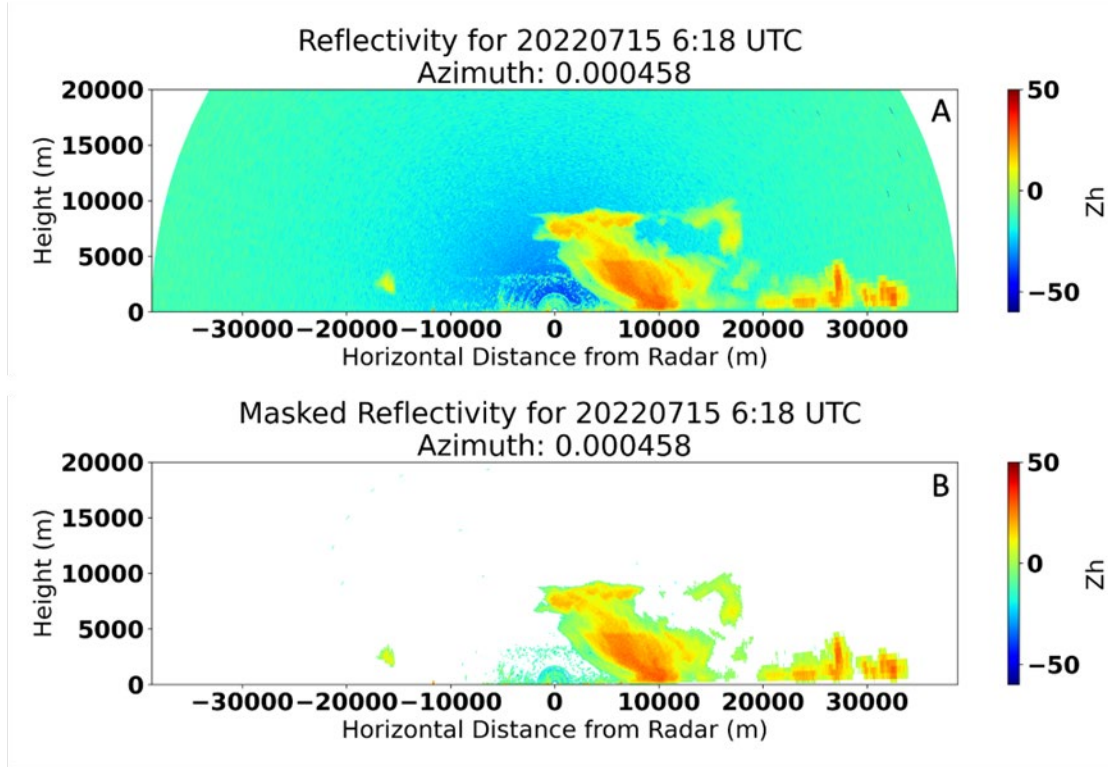
Figure 20. a) Unmasked XSACR reflectivity. b) The same data with the censor mask applied.
