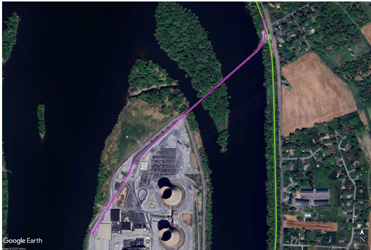
Figure 8. Aerial View of the Three Mile Island Onsite Rail Spur
