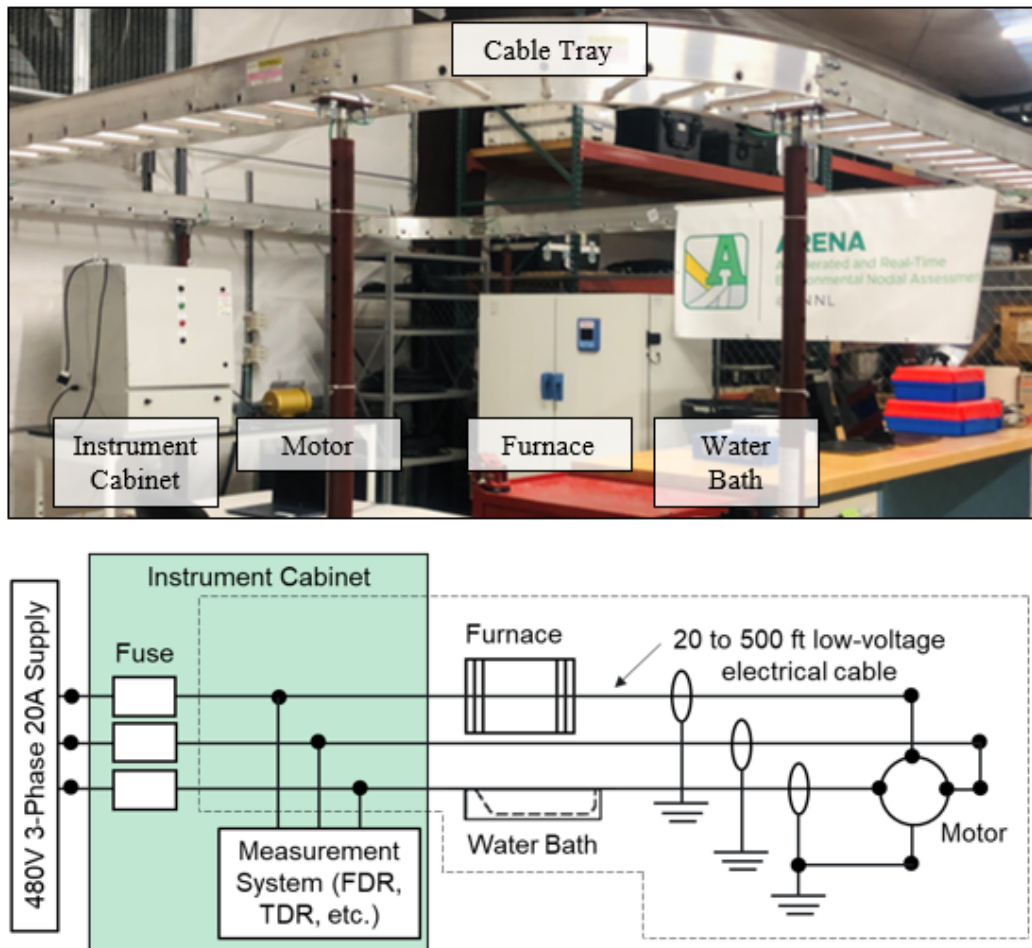
Figure 1-1. The ARENA test bed (top) digital image and (bottom) schematic (Glass et al. 2023).
