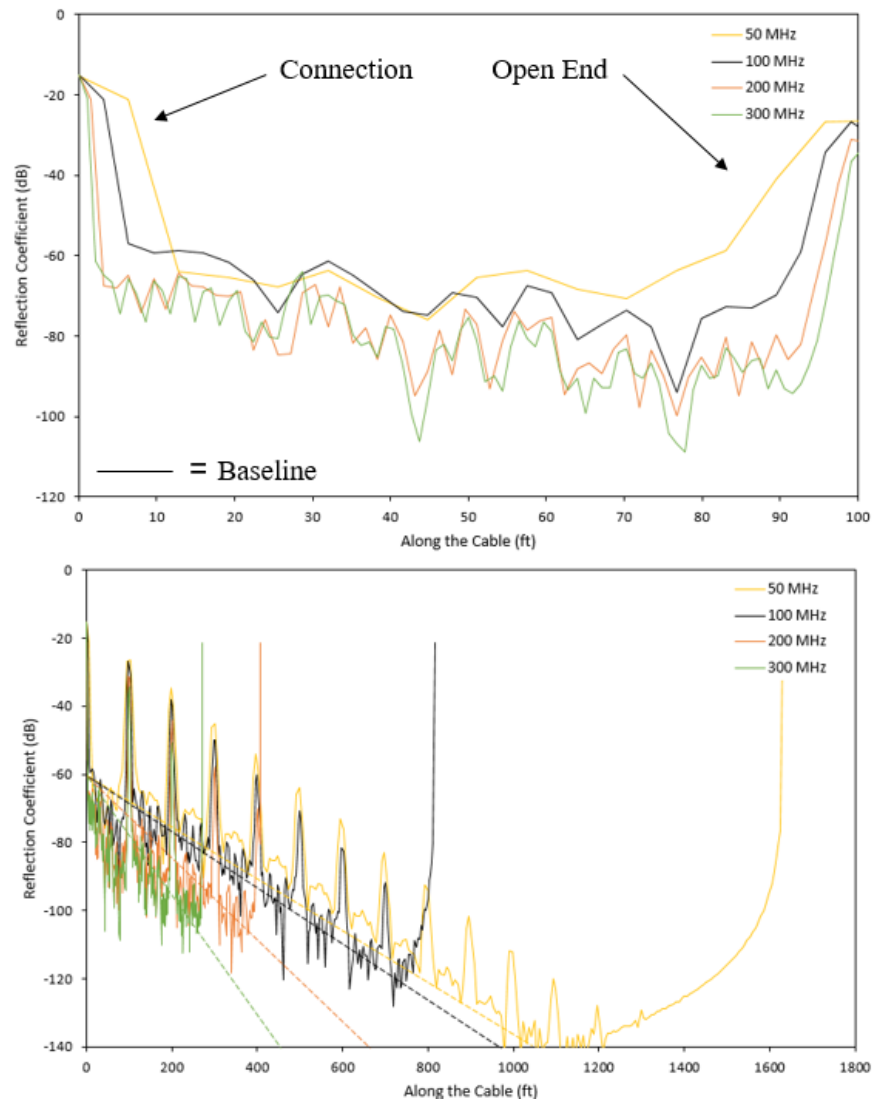
Figure 2-9. Effect of bandwidth on the electrical cable digital twin response demonstrating (top) spatial resolution and (bottom) propagated length and line loss. Baseline refers to the response of the baseline digital twin as discussed in Section 2.3.1.4.
