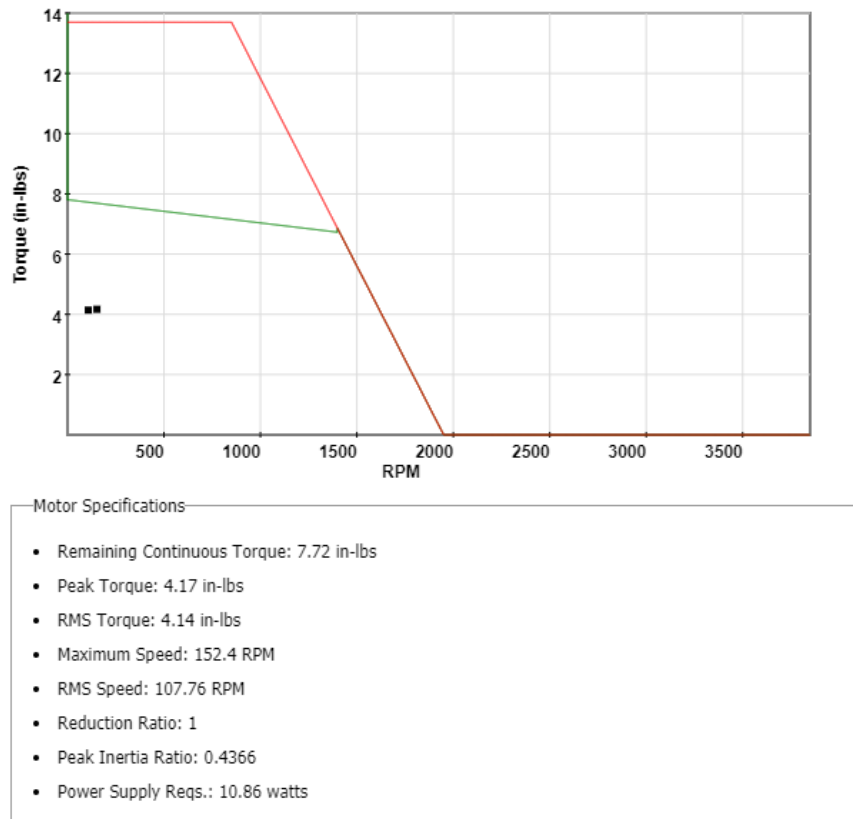
Figure 8: Motor Specifications for Tolomatic ERD Actuator
