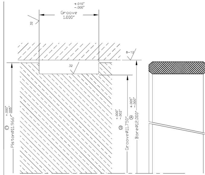
Figure 11: Wear Band Drawing - AHPS C-12686WB
