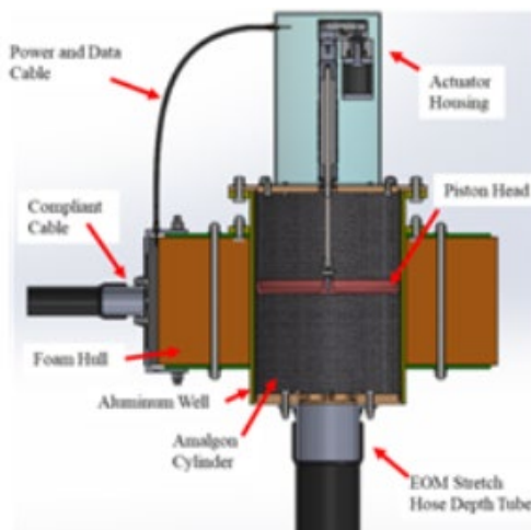
Figure 3: Triton WEC
