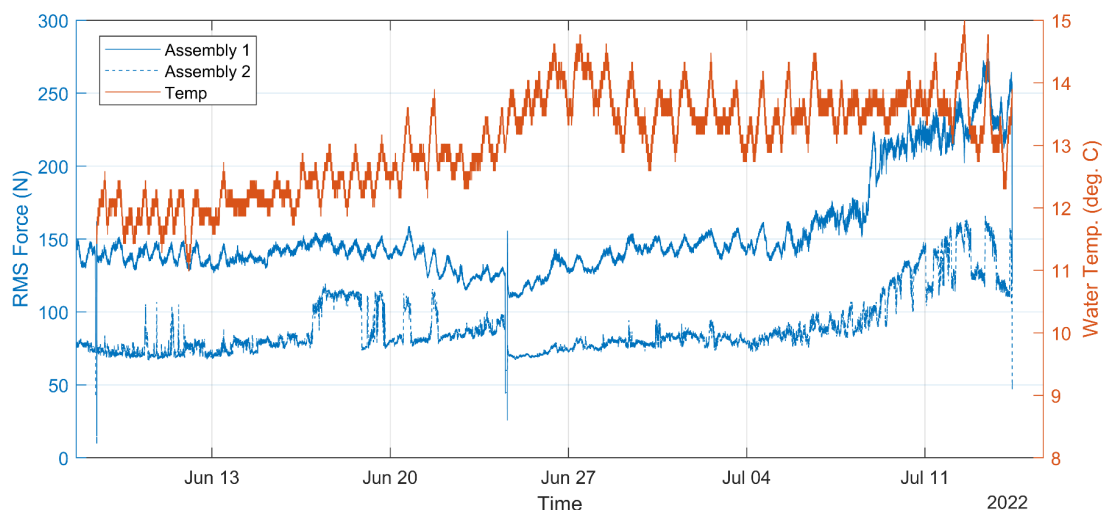
Figure 16: Moving RMS-filtered load cell force with a 100 s filtering window and tank water temperature for partial months 3 and 4 of core testing
