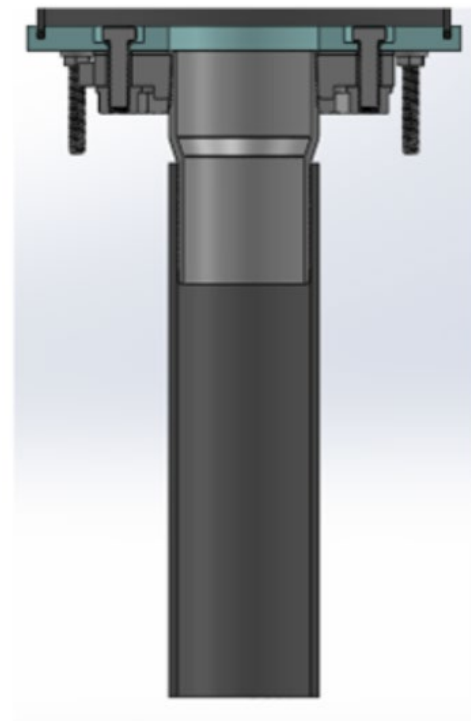
Figure 14: Depth Tube and Flange
