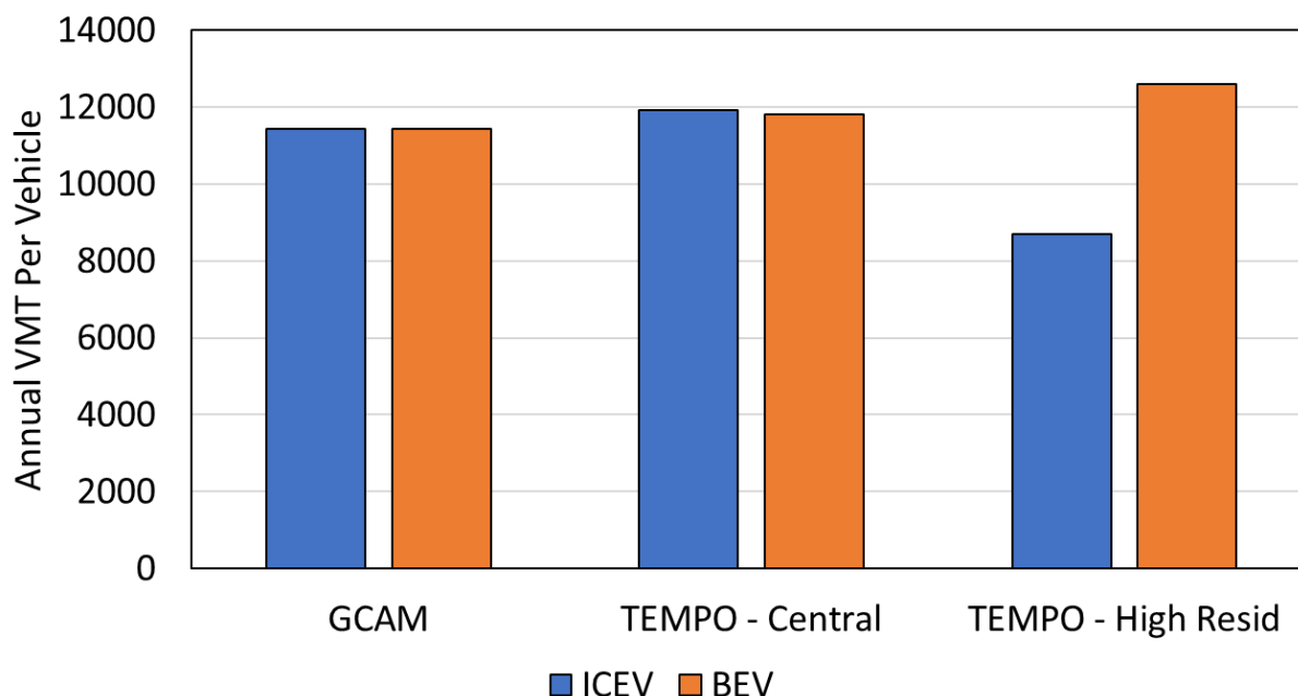
Figure 33. LDV VMT per vehicle by powertrain, model, and scenario, 2050
