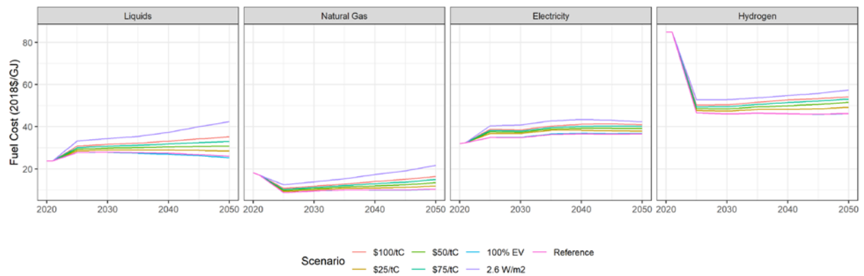
Figure A-4. Fuel cost assumptions
