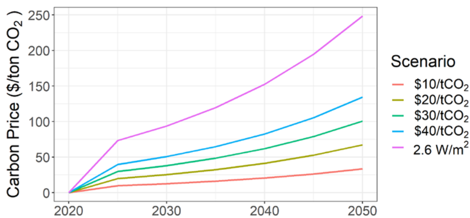
Figure 16. Carbon price trajectories (dollars per metric ton of CO 2 )
