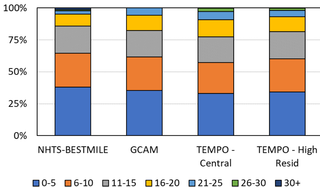
Figure 32. LDV share of VMT by vehicle age, 2050
