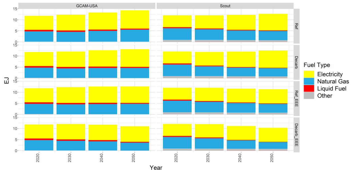
Figure 38. Residential building energy consumption by fuel, year, model, and scenario, 2020–2050 (GCAM-USA and Scout)
