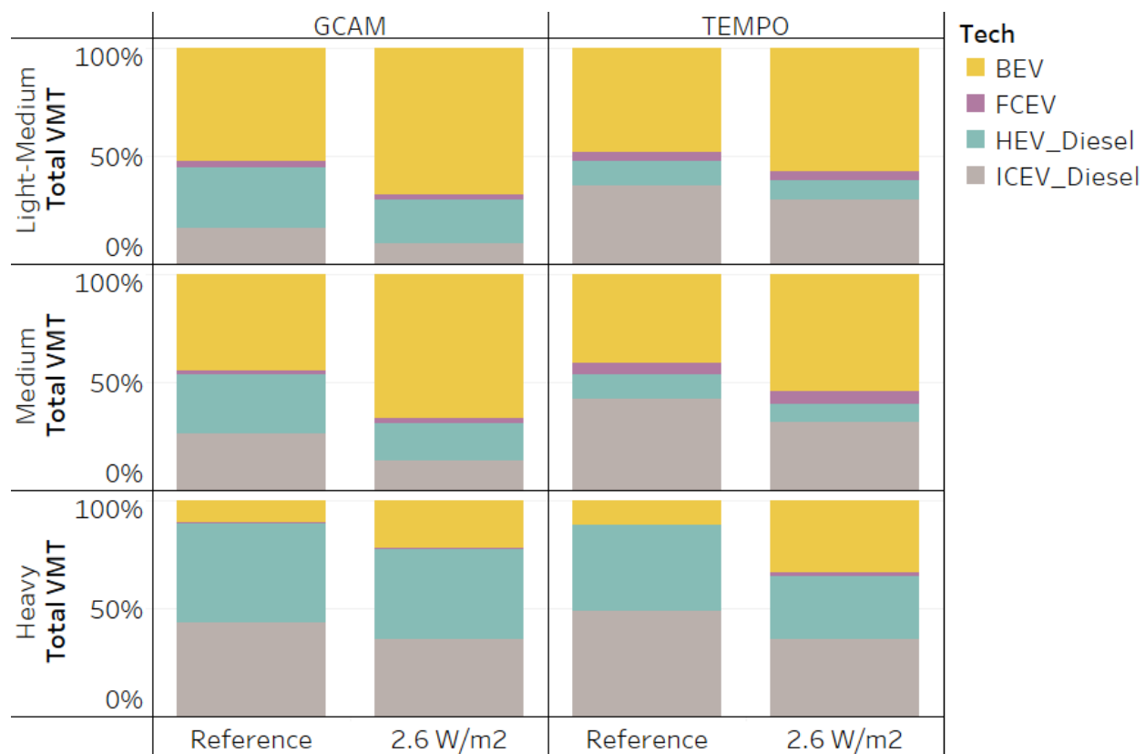
Figure 29. VMT share by technology, light-medium, medium and heavy trucks in the Reference and 2.6 W/m² scenarios, 2050
