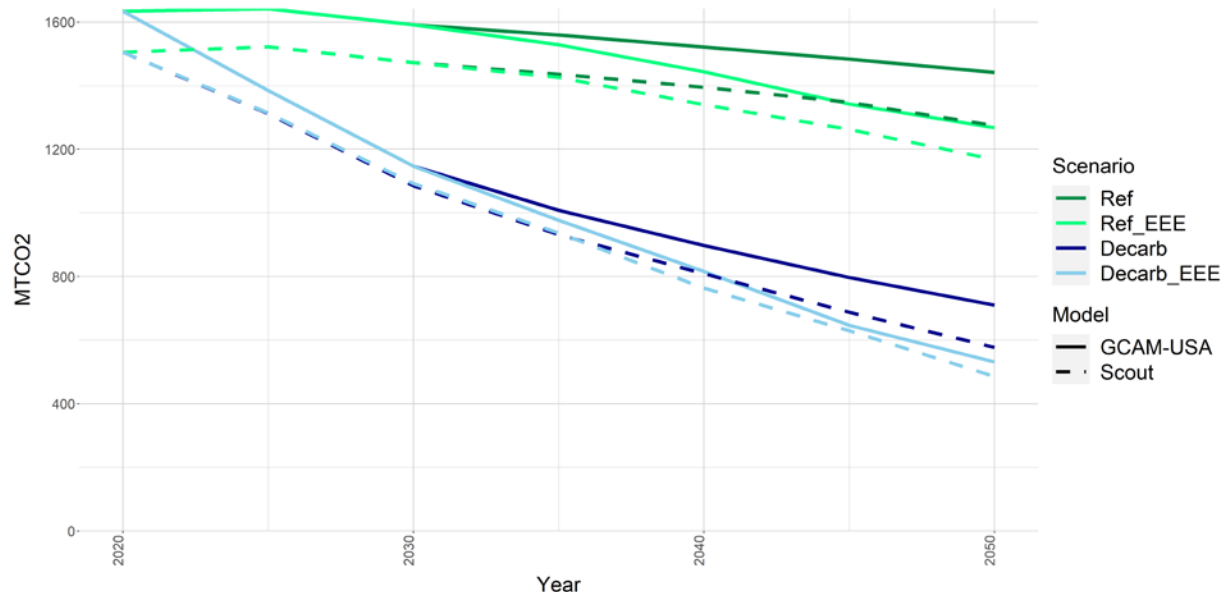
Figure 36. Total building CO 2 emissions by model and scenario, 2020–2050 (GCAM-USA and Scout)
