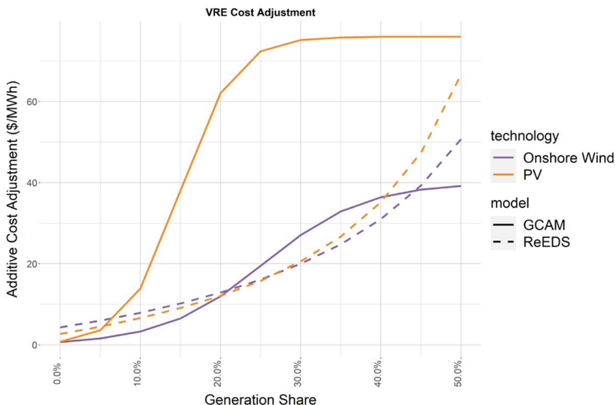
Figure 14. Comparison of VRE cost adjustment approaches
