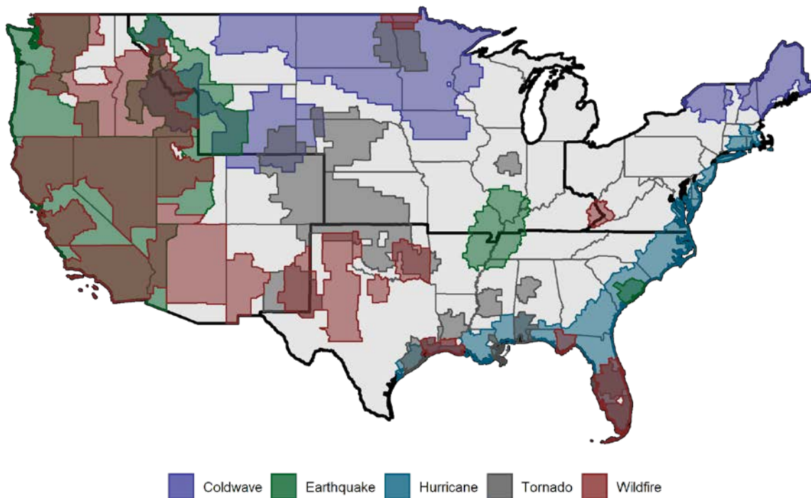
Figure 2. Map of select hazards. Colors denote counties in the top 10% highest occurrence frequency for a given hazard.
