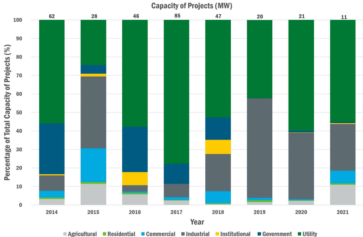
Figure 17. Distributed wind end-use customer types by capacity of projects, 2014–2021
