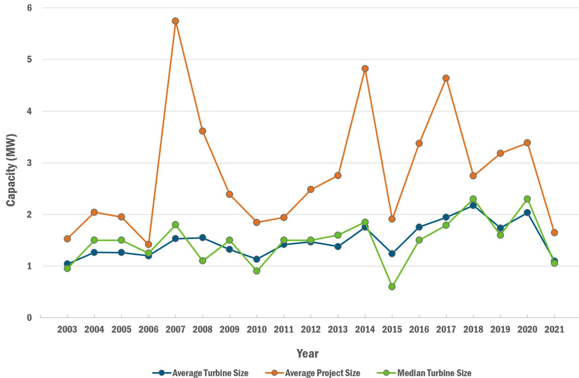
Figure 20. Average size of turbines greater than 100 kW in distributed wind projects and average size of those projects, 2003–2021
