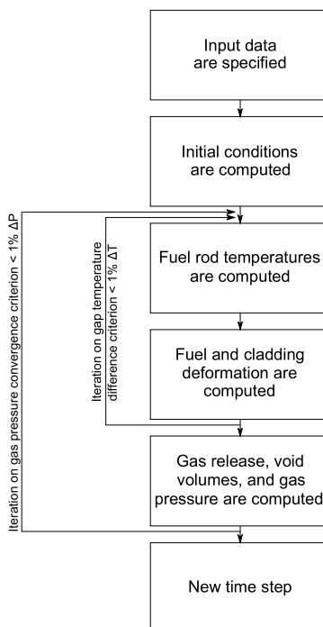
Figure 2-1. Simplified FAST steady-state flowchart
