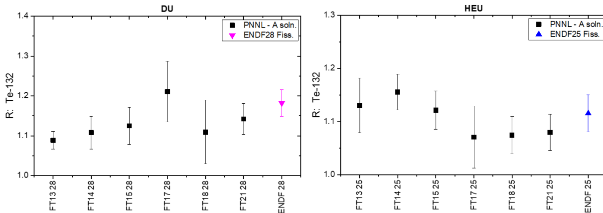
Figure 6.9. Tellurium-132 R-values for DU and HEU samples irradiated on the Flattop critical assembly compared to previous R-value campaigns and ENDF ( R \pm 1\sigma ).
