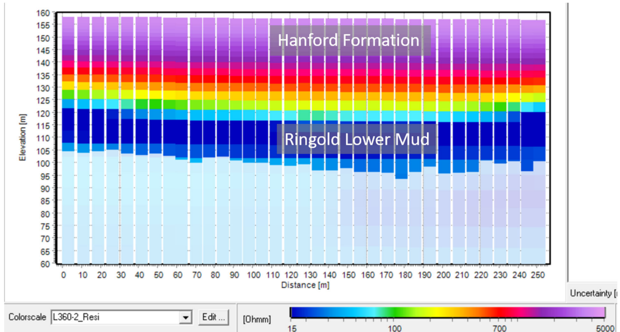
Figure 8. Preliminary tTEM data collected between TEDF and well 699-41-35 (FIO).
