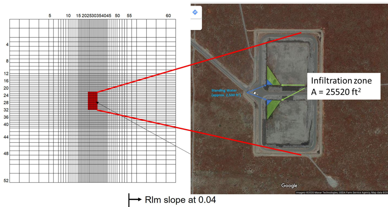
Figure 1. Infiltration simulation grid where the simulated infiltration areas at two flow rates are shown in blue and green, and the Ringold Lower Mud (RLM) is shown to slope to the east (flow and transport simulations courtesy of Matt Tonkin) [For Information Only (FIO)].
