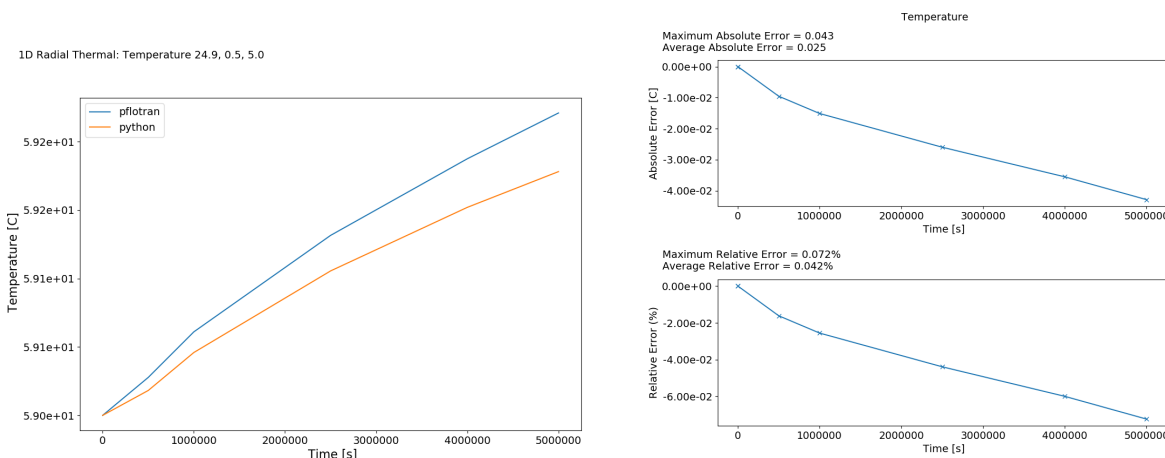
Figure 2-4 Left: Analytical (Python) vs numerical (PFLOTRAN) solution at 24.9 m. Right: absolute and relative error in the numerical solution
