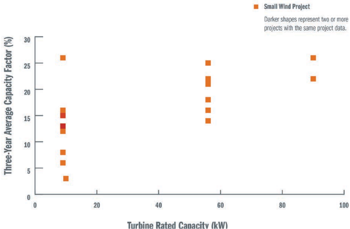
Figure 14. NYSEERDA small wind capacity factors
