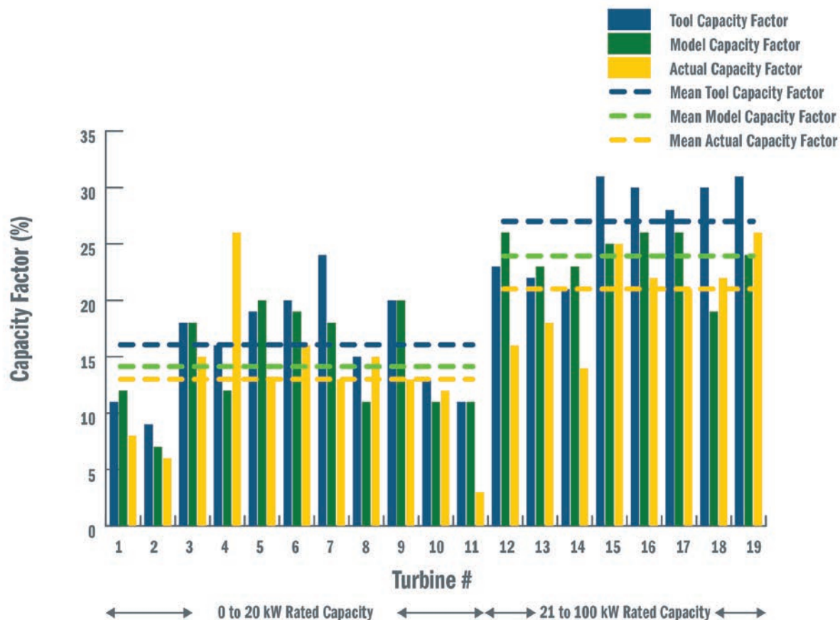
Figure 16. Actual and estimated performance for NYSEDA small wind projects
