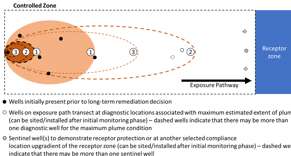
Figure 4.2. Conceptual well network for extended-scale monitoring of a diminishing source and plume scenario. In this scenario, the plume may expand and then decline (e.g., as shown by progression from numbers 1 to 3 for the source and the plume) in response to source flux changes and any previous remediation conditions.
