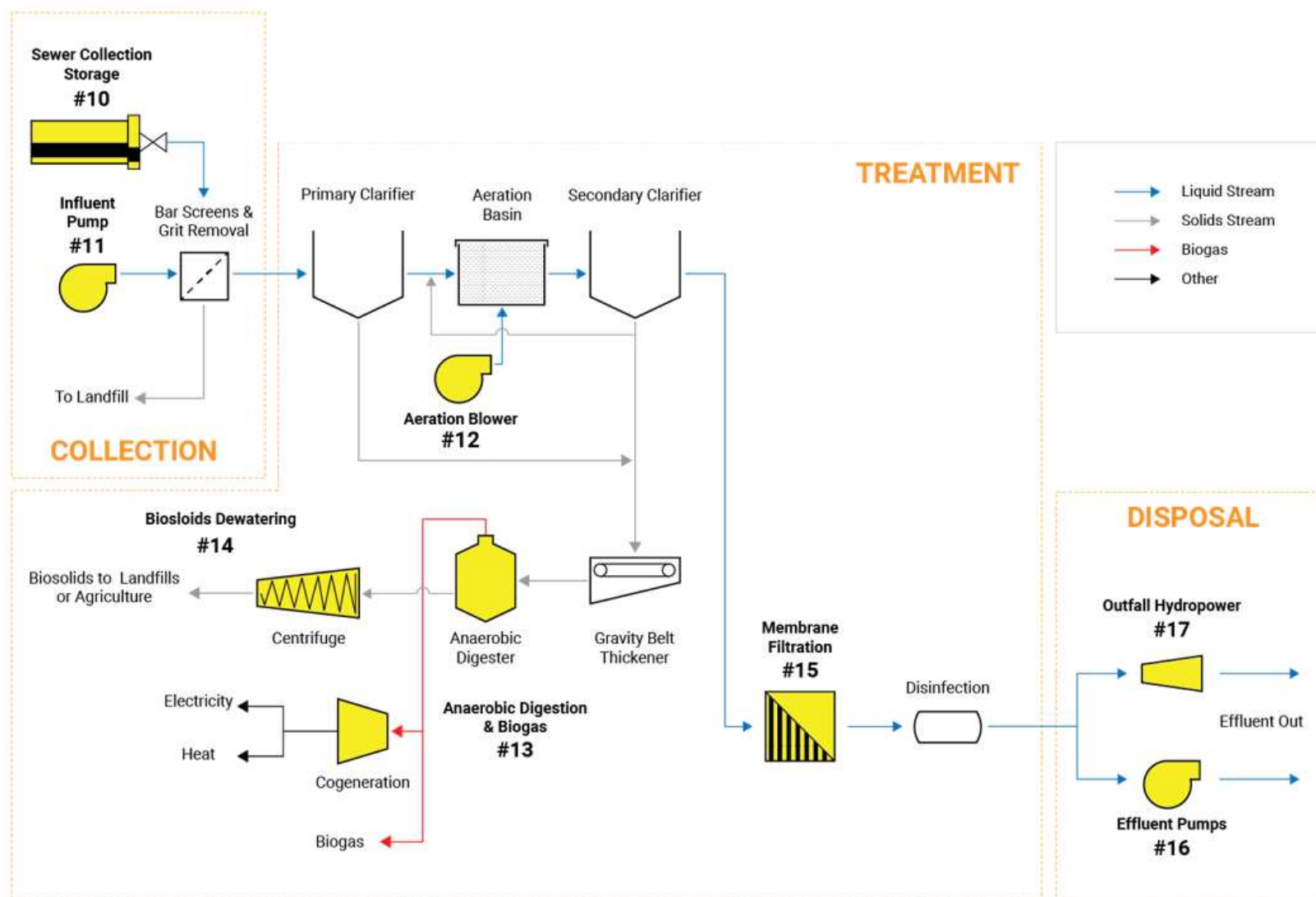
Figure 2. Wastewater System Unit Processes Yellow highlighted items have the potential to provide energy services. Adapted from Sparn and Hunsberger (2015).
