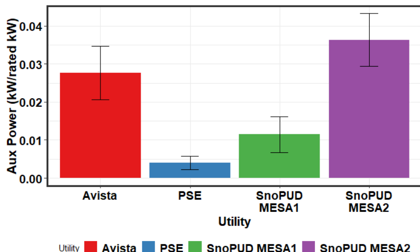
Figure 10.3. Average Auxiliary Consumption for All Utilities
