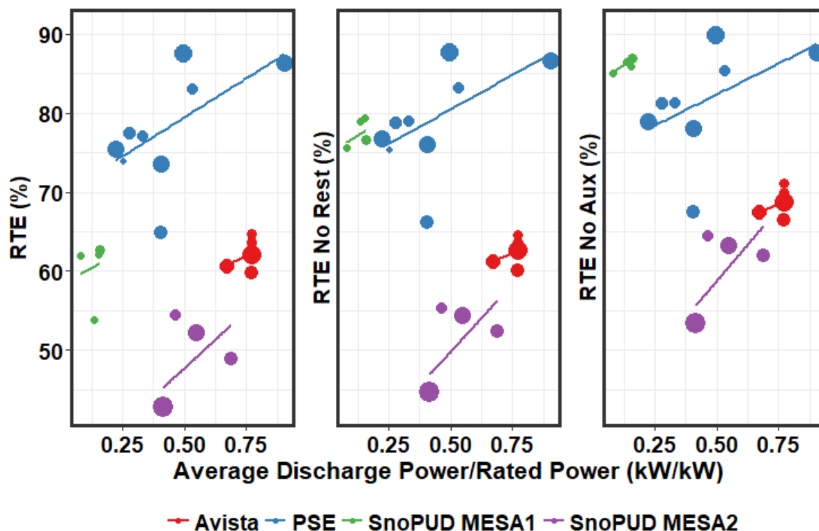
Figure 5.2. Capacity Use Case Round Trip Efficiencies
