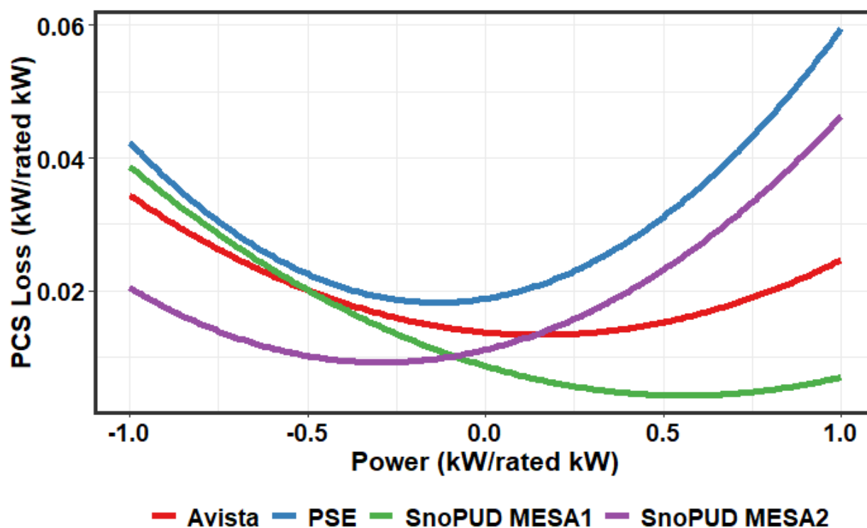
Figure 7.1. PCS Losses Regression
