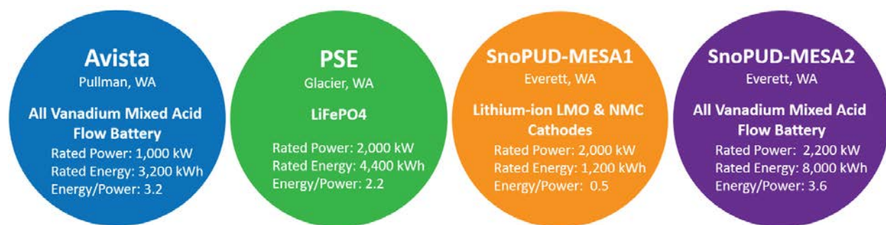
Figure ES.1. Washington CEF Battery System Characteristics
