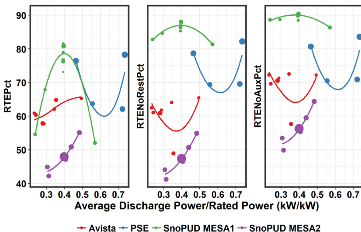
Figure 5.1. Arbitrage Use Case Round Trip Efficiencies
