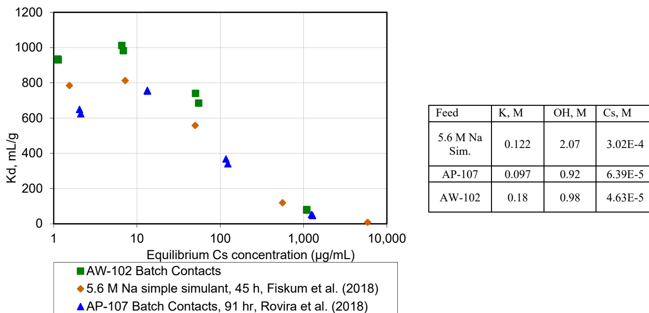
Figure 4.6. Comparison of AW-102 Test Data with 5.6 M Na Simple Simulant (Fiskum et al. 2018) and Rovira et al. (2018) Test Data
