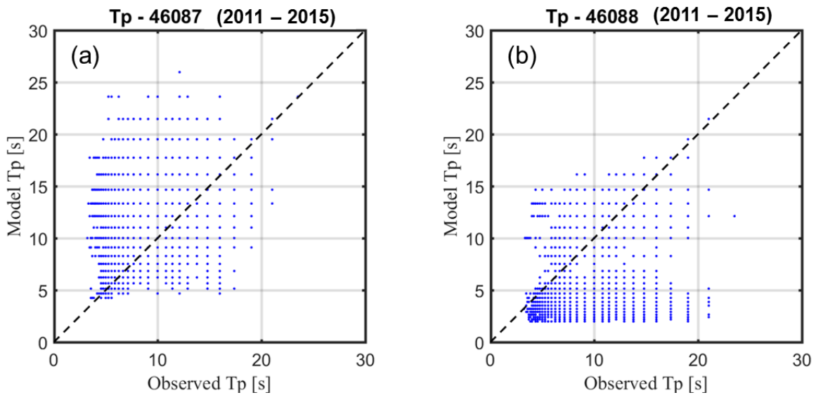
Figure 10. Scatter plots of modeled and observed wave peak period at hourly intervals at Buoy 46087 (a) and 46088 (b) for the period of 2011–2015.
