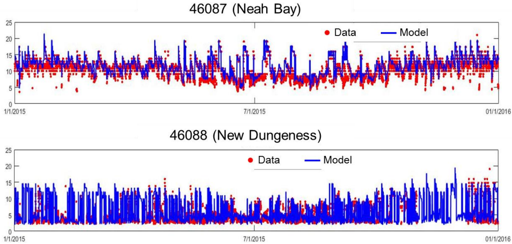
Figure 9. Comparison of simulated and measured peak period at Buoy 46087 and 46088 for 2015.
