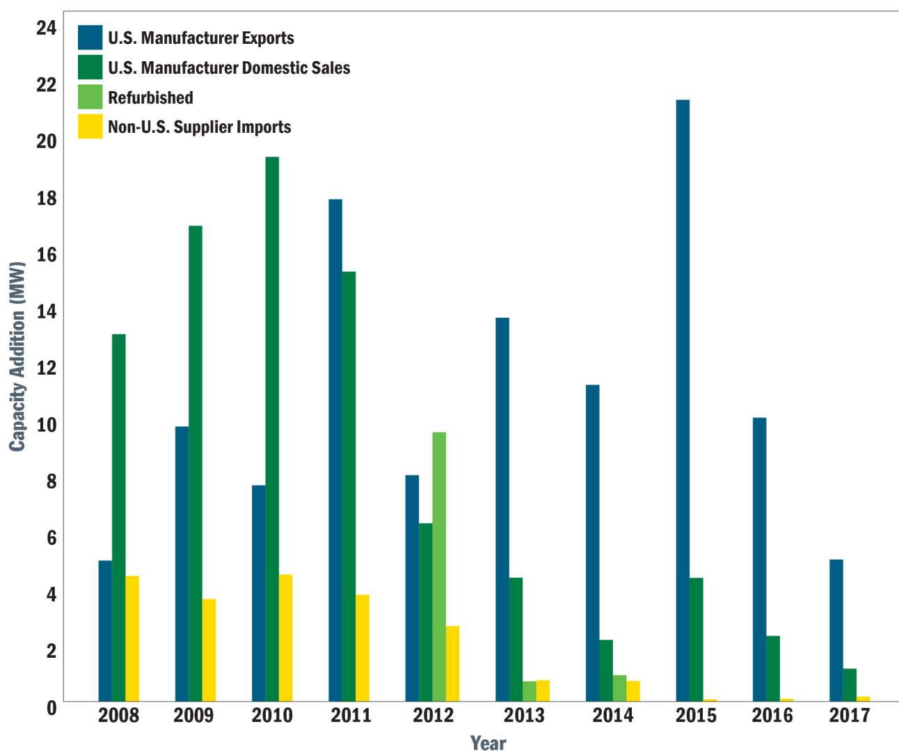
Figure 6. U.S. small wind turbine sales and exports, 2008–2017
