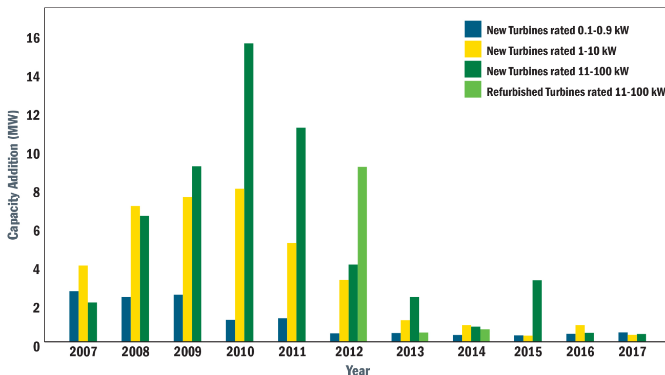
Figure 17. U.S. small wind sales capacity by turbine size
