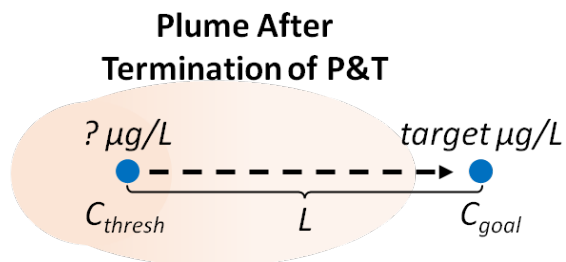
Figure 8. Depiction of the components for calculating a threshold concentration ( C_{thresh} ) based on the attenuation rate calculated from the flow-path analysis, the distance spanned ( L ), and the concentration goal at the downgradient well ( C_{goal} ). The contaminant plume with a concentration of C_{thresh} at the upgradient well will decrease in concentration to C_{goal} at the downgradient well as it passes through the attenuation zone between the wells.
