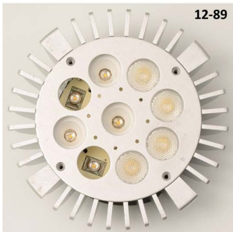
Figure 1. An example of an LED PAR38 lamp using individual secondary lenses.
