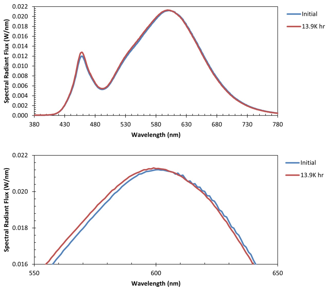
Figure 14. Spectral radiant flux plots for one sample of model 12-99. The spectrum was recorded when the lamp was first energized, and again after 13,925 hours of operation. The graph on the top shows the entire visible-spectrum response, whereas the graph on the bottom focuses on the region between 550 nm and 650 nm where phosphor emission is at its highest levels.
