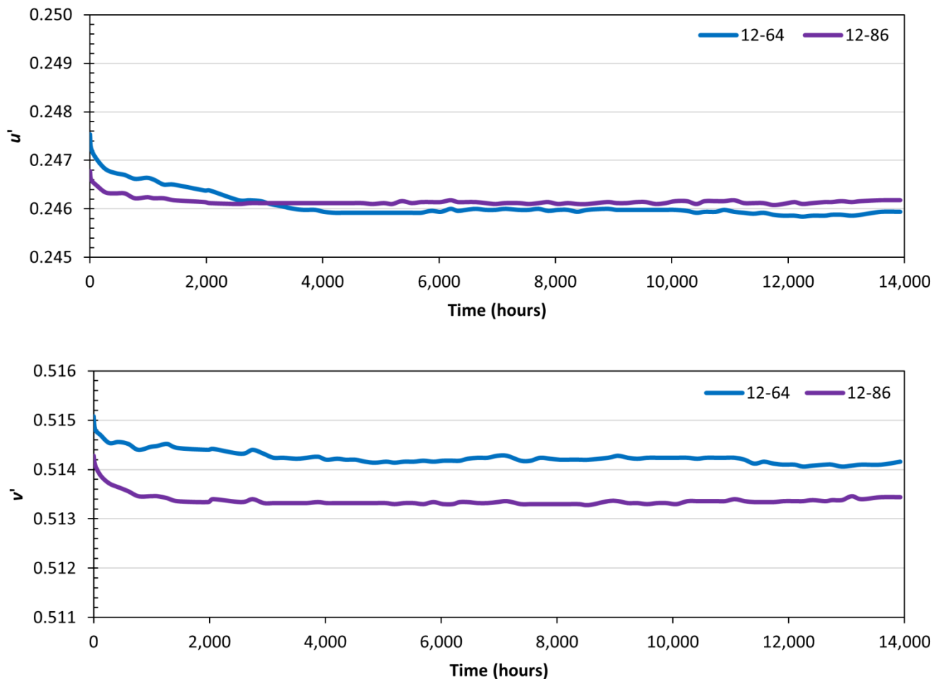
Figure 7. Time-based change in average u' and v' values for lamp models 12-64 and 12-86 during testing at an ambient temperature of 45°C in ALTA2. Both of these LED models exhibited a blue chromaticity shift during the test period. The reported values are the averages for the five samples tested for each lamp model.
