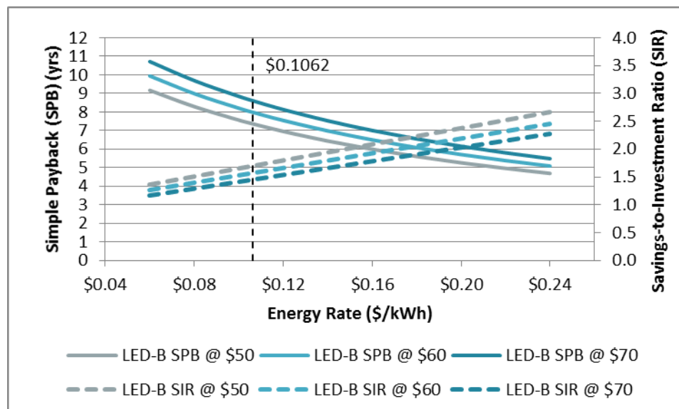
Figure 50. LED-B Simple Payback and Savings-to-Investment-Ratio with 100% of RS Means Labor Assumption
