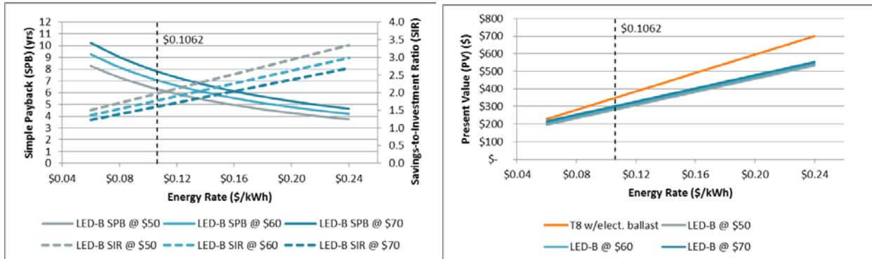
Figure 3. LED-B Simple Payback, Savings-to-Investment-Ratio, and Present Value Results with 50% RS Means Labor Assumption
