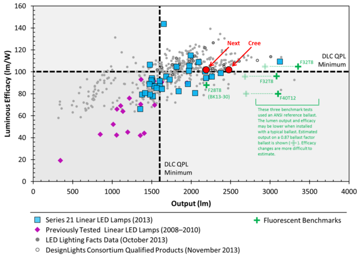
Figure 5. Existing Market Luminous Efficacy vs. Light Output
