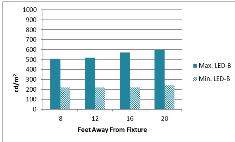
Figure 43. Auburn Design and Construction Luminous Intensity – Short Axis (LED-B)
