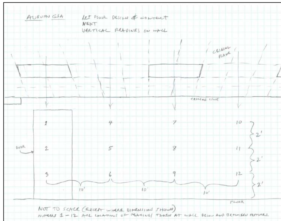
Figure 19. Sketch of Auburn Design and Construction Vertical Measurement Points (LED-B)
