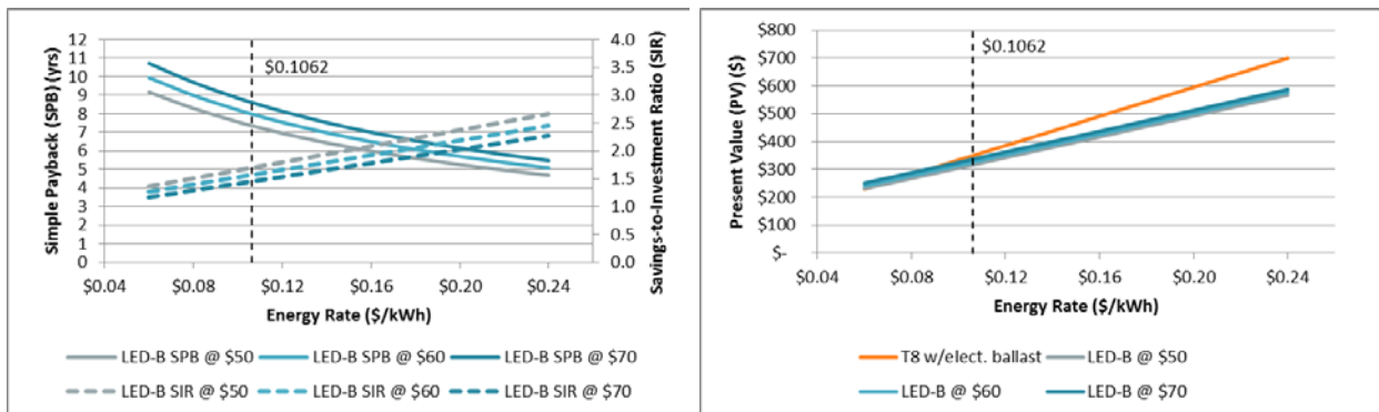
Figure 4. LED-B Simple Payback, Savings-to-Investment-Ratio, and Present Value Results with 100% RS Means Labor Assumption
