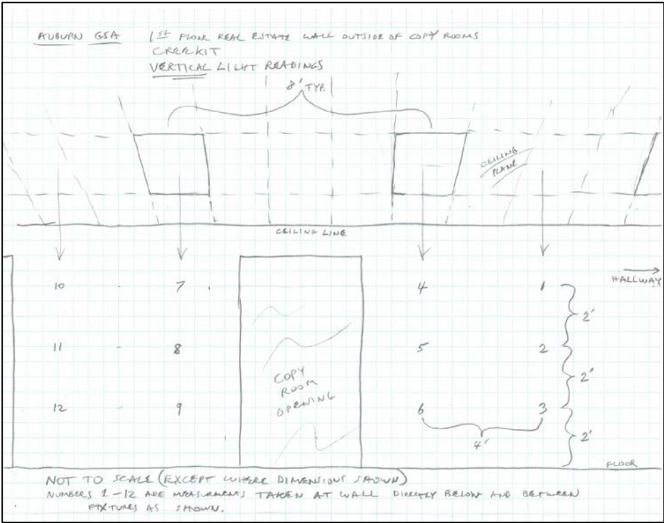
Figure 14. Sketch of Auburn Real Estate Vertical Measurement Points (LED-A)
