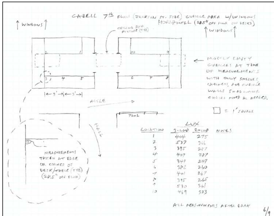
Figure 22. Sketch of Dallas Property Management Horizontal Measurement Points (LED-A)
