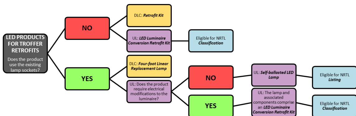
Figure 60. Luminaire Retrofit Classifications
