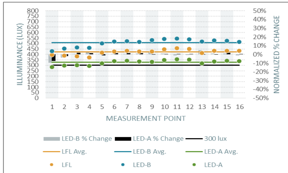
Figure 39. Philadelphia Daycare Playrooms 405 and 413 Combined Horizontal Illuminance and Normalized Percent Change (LED-A and LED-B)
