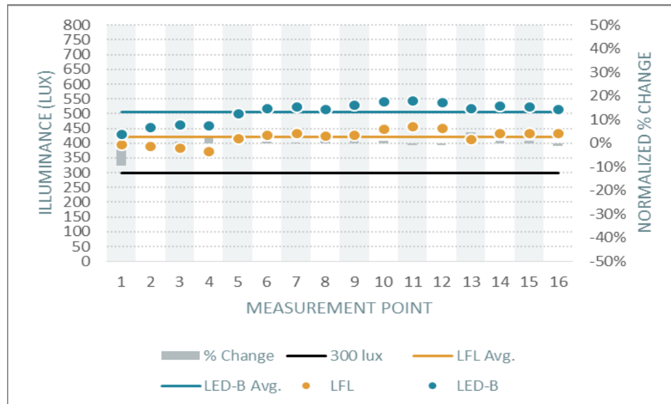
Figure 38. Philadelphia Daycare Playroom 413 Horizontal Illuminance and Normalized Percent Change (LED-B)
