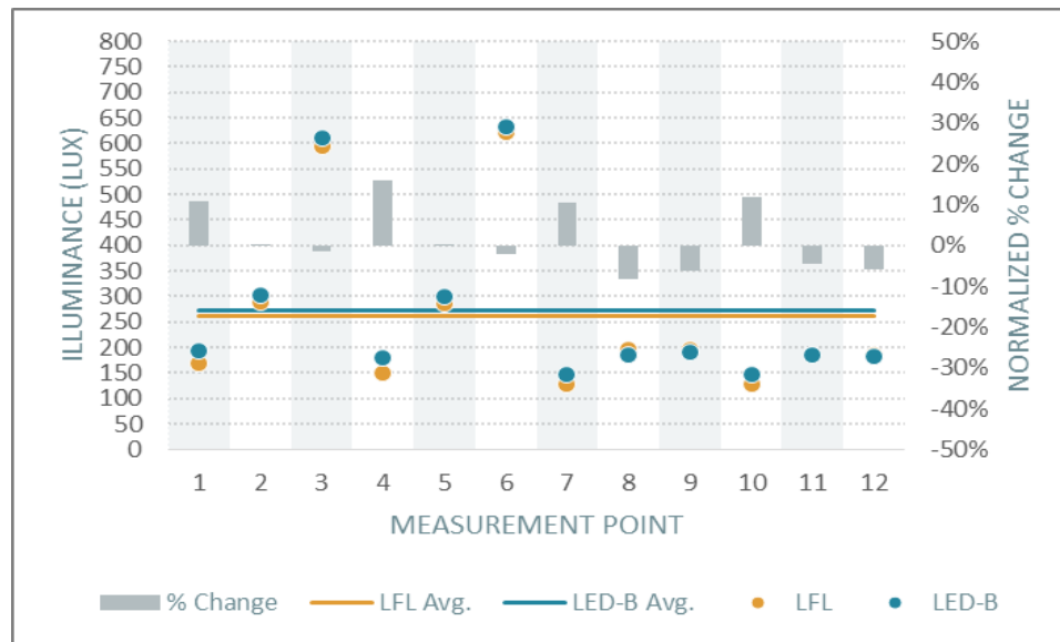
Figure 30. Dallas Project Management Vertical Illuminance and Normalized Percent Change (LED-B)
