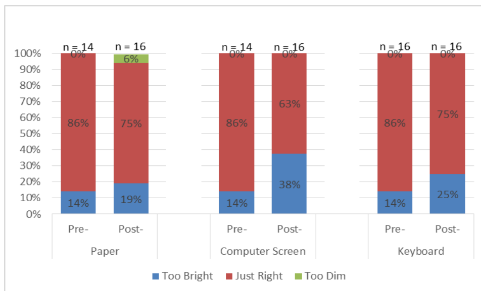
Figure 55. Auburn Real Estate (LED-A) Task Light Level Survey
