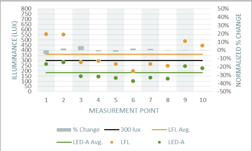
Figure 23. Dallas Property Management Horizontal Illuminance and Normalized Percent Change (LED-A)
