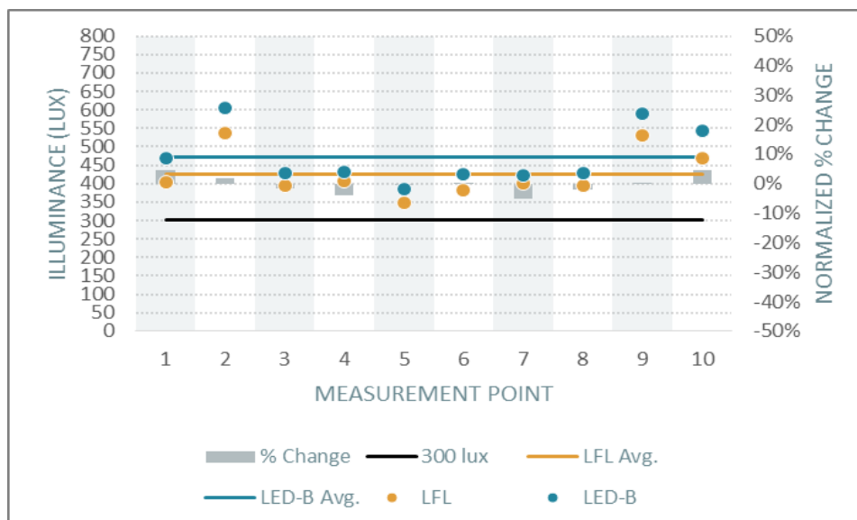
Figure 28. Dallas Project Management Horizontal Illuminance and Normalized Percent Change (LED-B)
