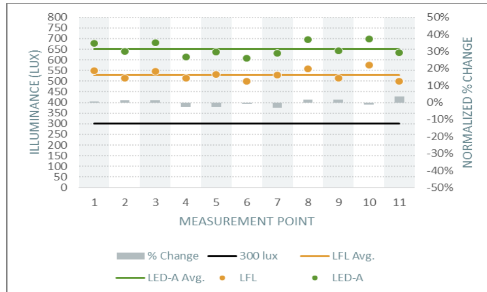
Figure 13. Auburn Real Estate (LED-A). Horizontal Illuminance and Normalized Percent Change
