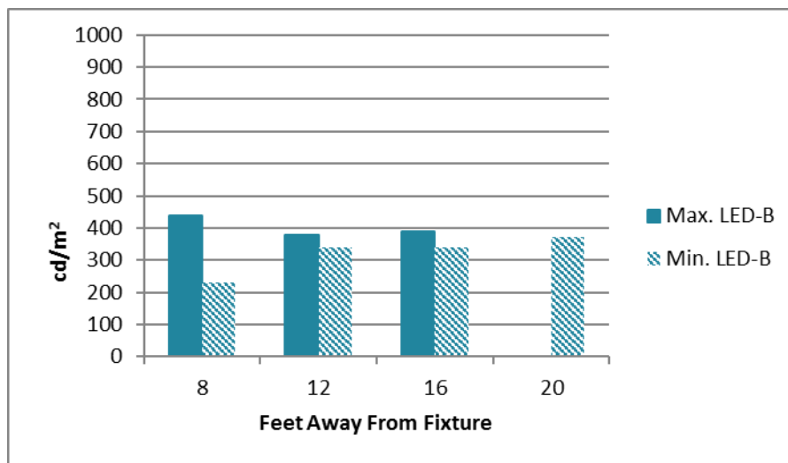
Figure 43. Auburn Design and Construction Luminous Intensity – Short Axis (LED-B)
