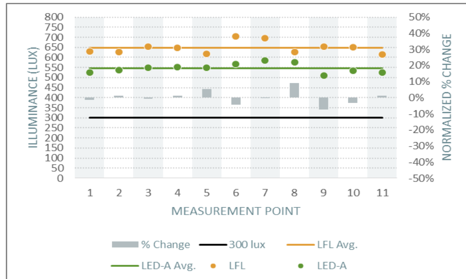
Figure 33. Philadelphia Daycare Classroom 460 Horizontal Illuminance and Normalized Percent Change (LED-A)
