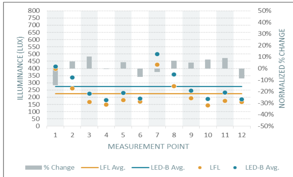
Figure 20. Auburn Design and Construction (LED-B) – Vertical Illuminance and Normalized Percent Change
