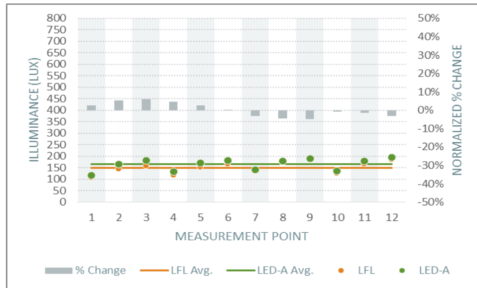
Figure 15. Auburn Real Estate (LED-A). Vertical Illuminance and Normalized Percent Change
