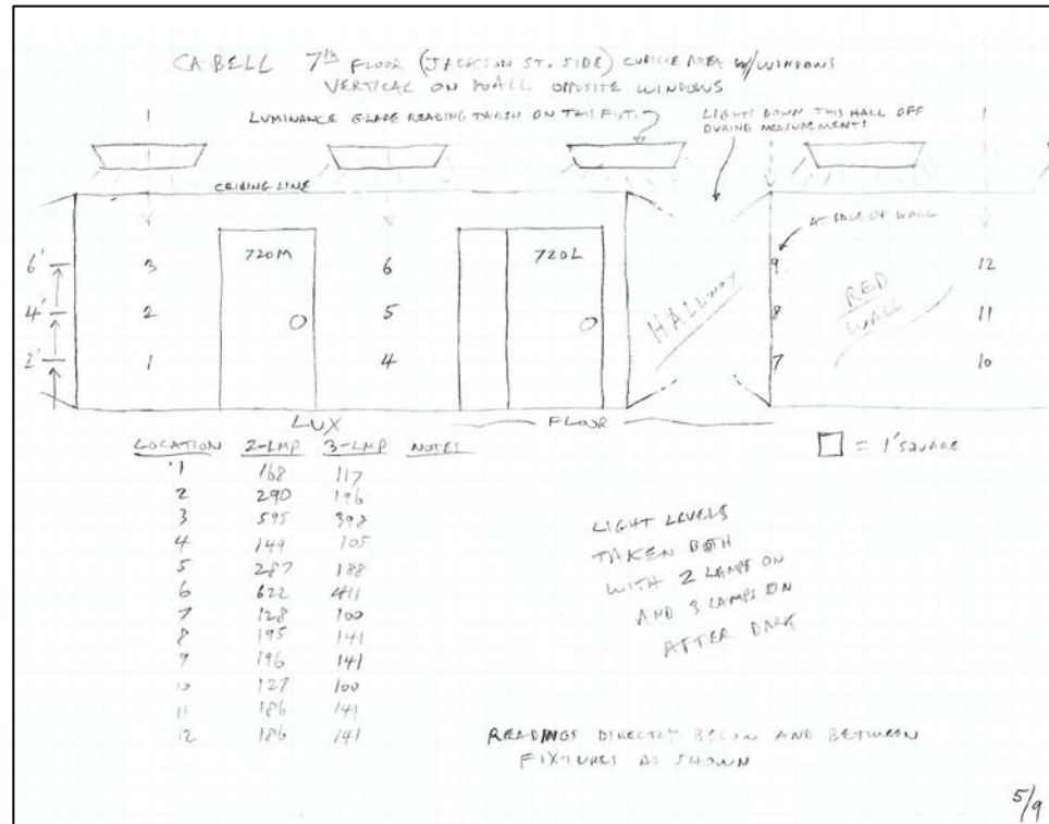
Figure 24. Sketch of Dallas Property Management Vertical Measurement Points (LED-A)
