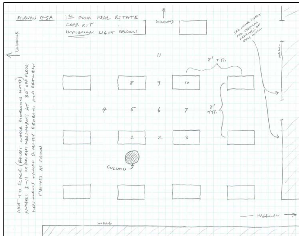
Figure 12. Sketch of Auburn Real Estate Horizontal Measurement Points (LED-A)
