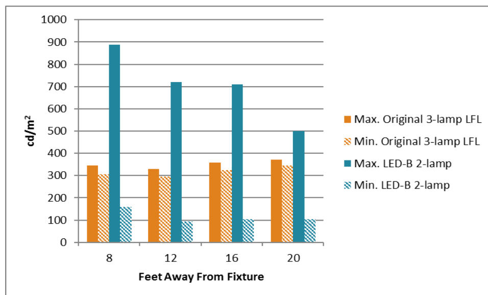
Figure 41. Dallas Project Management Luminous Intensity – Short Axis (LED-B)
