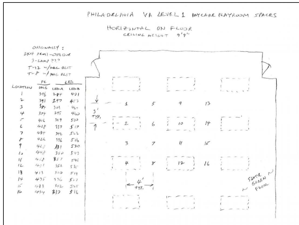
Figure 35. Sketch of Philadelphia Daycare Playroom 405 Horizontal Measurement Points (LED-A)
