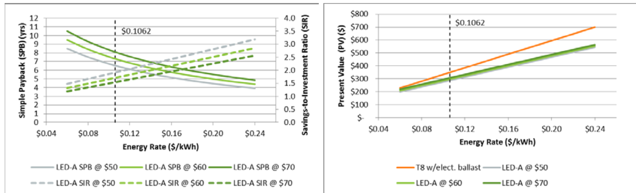
Figure 1. LED-A Simple Payback, Savings-to-Investment-Ratio, and Present Value Results with 50% RS Means Labor Assumption
