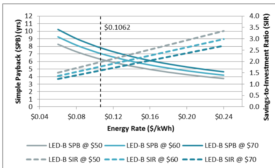
Figure 49. LED-B Simple Payback and Savings-to-Investment-Ratio with 50% of RS Means Labor Assumption
