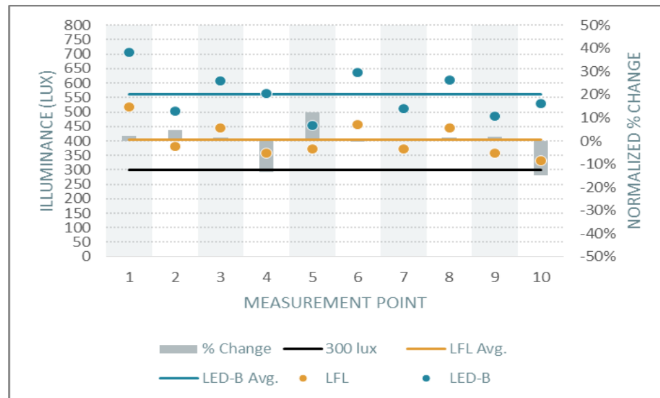
Figure 18. Auburn Design and Construction (LED-B). Horizontal Illuminance and Normalized Percent Change
