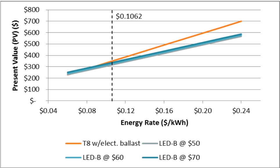
Figure 54. LED-B Present Value Results with 100% RS of Means Labor Assumption
