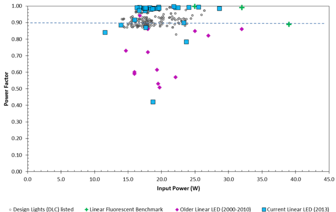
Figure 46. Linear LED and Fluorescent Lighting Product Power Factors
