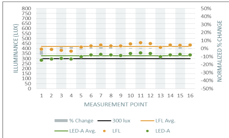
Figure 36. Philadelphia Daycare Playroom 405 Horizontal Illuminance and Normalized Percent Change (LED-A)
