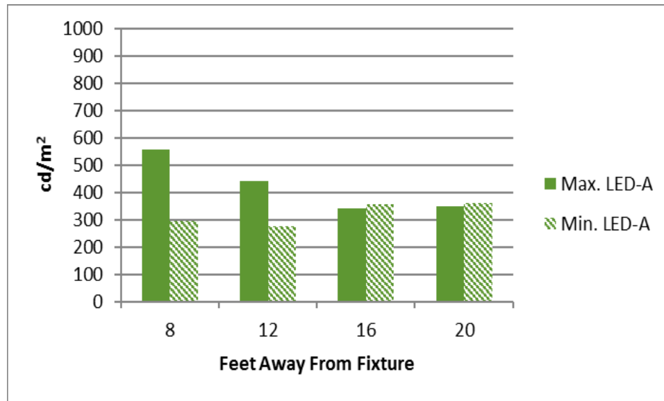
Figure 45. Auburn Real Estate Luminous Intensity – Short Axis (LED-A)
