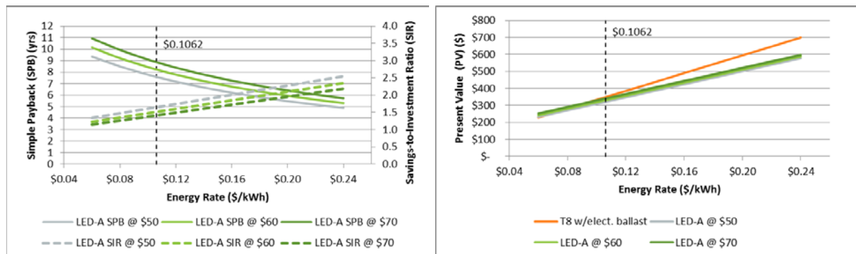
Figure 2. LED-A Simple Payback, Savings-to-Investment-Ratio, and Present Value Results with 100% RS Means Labor Assumption
