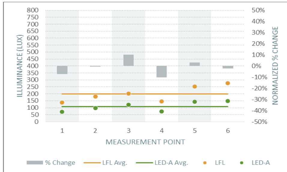
Figure 25. Dallas Property Management Vertical Illuminance and Normalized Percent Change (LED-A)
