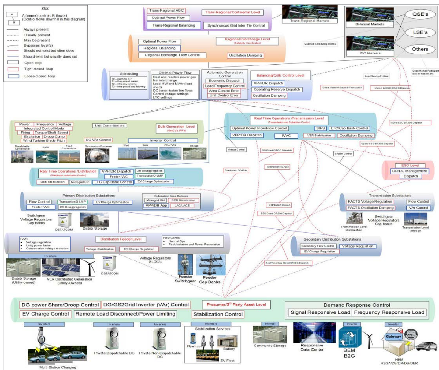
Figure 2. Grid Macro Control Reference Model
