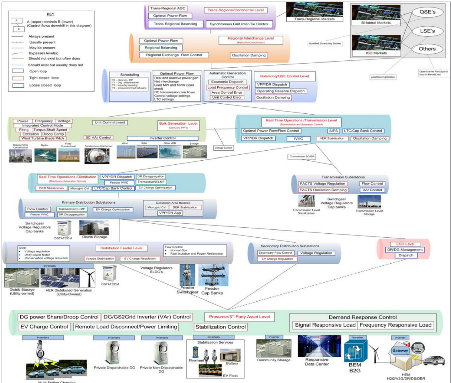
Figure 4. Regularized Grid Control Macro Structure
