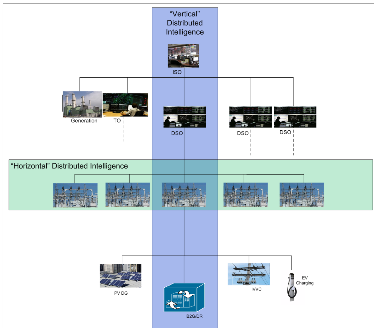
Figure 5. Vertical and Horizontal Distributed Intelligence
