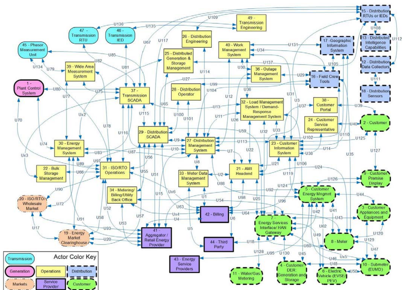
Figure 1. NIST/NISTR Grid Elements Diagram
