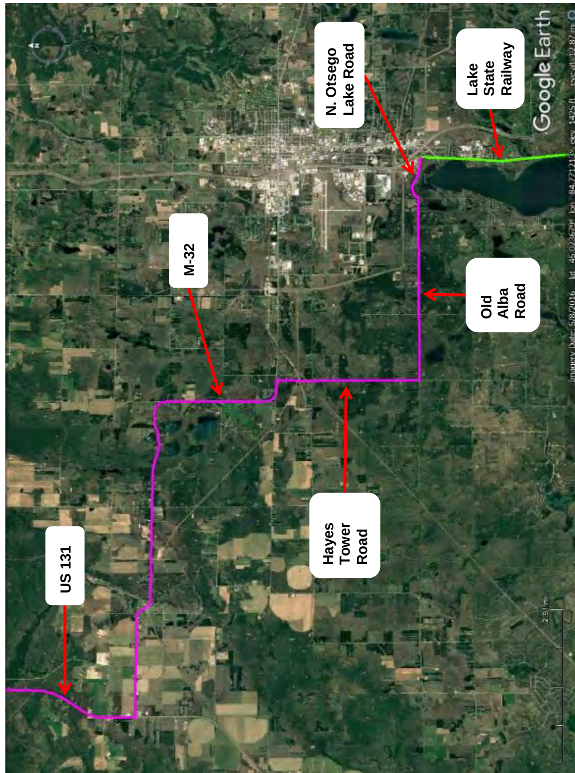
Figure 2-77. Route Taken By Reactor Pressure Vessel in the Vicinity of Gaylord, Michigan (Google 2017)
