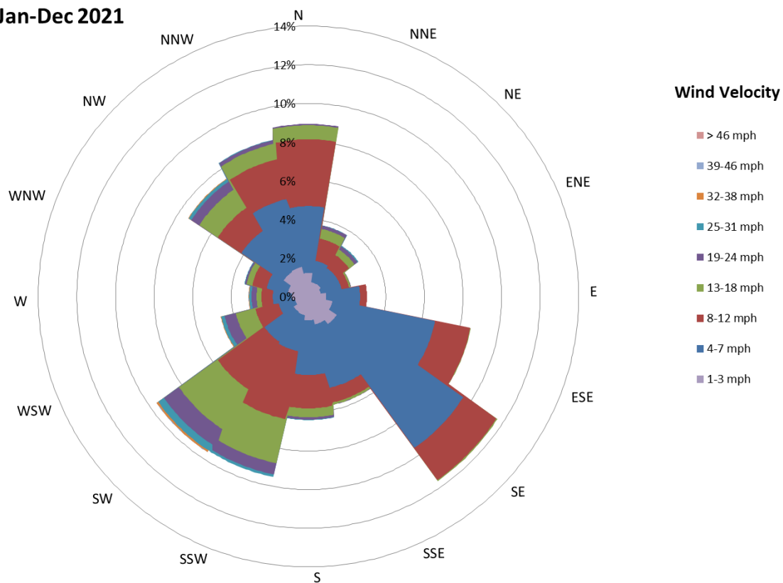
Figure A.1. Hanford Site 300 Area Meteorological Station Wind Rose and Histogram for 2021
