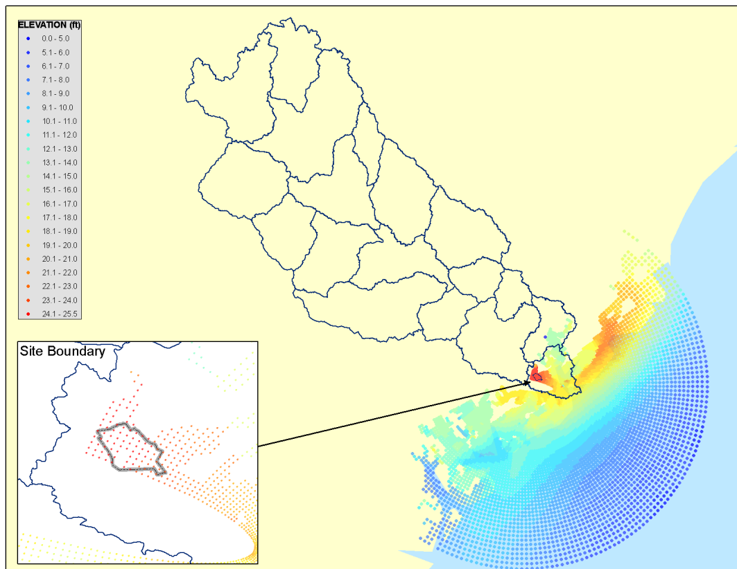
Figure E-1. The PMH MOM Water-Surface Elevations for the Study Watershed
