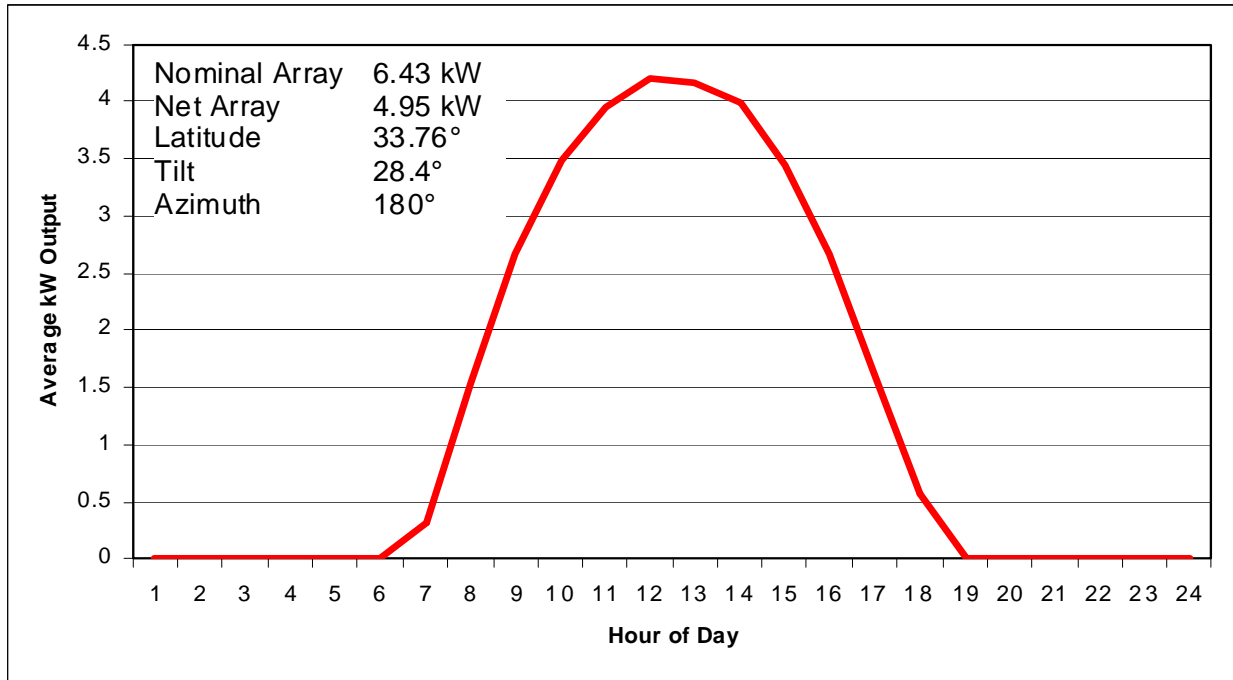
Figure 4. Fresno July Average Day—Net-Zero PV Array Output
