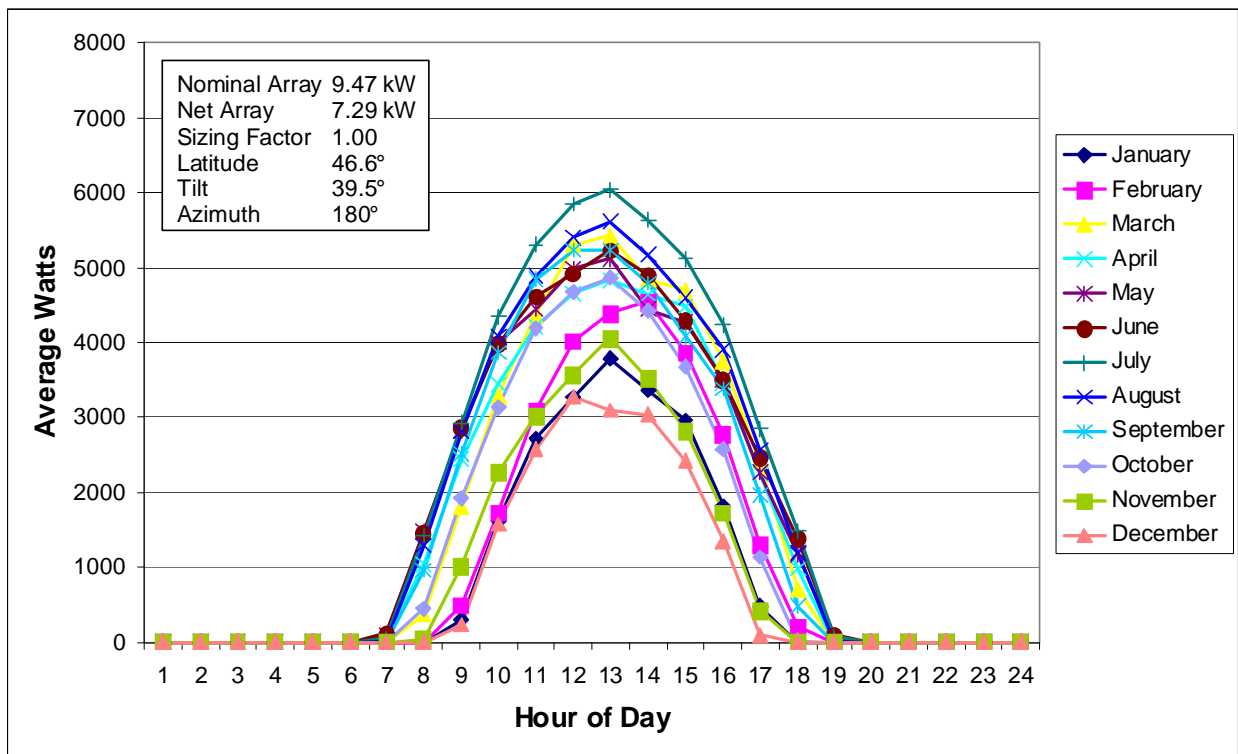
Figure 14. Helena Minimize Array Size
