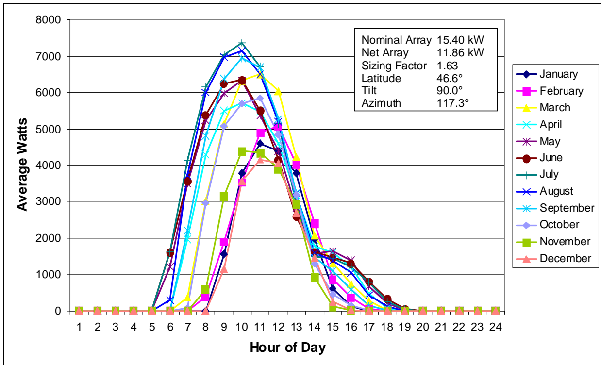
Figure 16. Helena Maximize Output at Hour of NWP Sub-Region Peak Demand (January 29 th at 7:30)
