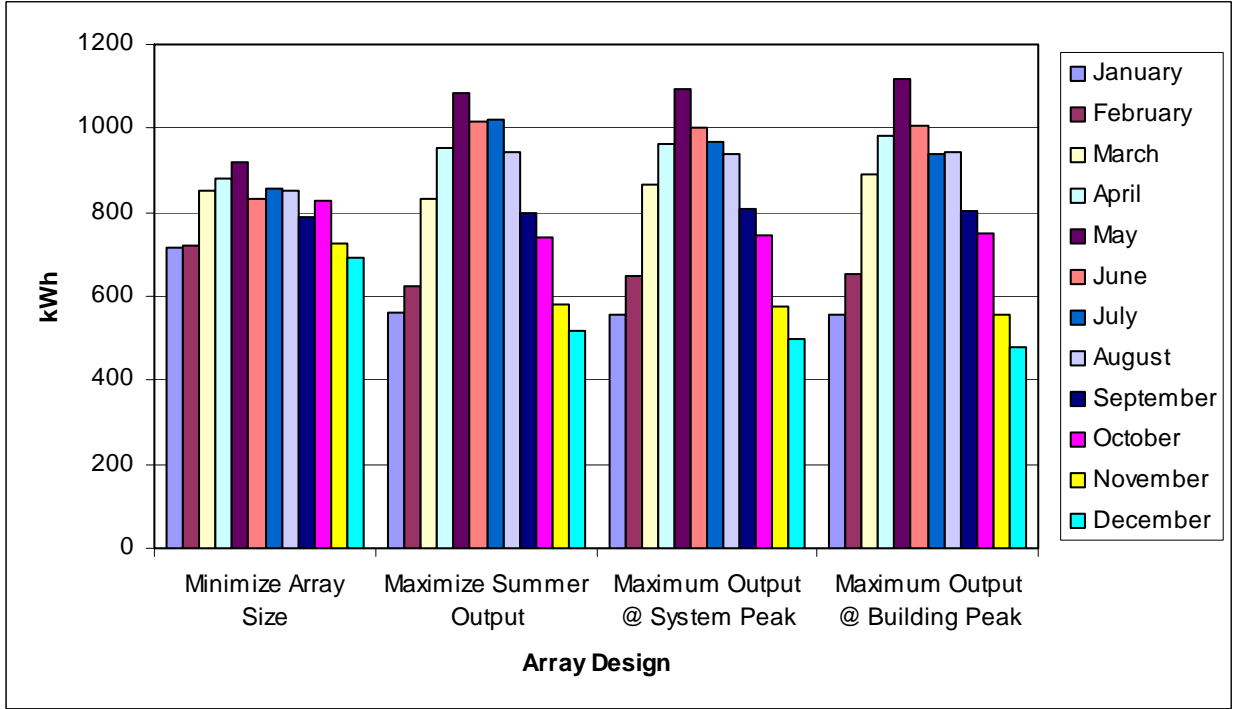
Figure 13. Albuquerque Monthly Generation—Net-Zero Arrays
