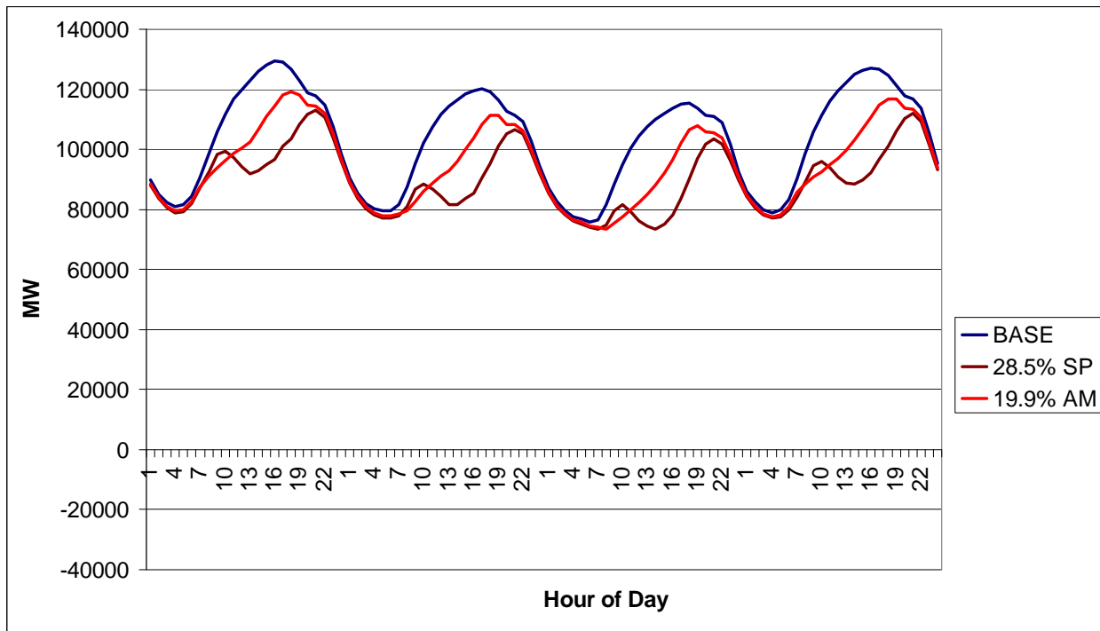
Figure 22. WECC Power Demand June 29 to July 2: Reduced ZEH Penetration
