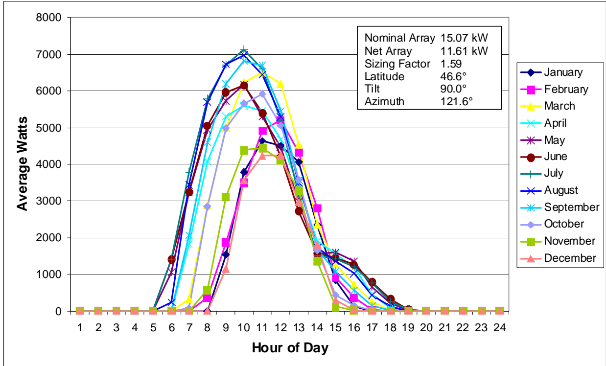
Figure 17. Helena Maximize Output at Hour of Building Peak Demand (January 16 th at 7:30)
