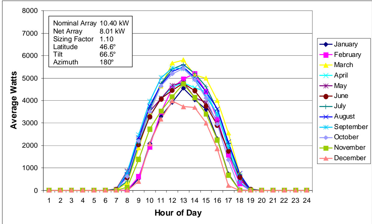
Figure 15. Helena Maximize January Generation
