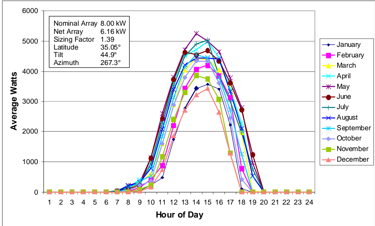
Figure 9. Albuquerque Maximize Output at Hour of System Peak Demand (July 10 th at 15:30)
