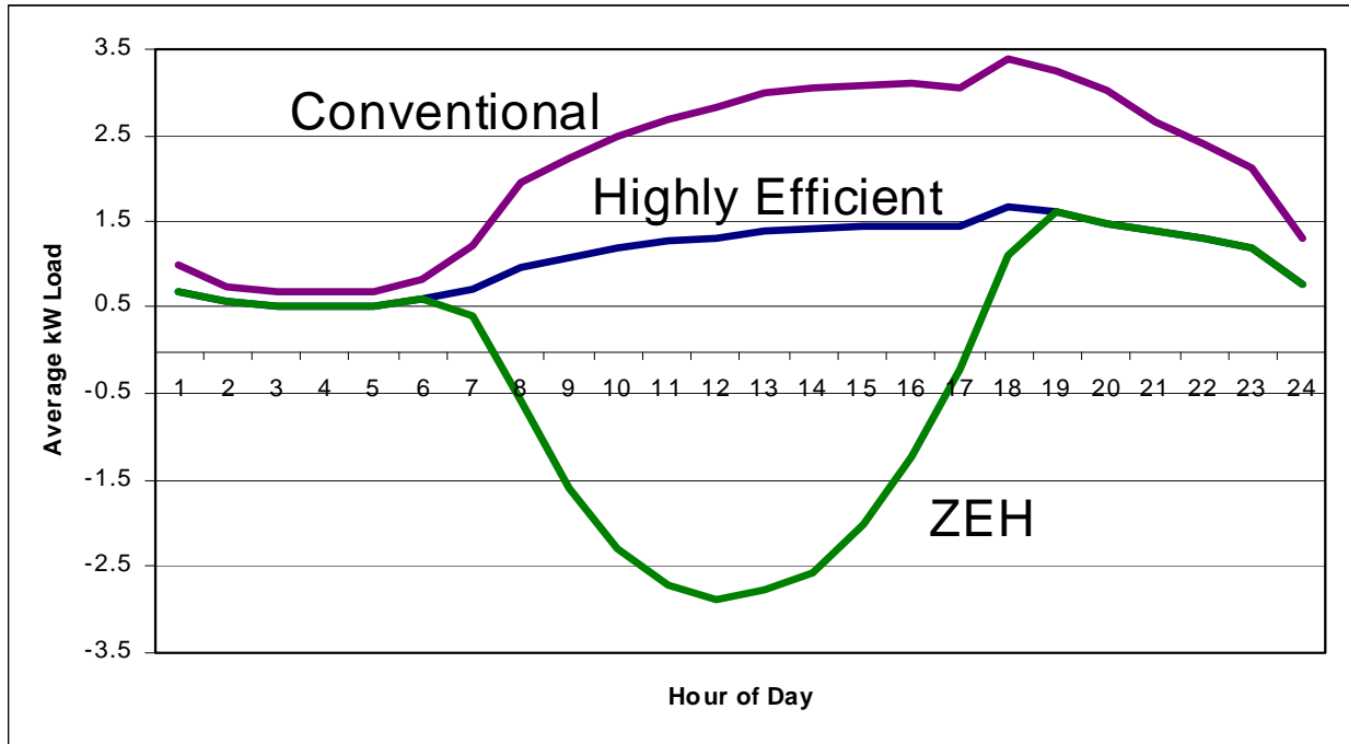
Figure 5. Fresno July Average Day—Net Load
