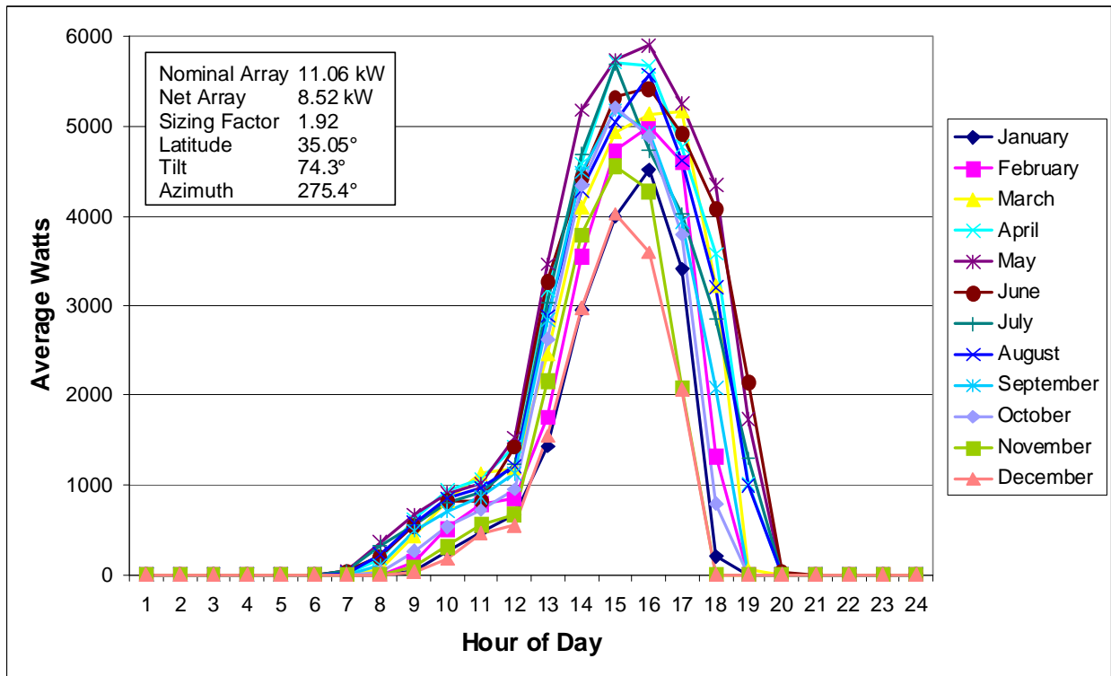
Figure 10. Albuquerque Maximize Output at Hour of Building Peak Demand (August 16 th at 17:30)
