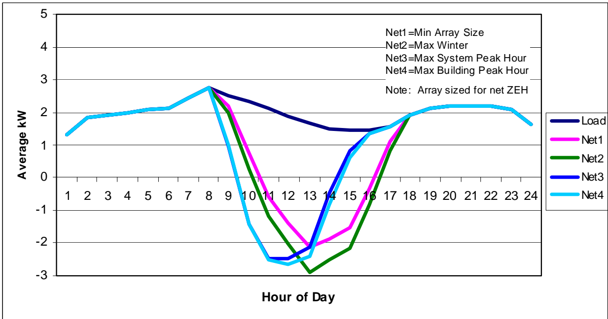
Figure 19. Helena January Average Hourly Net Load for Array Design Options
