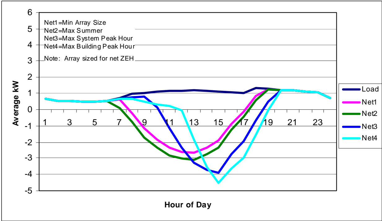
Figure 12. Albuquerque July Average Hourly ZEH Net Load for Array Design Options
