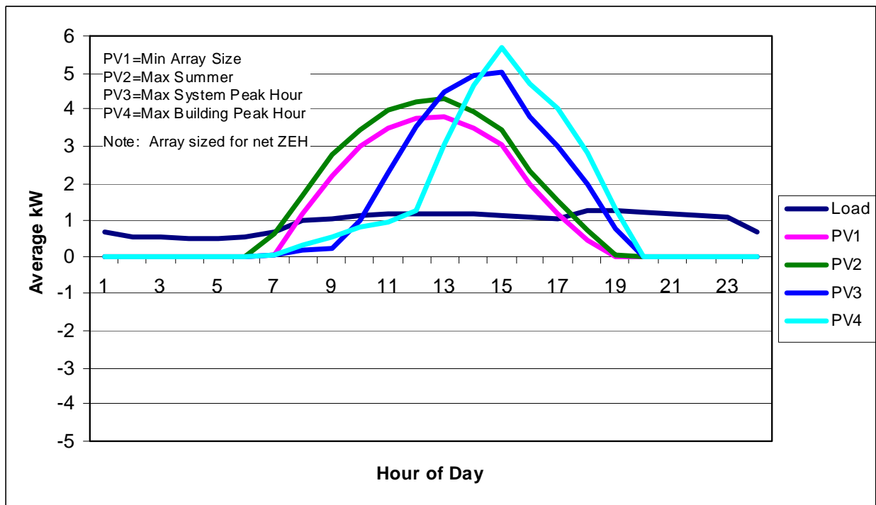
Figure 11. Albuquerque July Average Hourly Output for Array Design Options
