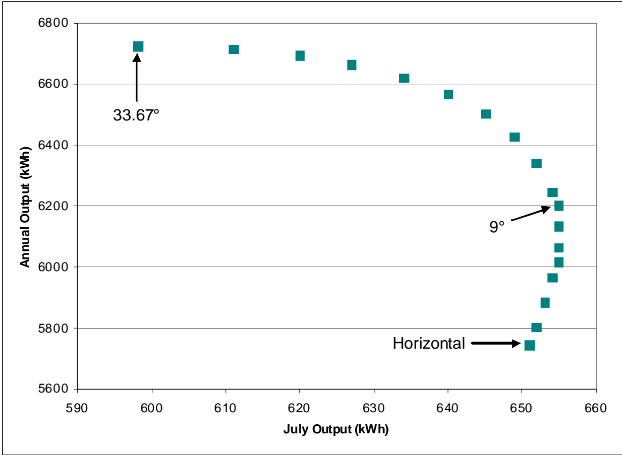
Figure 6. Albuquerque PV Array Output as a Function of Tilt (Latitude 35.05°)
