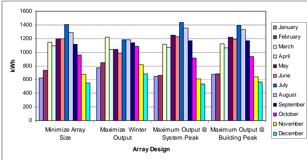
Figure 20. Helena Monthly Generation—Net-Zero Arrays
