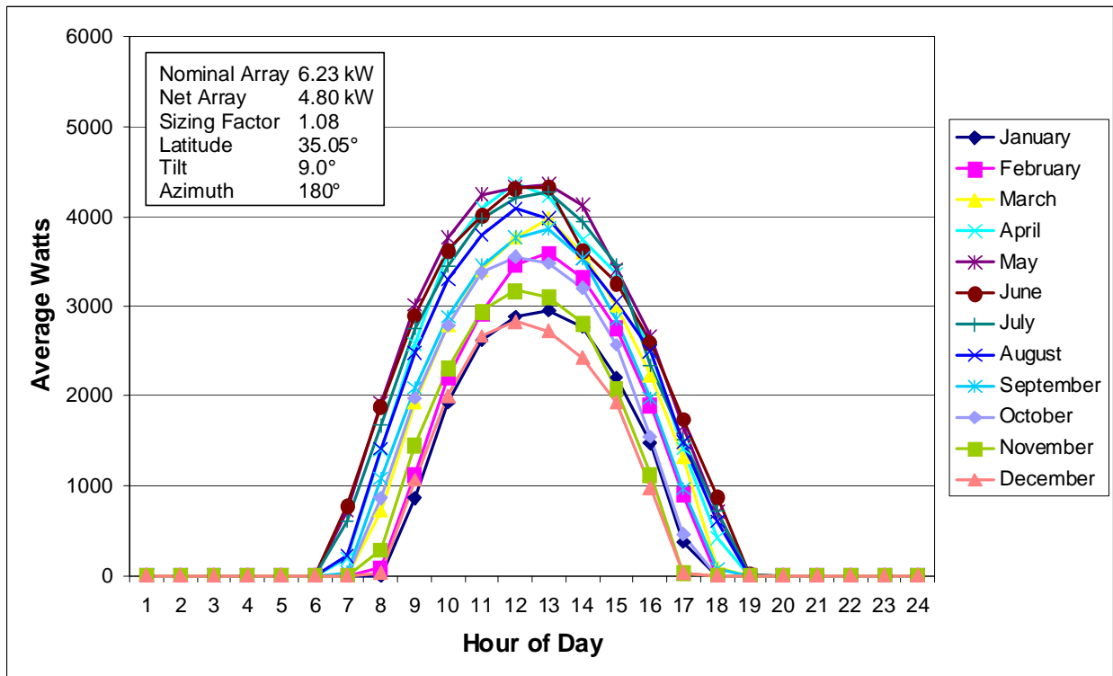
Figure 8. Albuquerque Maximize July Generation
