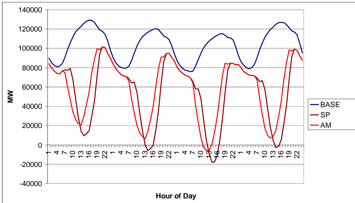
Figure 21. WECC Power Demand June 29 to July 2: 100% ZEH Penetration
