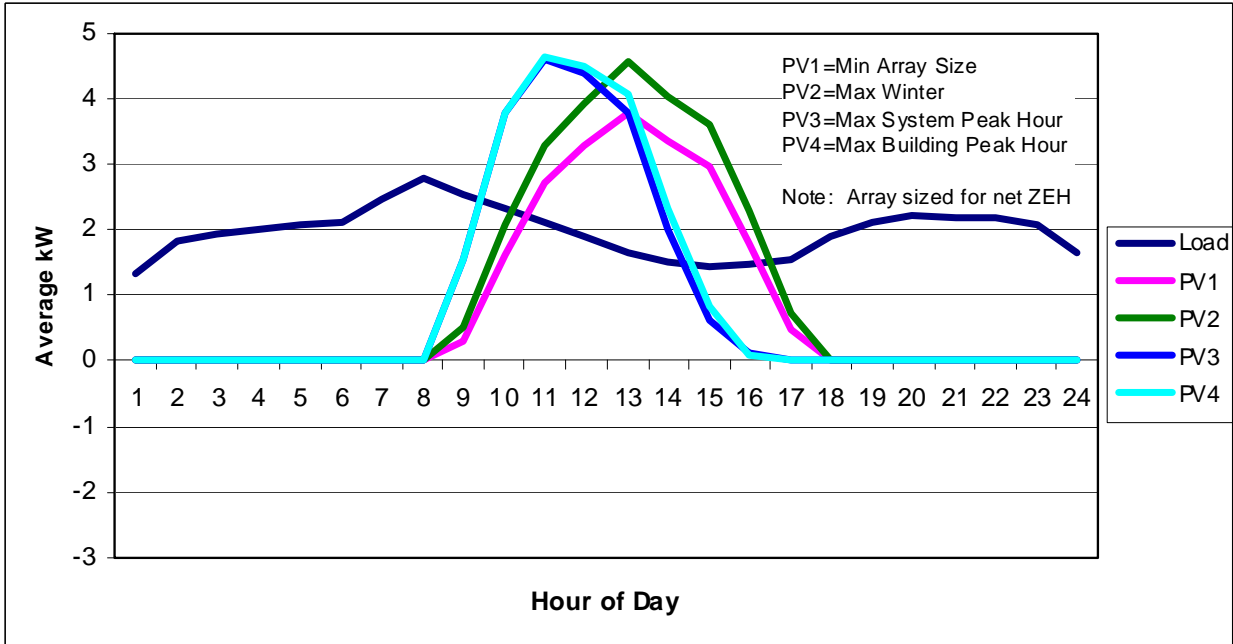
Figure 18. Helena January Average Hourly Output for Array Design Options
