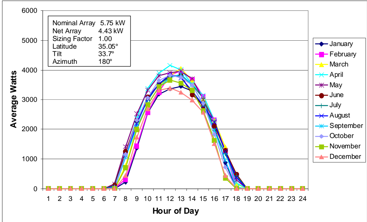
Figure 7. Albuquerque Minimize Array Size
