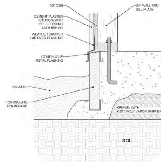
Davis Energy Group of the CARB Building America team developed a new method for insulating slab perimeters that is ideal for extremely hot climates and mixed dry climates. The method, which is still being tested, uses termiticide-treated rigid foam insulation encased in PVC as the form for the concrete foundation.
