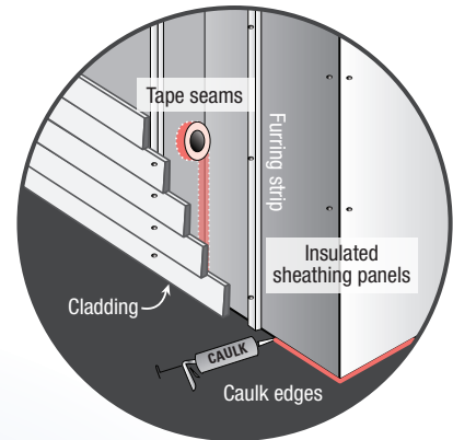
Insulating Sheathing Detail
