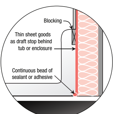
20 Tub
