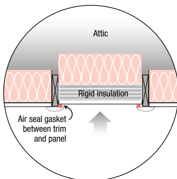
11 Attic Access
