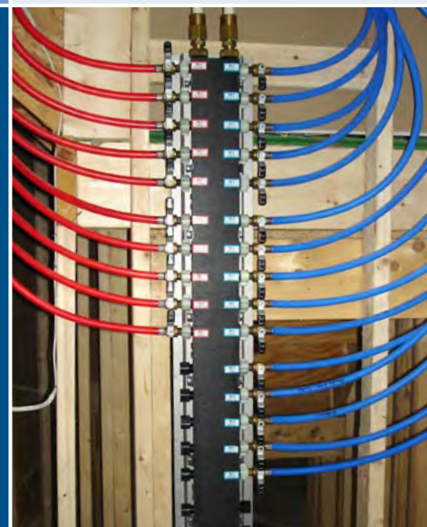
A centrally located manifold water distribution system saves energy by reducing hot water usage.
