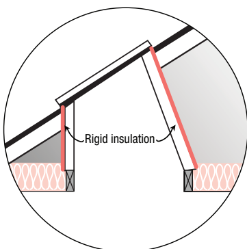
14 Skylight
