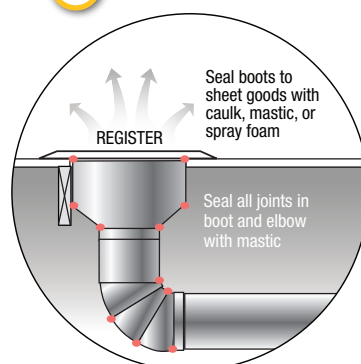
16 Registers
