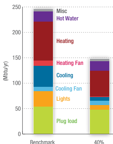
A Comparison of Energy Usage by End Use for a Home Built to Perform with 40% Energy Savings Compared to the Building America Benchmark (a home built to MEC 1993) in the Hot-Dry Climate.
