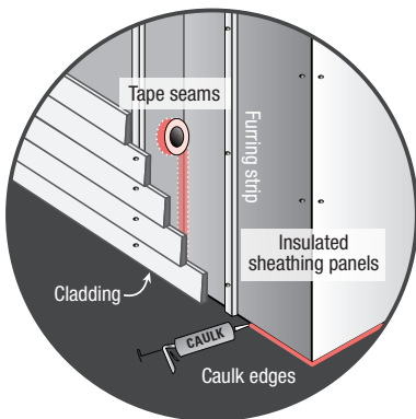
An exterior air barrier system, like rigid foam insulating sheathing, can provide a continuous air barrier when seams are taped or caulked. Furring strips attached over the foam allow the foam to act as a drainage plane and the space to serve as a ventilation gap, which is especially important under porous claddings like brick and stucco.
