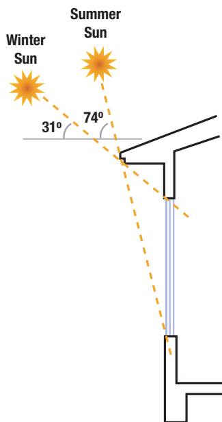
Sun angles for Albuquerque, NM. A 4-foot window would need an overhang extending 19 inches with 12 inches of wall above the window.
