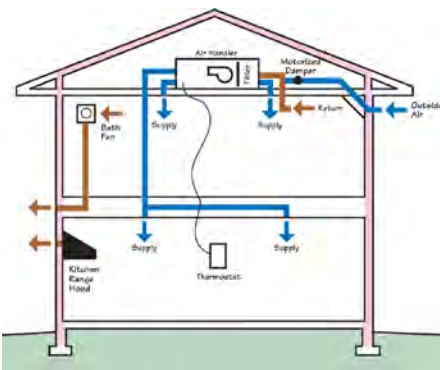
Building Science Corporation designed an HVAC system that included mechanically controlled ventilation using the furnace air handler along with point source ventilation in the kitchen and bath. (Figure source: Building Science Corporation)
