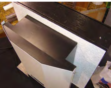
This exhaust fan and electronic controls are designed to ventilate—and could be used to create a slightly negative pressure in—the garage. Ventilation carries pollutants to the outside; negative pressure helps to stop garage air from migrating into attached houses.
