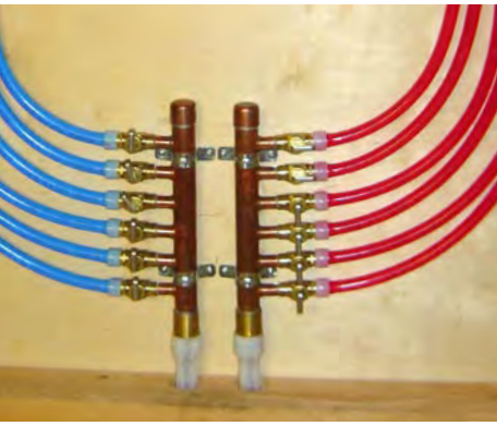
In an NAHB Research Center study, the central manifold hot water distribution system provided hot water to the fixtures more quickly than traditional trunk and branch and remote manifold distribution methods.
