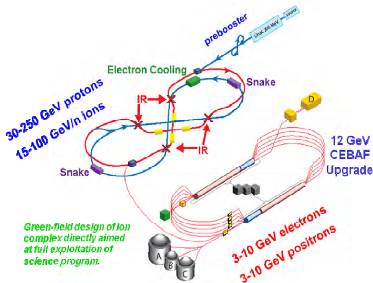
Figure 30. A schematic drawing for the Electron Light Ion Collider (ELIC) ring-ring concept. Image courtesy of Robert Ryne (Lawrence Berkeley National Laboratory).
