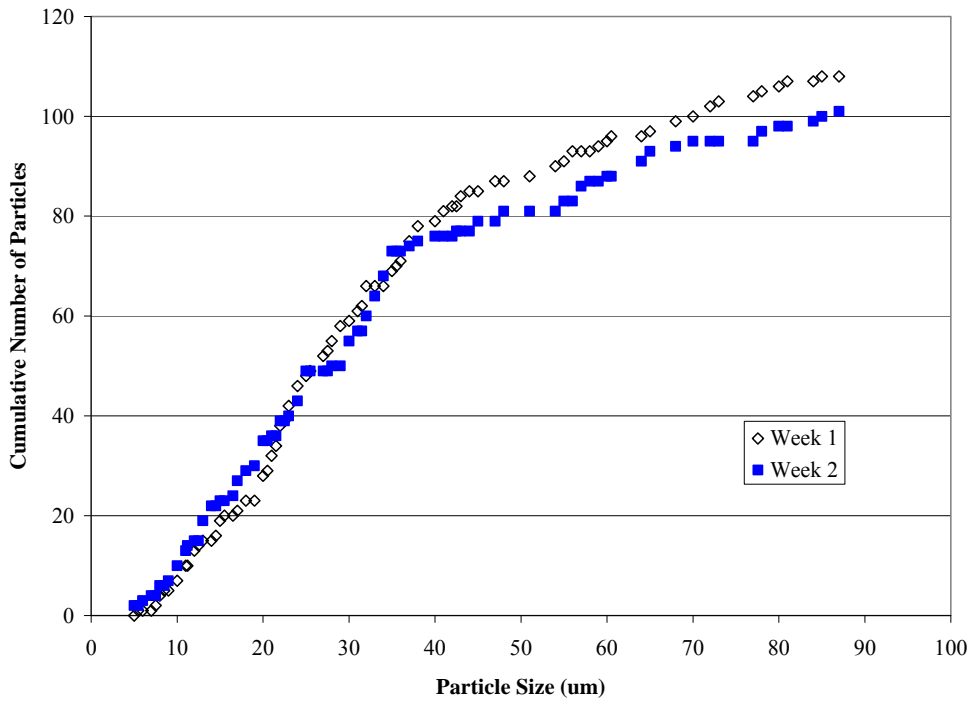
Figure 7.17. Particle Length Distribution of Sample Bottle #D_00PF1_015_XX_5476_ARC_4 (wash #40)
